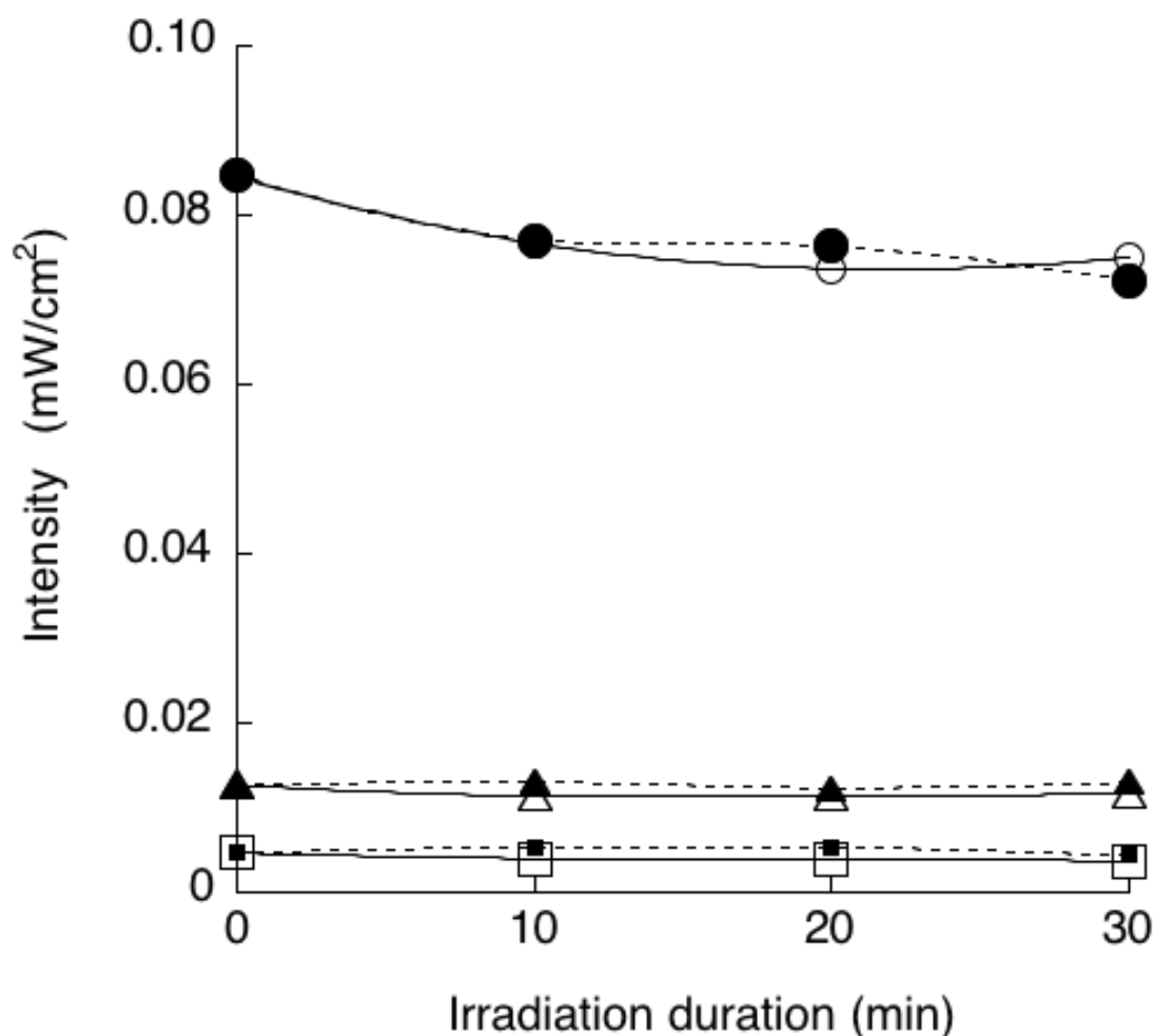
Fig. 3-2. The intensity of UVC-LED when the distance and temperature changes. 2 cm (○), 6 cm (△), and 10cm (□) at room temperature and 2 cm (●), 6 cm (▲), and 10cm (■) at -30°C.
