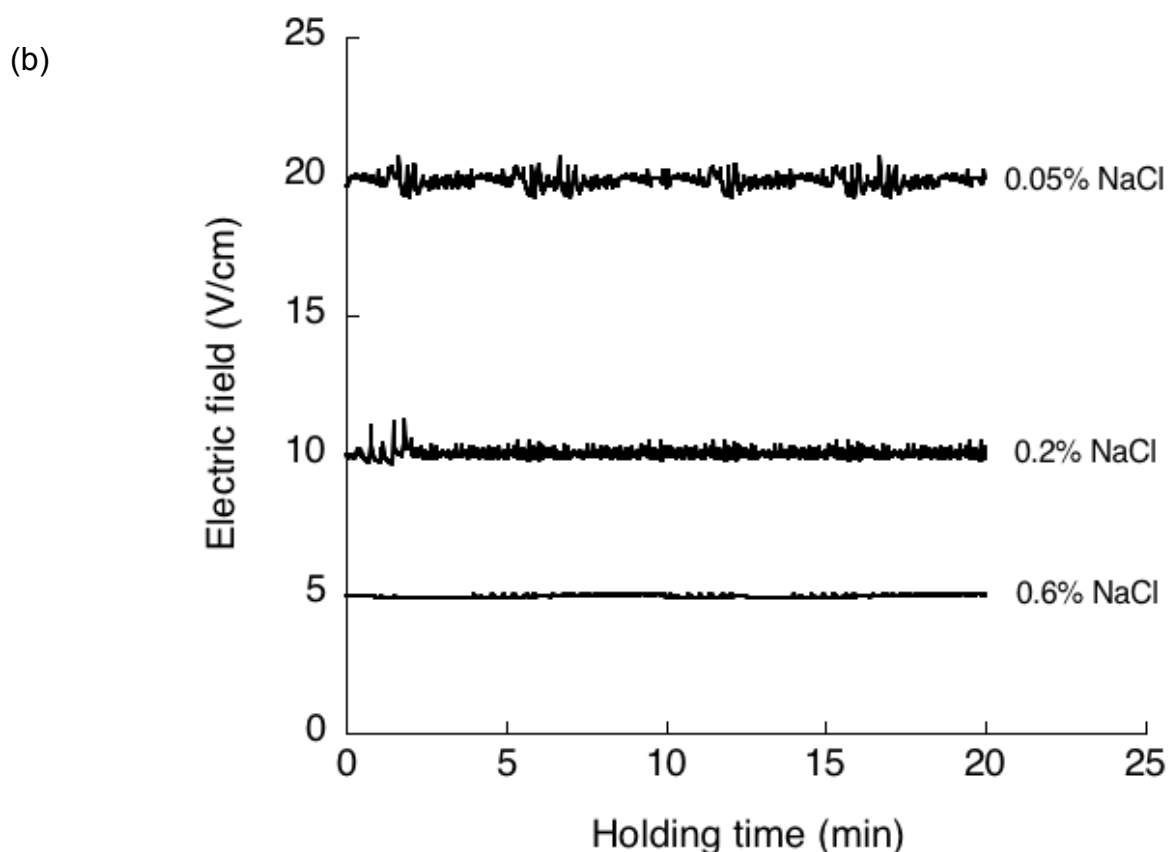
Fig. 2-2. Temperature history (a) and applied electric field history (b) for solutions with various concentrations of sodium chloride solution during ohmic heating.
