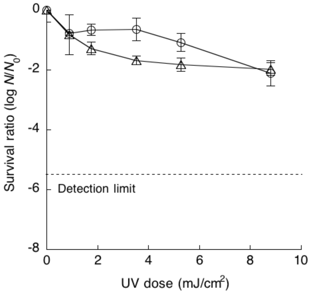
Fig. 5-3. The changes in the viable bacterial cell counts on lettuce (○) and cherry tomato (△) by UVC-LED at 0.013 mW/cm 2 . The error bars represent mean values with standard deviation (n = 3).
