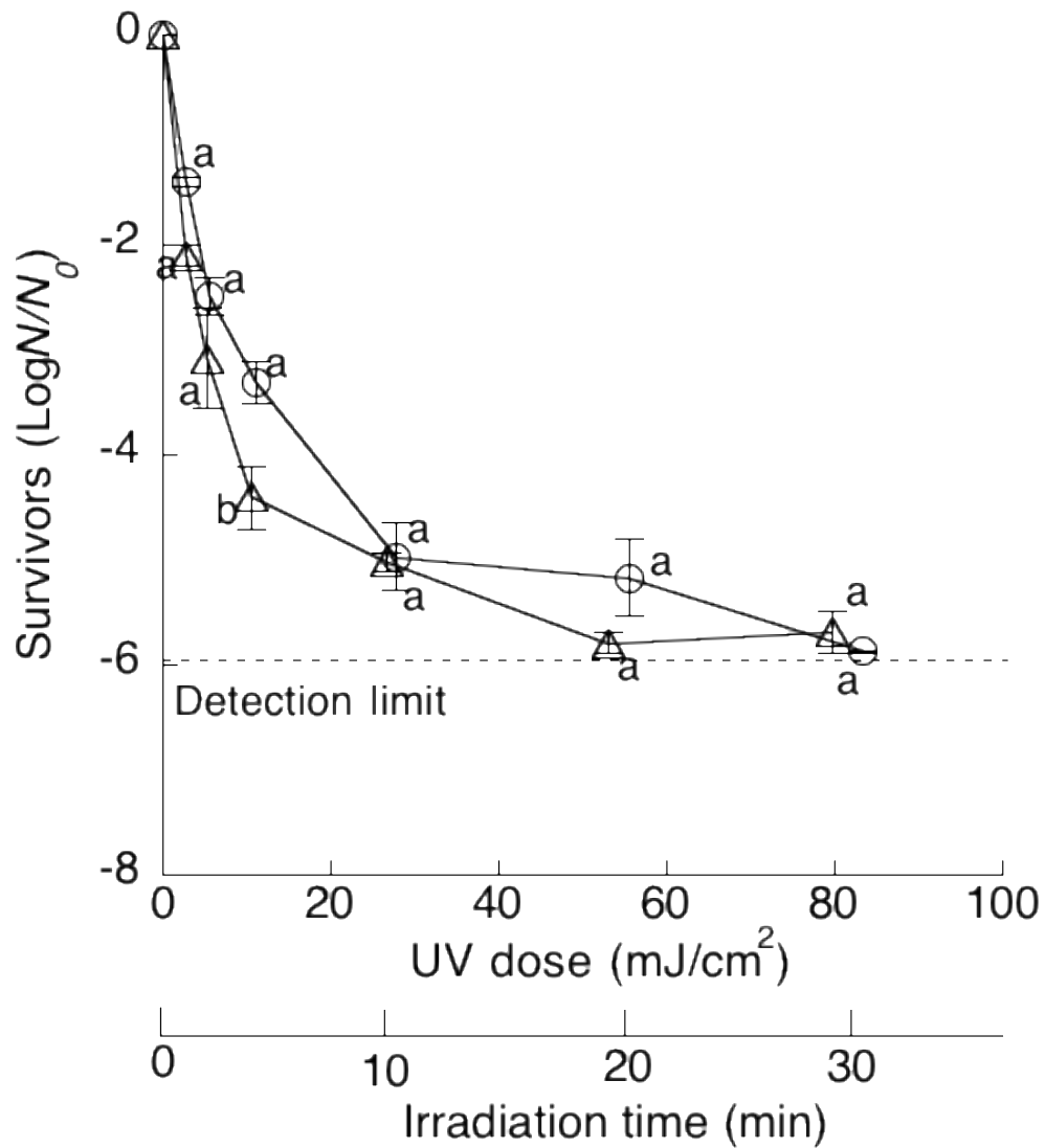
Fig. 4-5. The changes in the viable bacterial cell counts in ice during UVC irradiation at -30^{\circ}\text{C} by using three UVC-LED from the same (○) and different (△) directions. Each UVC-LED has UV intensity of 0.013\text{--}0.015\text{ mW}/\text{cm}^2 . The error bars represent mean values with standard deviation ( n = 3 ). Values with different letter means statistical significant difference.
