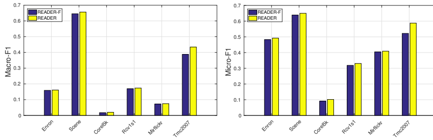
Figure 6.4: The analysis on the robustness of READER at n/N = m/M = 30\% . Here READER-F employs the square loss function in (6.17).
