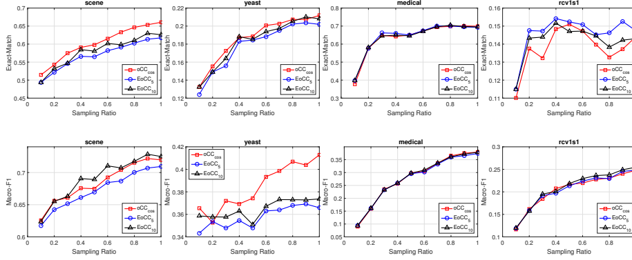
Figure 4.8: Comparison of OCC_{cos} , EOCC_5 and EOCC_{10} on four datasets in Exact-Match (the top row) and Macro-F1 (the bottom row). The sampling ratio on training instances is increased from 10% to 100% by step 10%.
