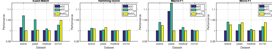
Figure 4.7: Comparison of OCC (with the canonical label order), OCC_{cos} and EOCC_5 on four datasets in four metrics. The values in each metric are normalized by dividing its minimum.
