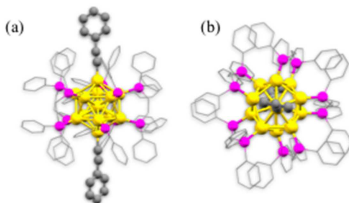
Figure 1. (a) Side and (b) top views of the crystal structure of the cationic moiety of \text{Au}_{13}(\text{C}\equiv\text{CPh})_2(\text{PF}_6)_3 . Phenylethynyl units are highlighted in light gray and the hydrogen atoms are omitted for clarity.
