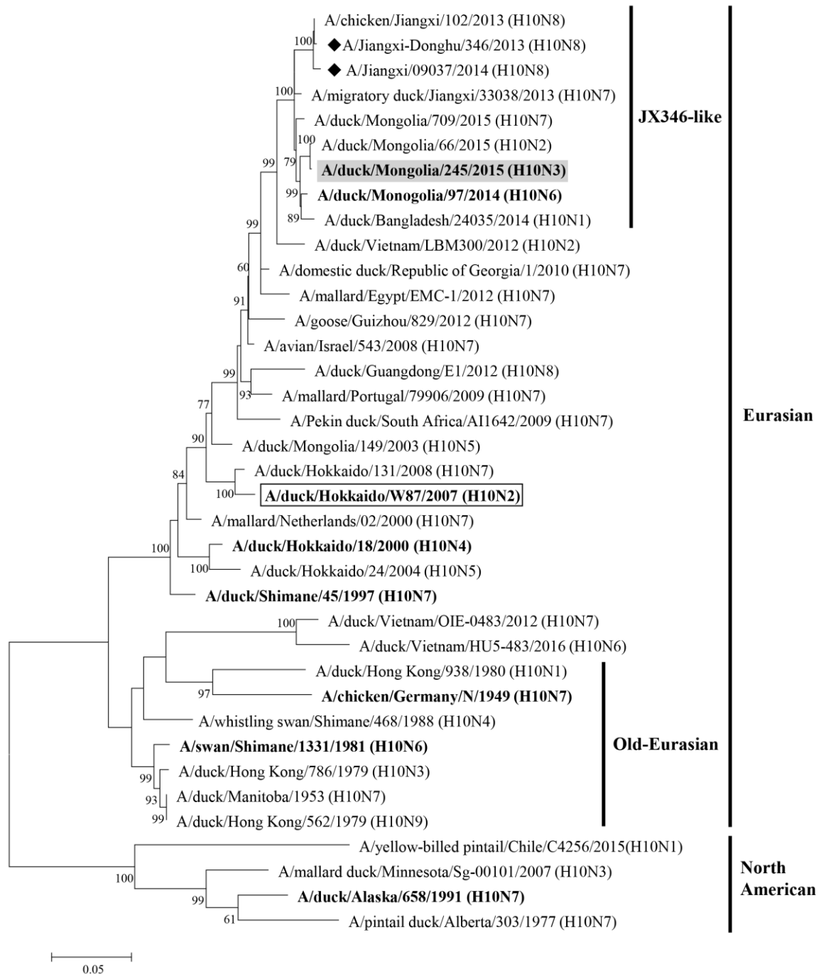
Fig. 3 Phylogenetic tree of H10 HA genes of influenza viruses Full-length nucleotide sequences of the HA gene were used for phylogenetic analysis using ML. Horizontal distances are proportional to the minimum number of nucleotide differences required to join nodes and sequences. Numbers at each node indicate the confidence level in bootstrap analysis with 1,000 replications. The viruses marked with black diamonds were isolated from human patients. The viruses used for antigenic analysis are shown in bold. The vaccine strain is highlighted in gray, and the challenge strain is enclosed in a box.
