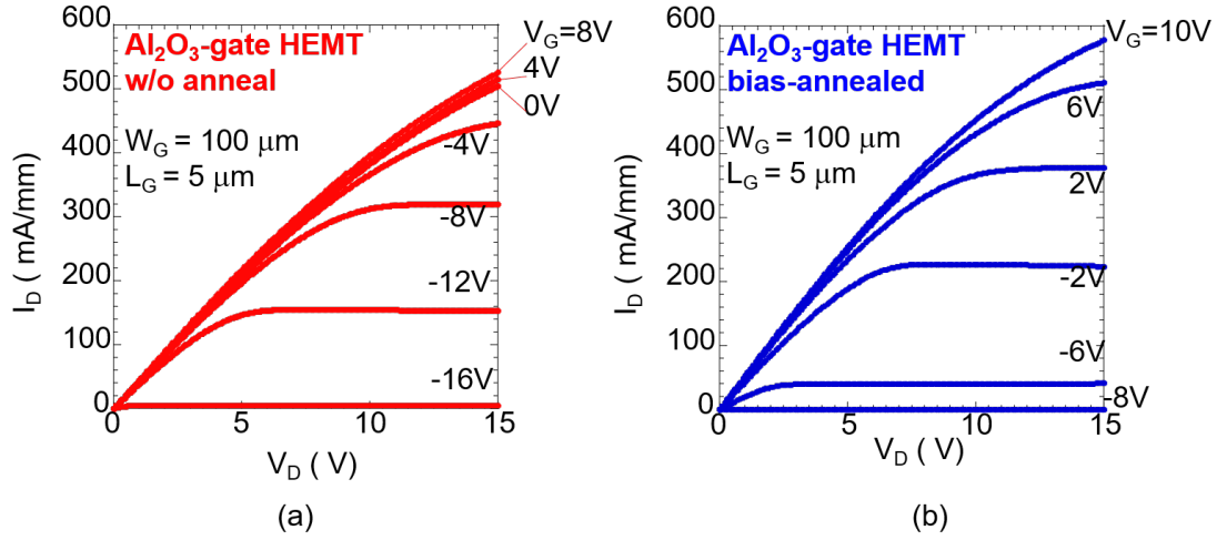
Figure 5.5. I_D - V_D characteristics of \text{Al}_2\text{O}_3/\text{AlGaIn}/\text{GaN} MOS HEMTs (a) without and (b) with the bias annealing.
