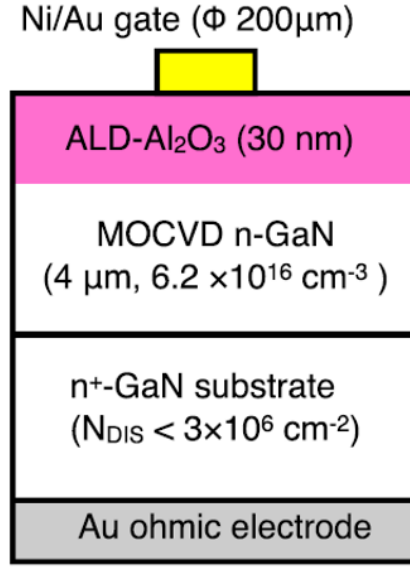
Figure 3.12. Schematic illustration of the \text{Al}_2\text{O}_3/\text{n-GaN} MOS structure fabricated on the GaN substrate.
