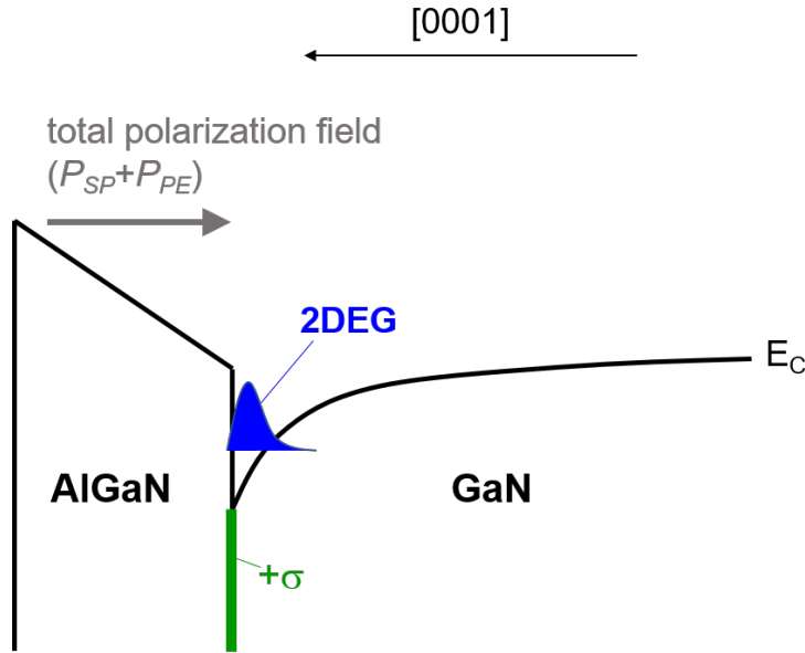
Figure 2.7. Schematic illustration of the conduction-band diagram of AlGa N /Ga N heterostructure.
