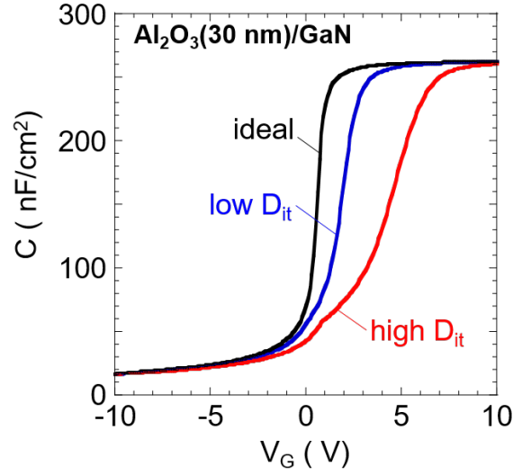
Figure 3.8. Theoretical C-V curves calculated for a Al 2 O 3 /GaN MOS diode.
