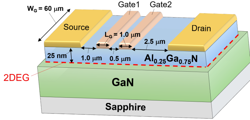
Figure 4.2. Dual-gate AlGaIn/GaN HEMT structure.
