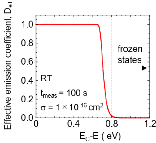
Figure 5.9. Calculated D_{eT}(E) using t_{\text{meas}} = 100 s, s = 1 \times 10^{-16} \text{ cm}^{-2} and t(E) obtained from Eq. (4).
