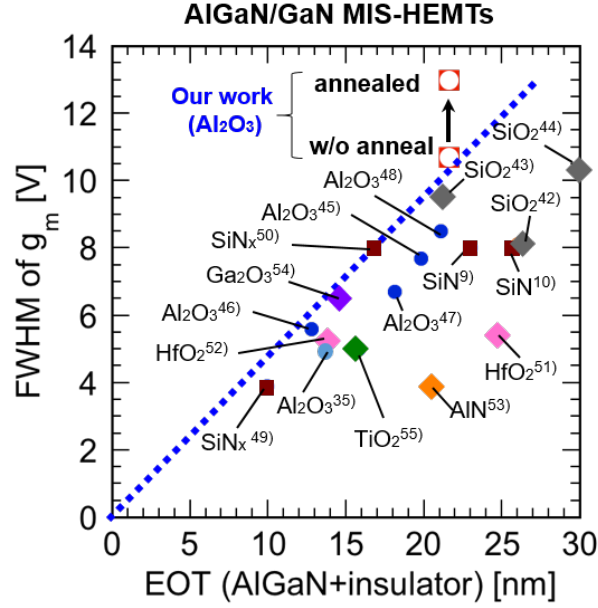
Figure 5.11. Plots of FWHM in the gm spectrum as a function of the equivalent oxide thickness (EOT) including insulator and AlGaIn barrier layers for AlGaIn/GaN MIS-HEMTs. The numbers indicate literatures cited.
