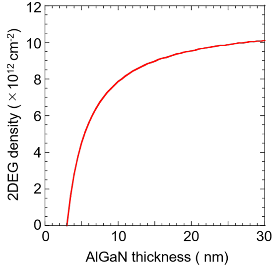
Figure 2.8. Calculated the 2DEG sheet carrier density as a function of \text{Al}_{0.20}\text{Ga}_{0.80}\text{N} barrier thickness.
