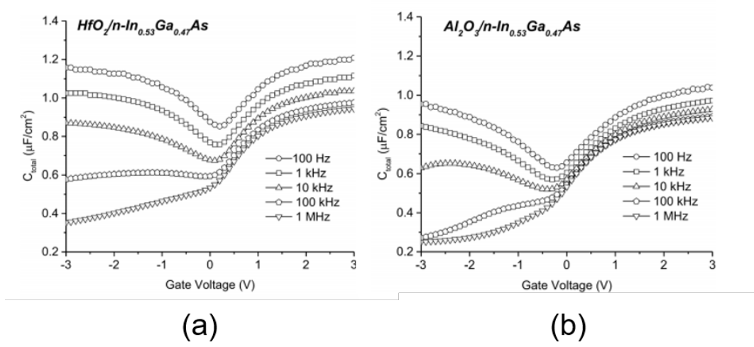
Figure 3.10. C-V characteristics as a function of frequency of (a) \text{HfO}_2 and (b) \text{Al}_2\text{O}_3 on n-InGaAs [28].
