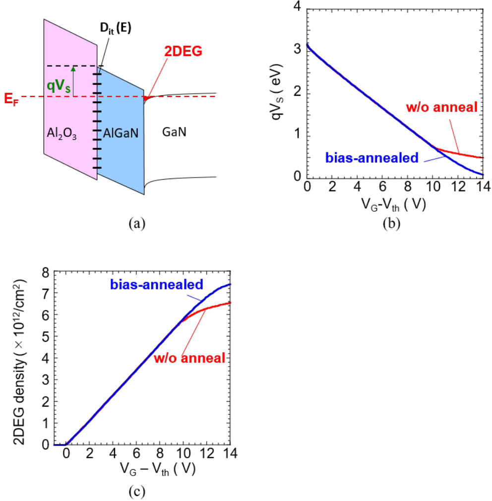
Figure 5.10. (a) Band diagram of the Al 2 O 3 /AlGaN/GaN structure. V_s indicates the AlGaN surface potential. (b) Calculated V_s as a function of V_G - V_{TH} with assuming D_{it} distributions shown in Figure 5.8. (c) Calculated 2DEG densities as a function of V_G - V_{TH} for the MOS-HEMTs without and with the bias annealing.
