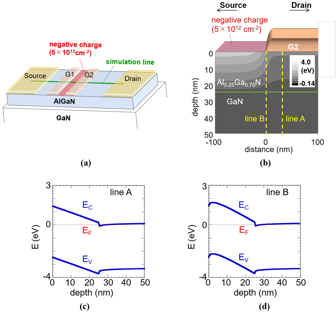
Figure 4.9. (a) Indicate the “simulation line” at the dual-gate AlGaIn/GaN HEMT. (b) Calculated 2D potential distribution near the G2 edge on the source (G1) side. Band diagram of the AlGaIn/GaN heterostructure along (c) cutline A and (d) cutline B.
