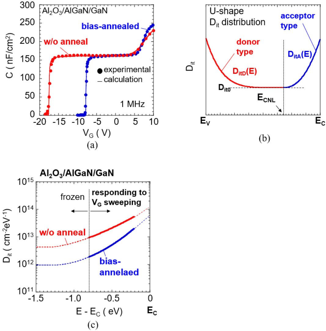
Figure 5.8. (a) C-V characteristics of the \text{Al}_2\text{O}_3/\text{AlGaIn}/\text{GaN} MOS diodes. The solid line indicates calculated curves. (b) Schematic illustration of interface state density ( D_{it} ) distribution used for calculation. (c) D_{it} distributions determined by the fitting of C-V curves.
