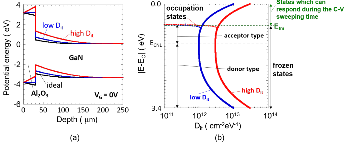
Figure 3.7. (a) Calculated potential distribution of Al 2 O 3 /n-GaN MOS diode and (b) interface states distributions used in calculation. E_{tm} is the deepest energy of the state which can respond during the C-V sweeping time.
