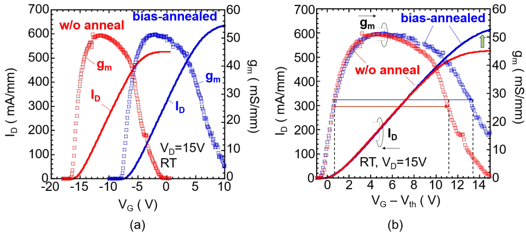
Figure 5.6. (a) Transfer characteristics of \text{Al}_2\text{O}_3/\text{AlGaIn}/\text{GaN} MOS HEMTs without and with the bias annealing process. (b) The data were replotted with respect to V_G - V_{th} .
