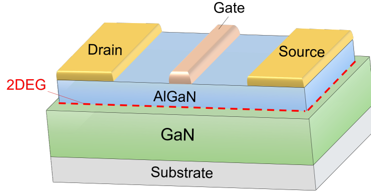
Figure 1.7. Schematic illustration of AlGaN/GaN HEMT.
