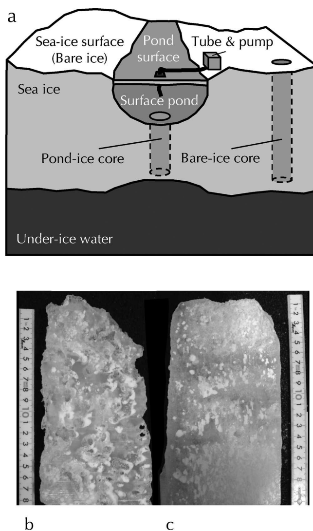
Fig. 2. (a) Schematic section of a surface pond in the sea ice, illustrating the sampling of surface pond water and pond-ice and bare-ice core collection. (b, c) Photographs of the top portions of the split ice cores in transmitted light: (b) pond-ice core and (c) bare-ice core.
