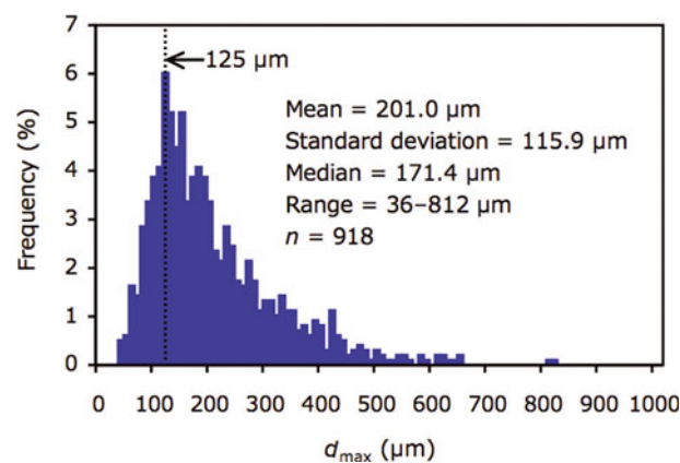
Fig. 4. Size distribution of d_{\max} for all ikaite crystals ( n=918 ) examined in this study.
