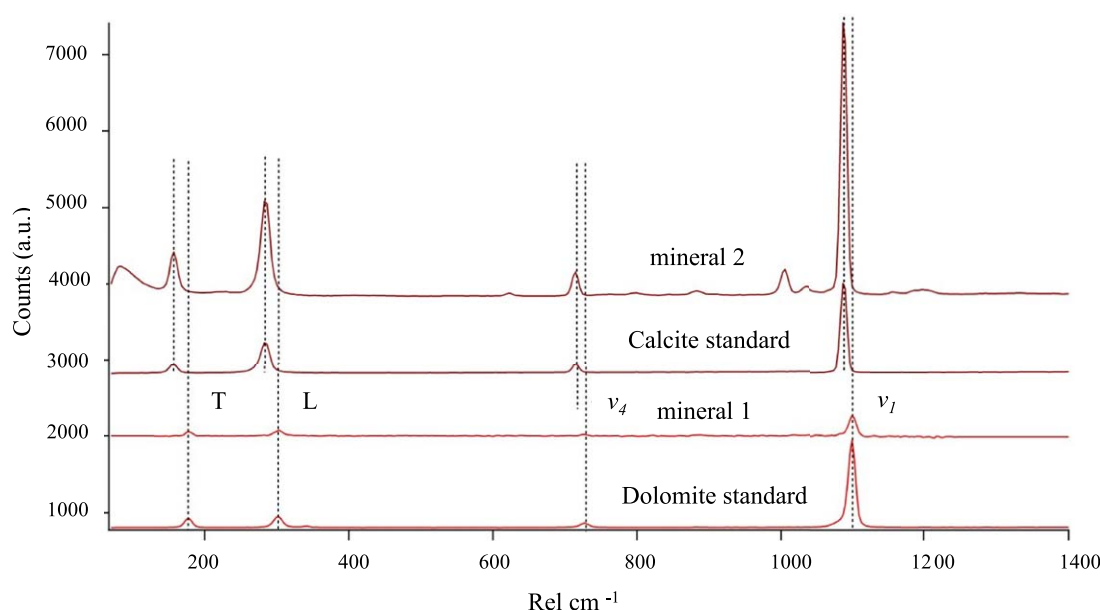
Figure 6. Raman spectra of dolomite, calcite, and two minerals (#1 and #2) from the glacial ice sample. It can be seen that the spectral position (given in relative wavenumbers; rel. \text{cm}^{-1} ) of two lattice modes (translation mode; T and librational mode; L) as well as the two internal modes (in-plane band; \nu_4 and symmetric stretch \nu_1 ) unambiguously proved the presence of dolomite and calcite in the investigated sample.
