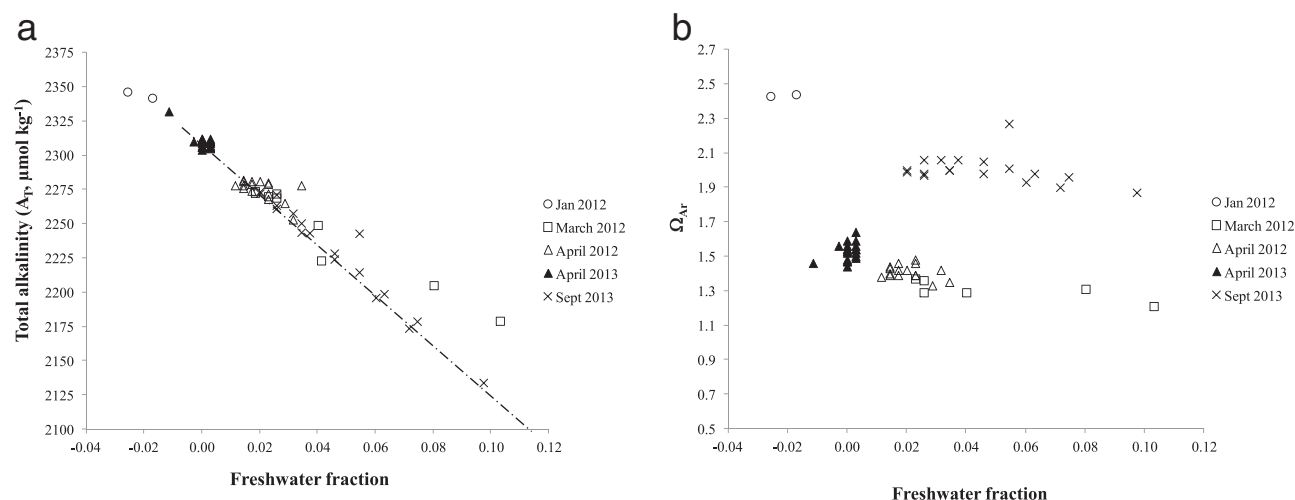
Figure 8. Freshwater fractions (x axis) versus (a) total alkalinity ( A_T , \mu\text{mol kg}^{-1} ), and (b) aragonite saturation state ( \Omega_{Ar} ) in January 2012 (open circles), March 2012 (open squares), April 2012 (open triangles), April 2013 (filled triangles), and September 2013 (crosses). The dashed dotted line in Figure 7a shows the dilution for the April 2013 data.
