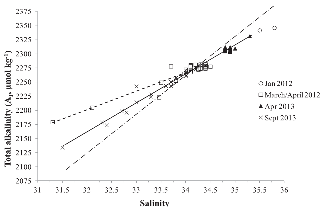
Figure 7. Linear relationship between salinity (x axis) and total alkalinity ( A_T , \mu\text{mol kg}^{-1} , y axis) during January 2012 (open circles), March and April 2012 (open squares), April 2013 (filled triangles), and September 2013 (crosses). The linear relationships were for: winter 2012 (March and April 2012) A_T = 33.08x + 1142 , R^2 = 0.901 , dashed line; for all values in 2013 (April 2013 and September 2013), A_T = 51.13x + 526 , R^2 = 0.984 , black line. The intercept of the linear relationship at zero-salinity based on 2013 values was A_T = 66.54 , R^2 = 0.895 , dashed dotted line.
