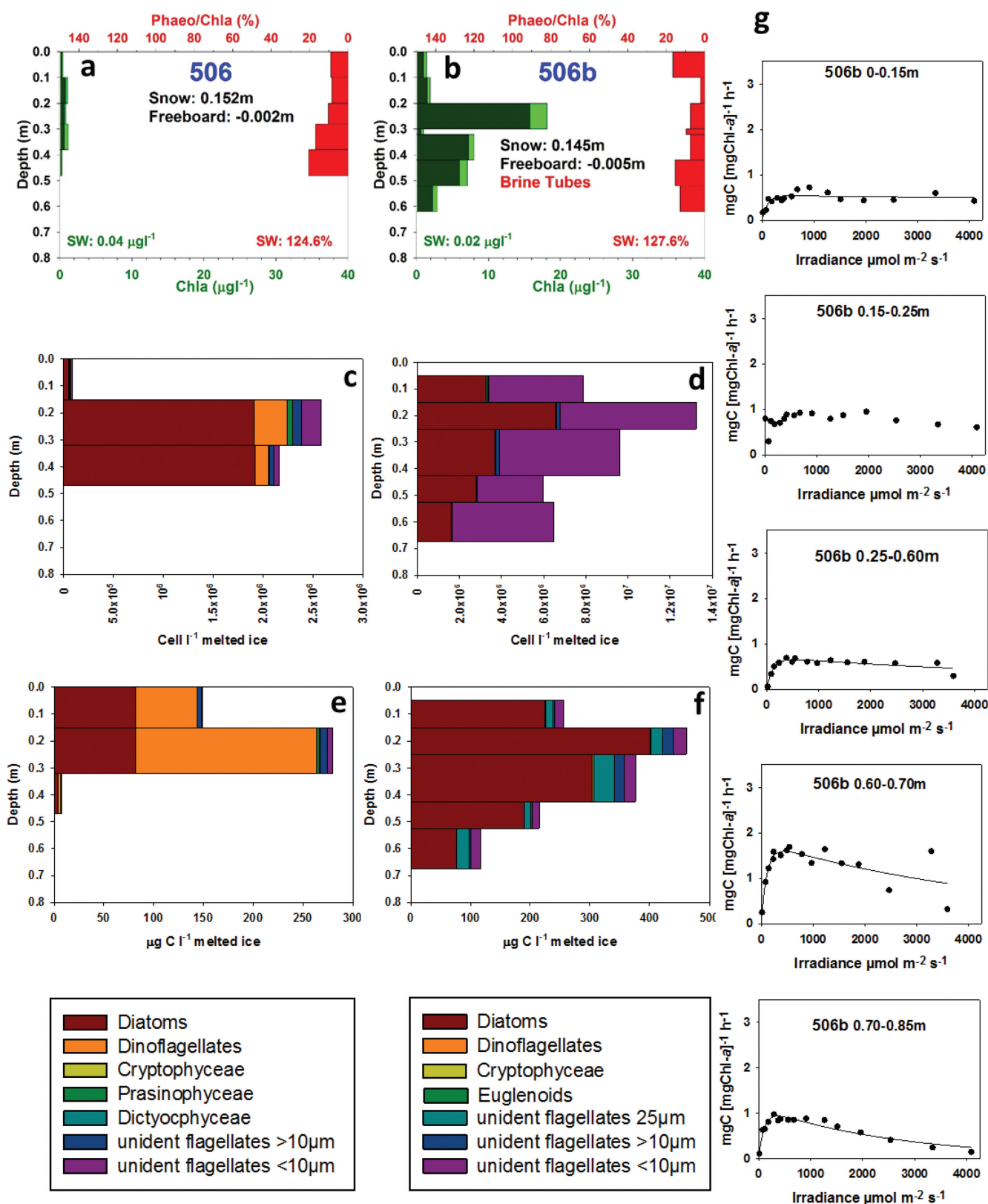
Figure 8. Biological characteristics at Station 506 (a and b are 4 days and 20 m apart)—(a and b) Chl- a (dark green = >10 \mu\text{m} ; light green = 0.8\text{--}10 \mu\text{m} ) and Phaeo-pigments to Chl- a ratio (%; red); (c and d) number of cells per liter of melted ice; (e and f) biomass in micrograms Carbon per liter of melted ice; (g) PI curves for five successive and continuous layers of station 506b. Note the difference in scales between 8c–8d and 8e–8f. See text for details.
