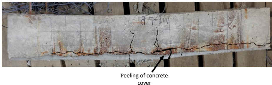
Figure 3.13. Typical crack formation of the corroded beams repaired with method 1
