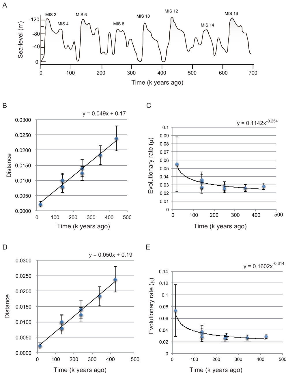
Fig. 3. (A) Sea level changes during the last 700,000 years (Bintanja et al., 2005). The p -distances for the divergences of insular lineages of Apodemus speciosus (Table 1) are plotted under the assumption that the divergences were associated with either the appearance and disappearance of land-bridge-like structures for a limited time during the glacial maxima (B) (dispersal-based calibration) or a rapid growth of population size at the beginning of warming periods after the glacial maxima (C) (expansion-based calibration). The evolutionary rates of cytochrome b in the Japanese Apodemus species computed from the dispersal-based (D) and expansion-based (E) calibrations are plotted (see Table 1 for details).
