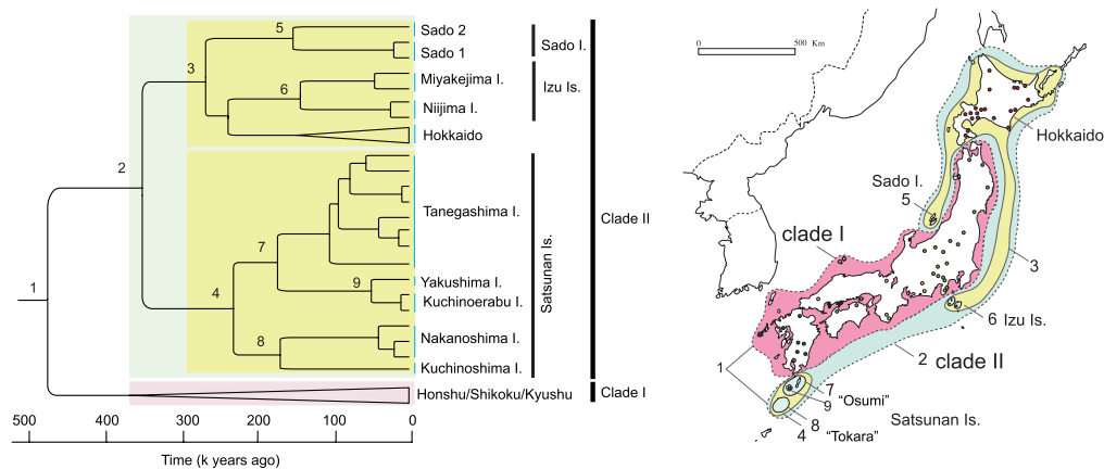
Fig. 2. A Bayesian phylogenetic tree based on mitochondrial cytochrome b sequences (1140 bp) of Apodemus speciosus (Suzuki et al., 2015), showing the geographical structure of central (Honshu, Shikoku, Kyushu) and peripheral island blocks (Sado, Hokkaido, Izu, and Satsunan Islands) (A). Numbers (1–9) of nodes indicate haplotype groups addressed in this study. A map of the Japanese Islands, showing the geographic distribution of the haplotype groups (B).
