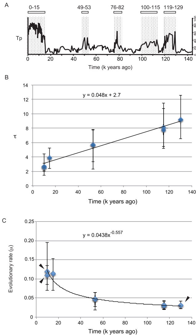
Fig. 5. Inferred climatic changes during 144,000 years based on high-resolution pollen analysis on a core from the northwest Pacific off the coast of central Japan (Igarashi and Oba, 2006) (A) . The T_p value (Kanauchi et al., 2007) is the ratio of the pollen abundance of cool-temperate broadleaf trees to the sum of that of cool-temperate broadleaf plants and subarctic conifer trees (defined by Igarashi and Oba, 2006). Five noticeable epochs of sharp increases in temperate tree species are marked (Igarashi and Oba, 2006). (B) \tau values obtained from the cytochrome b (1140 bp) analyses are plotted. The three data points were obtained based on the assumption that the rapid expansion of the mitochondrial DNA haplotype groups in Apodemus argenteus was associated with the specific geological events of rapid cooling and rapid warming 15,000, 53,000, and 115,000 years ago (Table 2). Other \tau values from our previous study for 10,000 and 130,000 years ago (arrowheads; Suzuki et al., 2015) are plotted (see Table 2 for details). (C) The evolutionary rates (substitutions/site/million years) of cytochrome b in the Japanese Apodemus species calculated from the resultant plot shown in (B) . Those predicted in a previous study (Suzuki et al., 2015) are shown with arrowheads.
