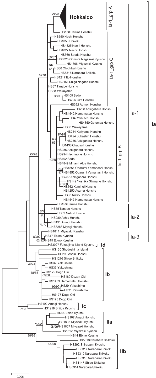
Fig. 4. An unrooted maximum likelihood tree for Apodemus argenteus based on mitochondrial DNA cytochrome b sequences. Only high bootstrap values are shown at the branches (1000 replicates, > 60%). Numbers at nodes indicate bootstrap values of maximum-likelihood and neighbor-joining methods (1000 replicates, > 60%). The taxon names correspond to those in Supplementary Table S1.
