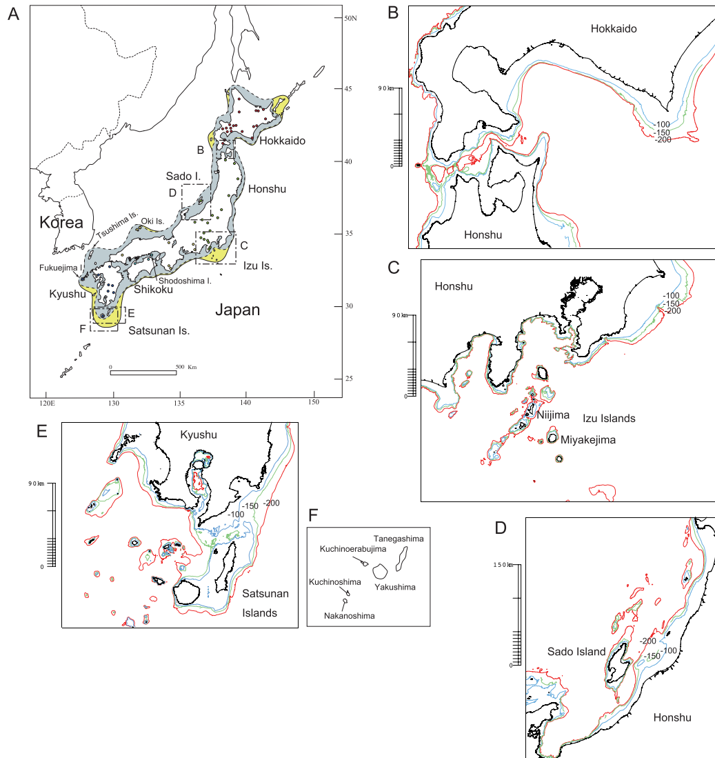
Fig. 1. Locations of the central main Japanese islands of Honshu, Shikoku, and Kyushu (A) and the peripheral islands of Hokkaido (B), Izu (C), Sado (D), and Satsunan (E, F). Rough distribution ranges of Apodemus argenteus and A. speciosus are indicated with dotted and solid lines, respectively (A). Lines indicate current sea depths of 100, 150, and 200 m (Japan Hydrographic Association) (B–E).
