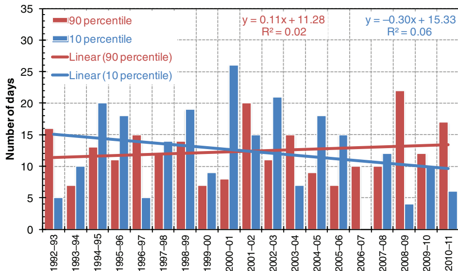
Figure 2. Multiannual values for the number of days with negative ( T_{min10} ) and positive ( T_{max90} ) winter temperature extremes with their trend lines. [Colour figure can be viewed at wileyonlinelibrary.com ].
