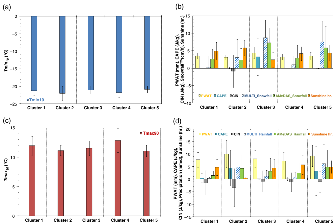
Figure 5. (a) Minimum temperature extremes ( T_{min10} ) and (b) PWAT, CAPE, CIN, snowfall (MULTI and AMeDAS), and sunshine hour for all the identified clusters. (c), (d) Same figures but for maximum temperature extremes ( T_{max90} ). [Colour figure can be viewed at wileyonlinelibrary.com .]
