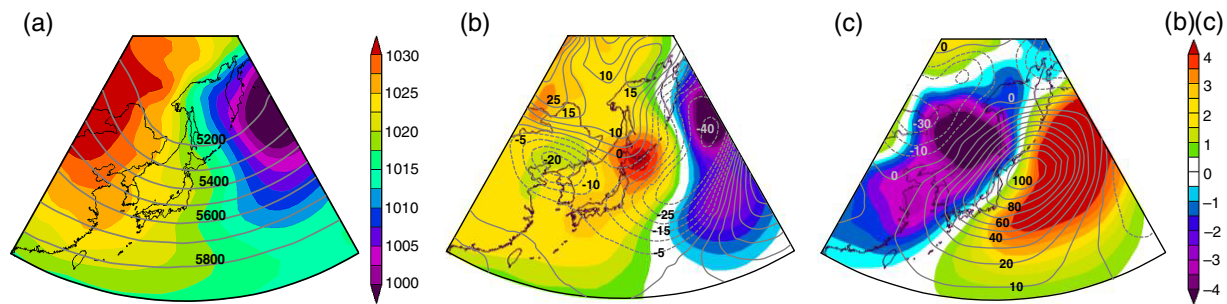
Figure 3. (a) Seasonal mean SLP in hPa (shading) and 500 hPa height in meter (solid lines) for the winter season (December–March: 1992–2011). (b) SLP (hPa) and 500 hPa height (m) of the T_{min10} composite anomaly from climatology (DJFM: 1981–2010). (c) Same as (b) but for T_{max90} . [Colour figure can be viewed at wileyonlinelibrary.com ].
