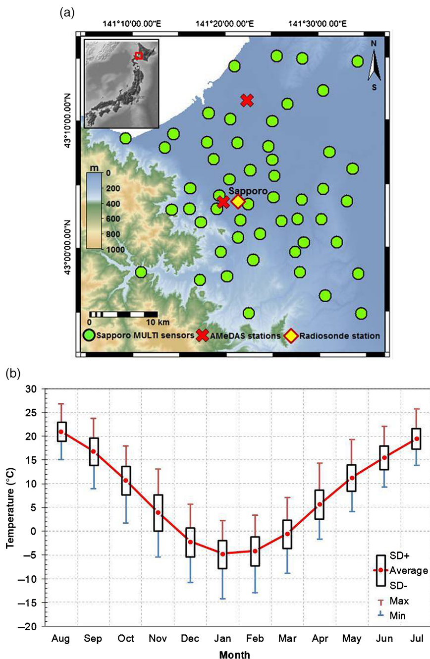
Figure 1. (a) Location of Sapporo MULTI network (52), AMeDAS (2), and radiosonde (1) stations. (b) Boxplot graph for the monthly course of air temperatures with standard deviation (box) and maximum/minimum daily means (whiskers) for the period 1992–2011 from Sapporo MULTI data set. [Colour figure can be viewed at wileyonlinelibrary.com ].
