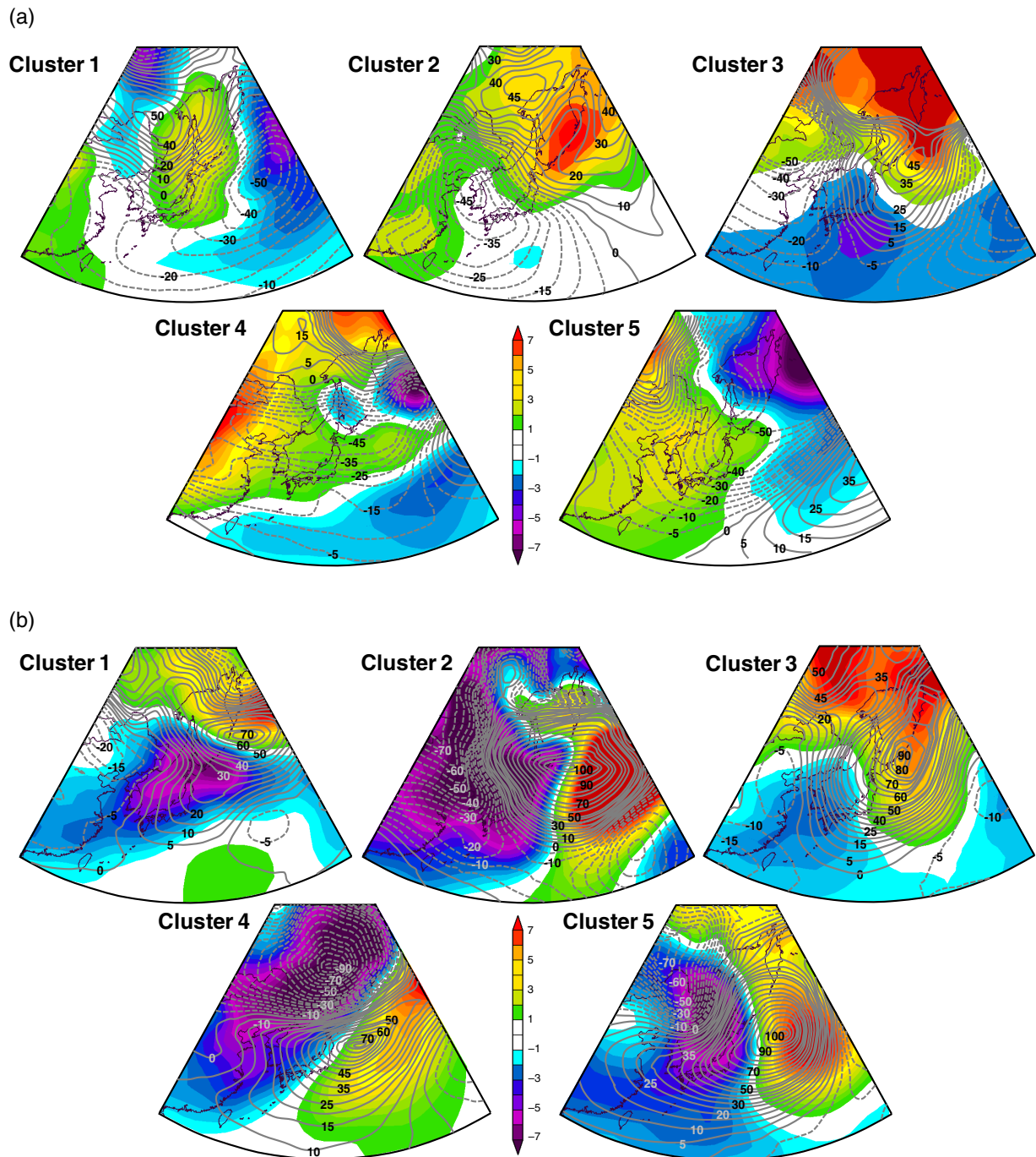
Figure 4. (a) SLP in hPa (shading) and 500 hPa height in meter [lines: solid (positive anomaly) and dotted (negative anomaly)] anomaly for the classified five groups for the days with minimum temperature extremes ( T_{min_{10}} ). (b) SLP in hPa (shading) and 500 hPa height in meter [lines: solid (positive anomaly) and dotted (negative anomaly)] anomaly for the classified five groups for the days with maximum temperature extremes ( T_{max_{90}} ). [Colour figure can be viewed at wileyonlinelibrary.com ].
