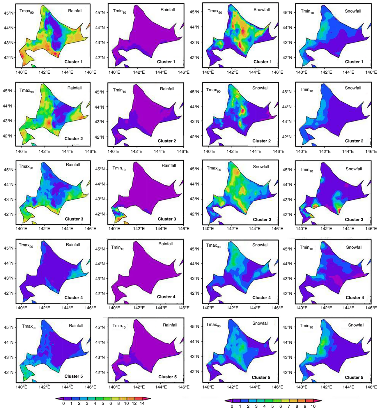
Figure 6. Spatial map of rainfall ( \text{mm day}^{-1} ) and snowfall ( \text{mm day}^{-1} ) distribution all over Hokkaido for each cluster type using AMeDAS data for maximum ( T_{\text{max}90} ; first and third panel) and minimum temperature extremes ( T_{\text{min}10} ; second and fourth panel). [Colour figure can be viewed at wileyonlinelibrary.com ].
