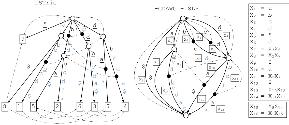
Figure 5.1: Illustration of LSTrie(T) and our index structure L-CDAWG(T) with SLP for text T = abcdcbcd\$ . Solid and broken arrows represent the edges and suffix links, respectively. Underlined and shaded characters attached to each edge are the first (real) and the following (virtual) characters of the original edge label. The expression X_i at the edge indicates the i -th variable of the SLP for T .
