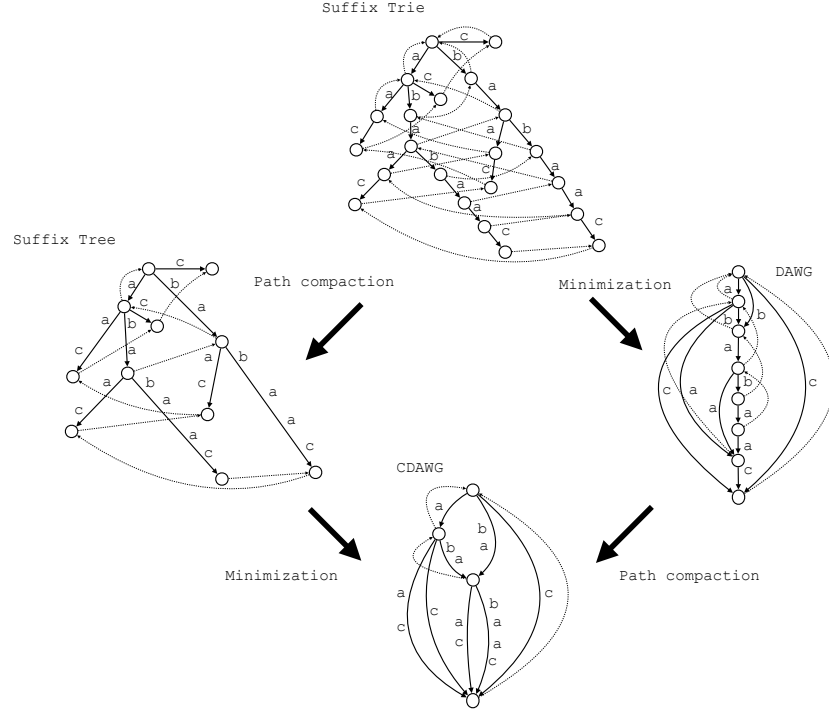
Figure 2.1: Illustration of STrie(T) , STree(T) , DAWG(T) , and CDAWG(T) with T = ababaac . The solid arrows and broken arrows represent the edges and the suffix links of each data structure, respectively.
