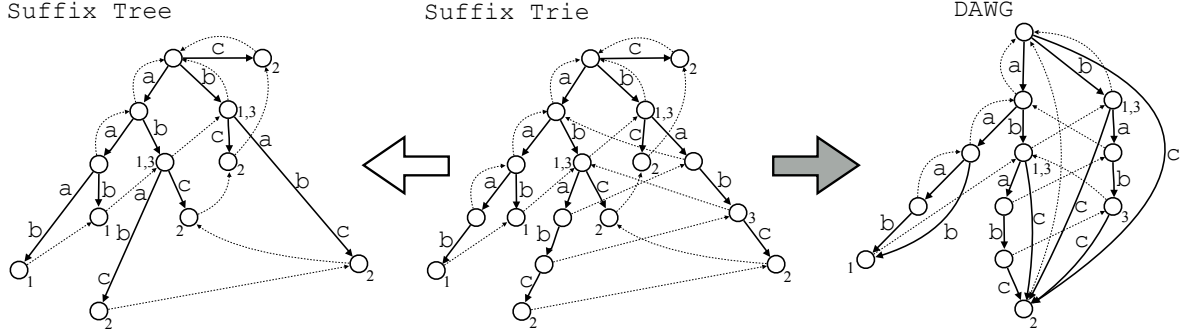
Figure 4.1: Illustration for STrie(\mathcal{T}) , STree(\mathcal{T}) , and DAWG(\mathcal{T}) with \mathcal{T} = \{T_1 = \text{aaab}, T_2 = \text{ababc}, T_3 = \text{bab}\} . The solid arrows and broken arrows represent the edges and the suffix links of each data structure, respectively. The number k ( k = 1, 2, 3 ) beside each node indicates that the node represents a suffix of T_k . The nodes [\text{ab}]_{\mathcal{T}} and [\text{b}]_{\mathcal{T}} are separated in DAWG(\mathcal{T}) since the node bab in STrie(\mathcal{T}) represents a suffix of T_3 , while the node abab does not (see also the subtrees rooted at nodes ab and b in STrie(\mathcal{T}) ).
