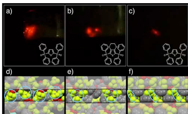
Figure 3. a-c) Pictures of TL and chemical structures of bridging ligands, and d-f) corresponding space filling models focused on intermolecular CF 3 arrangement in [Eu(hfa) 3 (dpf)] n , [Eu(hfa) 3 (dpedot)] n , and [Eu(hfa) 3 (dpt)] n .
