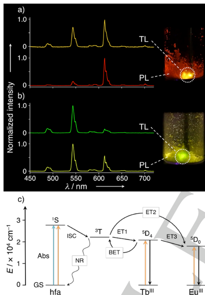
Figure 5. Normalized TL and PL spectra and pictures of a) [\text{Tb,Eu}(\text{hfa})_3(\text{dpf})]_n (Tb/Eu = 1) and b) [\text{Tb,Eu}(\text{hfa})_3(\text{dpf})]_n (Tb/Eu = 10). c) A simplified diagram of excitation processes of TL (orange line) and PL (blue line) in \text{Tb}^{\text{III}}/\text{Eu}^{\text{III}} mixed coordination polymers (Abs: absorption, ET: energy transfer, GS: ground state, ^1\text{S} : singlet excited state, ^3\text{T} : triplet excited state, ISC: intersystem crossing, NR: non-radiative relaxation).
