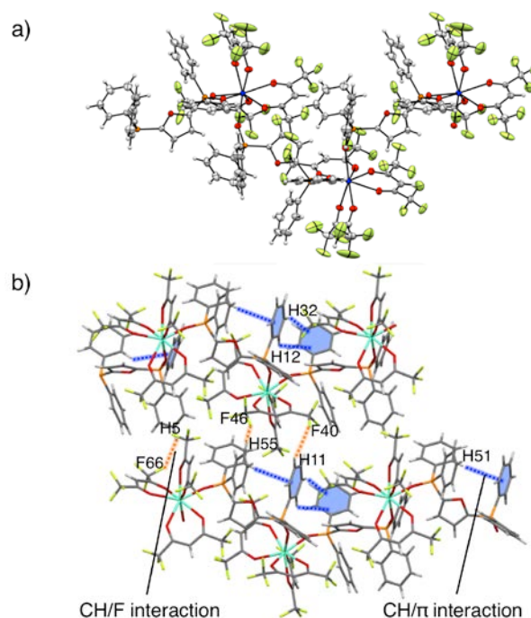
Figure 2. a) ORTEP drawing (showing 50% probability displacement ellipsoids) of single polymer chain and b) crystal packing structure focused on intra and intermolecular interactions of [\text{Eu}(\text{hfa})_3(\text{dpf})]_n .
