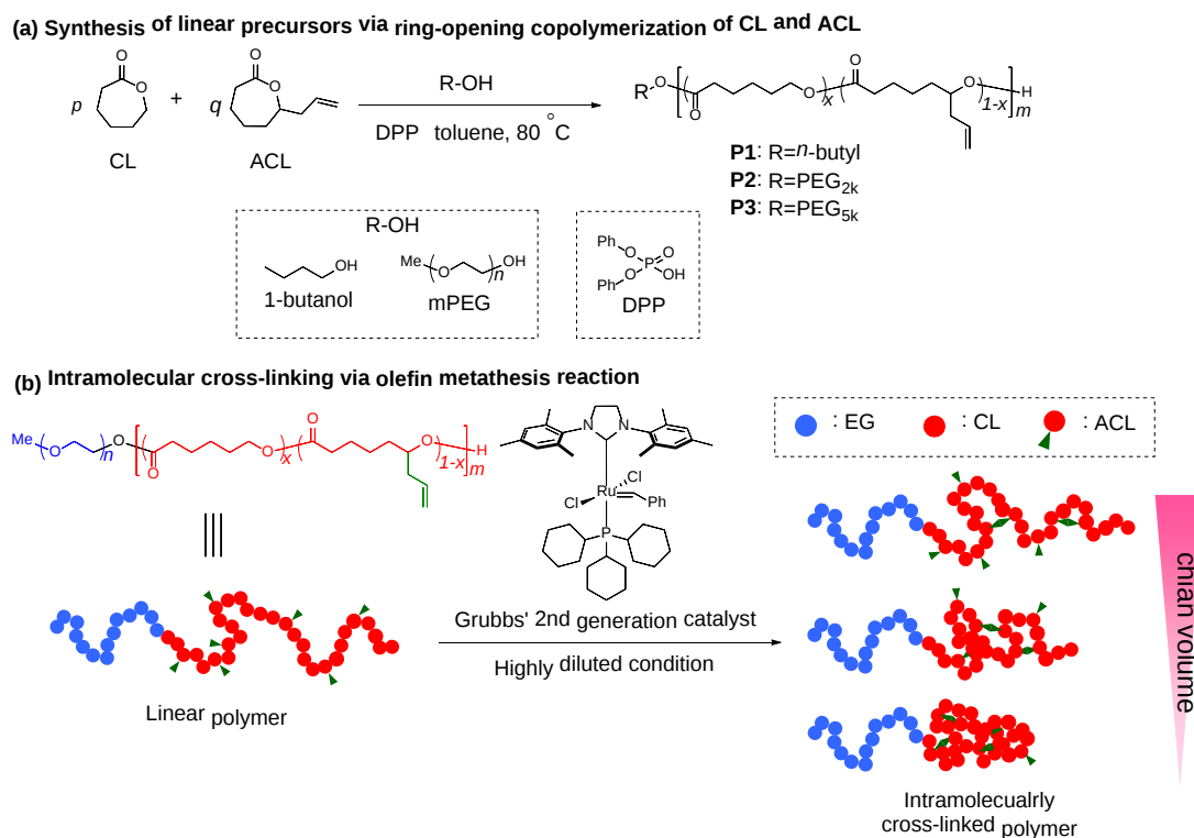
Scheme 1. (a) Diphenyl phosphate (DPP)-catalyzed ring-opening copolymerization of \epsilon -caprolactone (CL) and 7-allyloxepan-2-one (ACL) using 1-butanol or poly(ethylene glycol) monomethyl ether (mPEG) as the initiator. (b) Intramolecular cross-linking via the olefin metathesis reaction to produce a series of intramolecularly cross-linked block copolymers.
