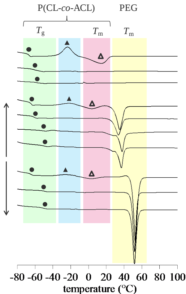
Figure 3. DSC curves during 2 nd heating process of (a) P1 , (b) P1 d,1 , (c) P1 d,2 , (d) P2 , (e) P2 d,1 , (f) P2 d,2 , (g) P2 d,3 , (h) P3 , (i) P3 d,1 , and (j) P3 d,2 at the heating rate of 10 °C min -1 . The closed circles, the closed triangles, and the open triangles denote the T_g , T_c , and T_m of the P(CL-co-ACL) blocks, respectively.
