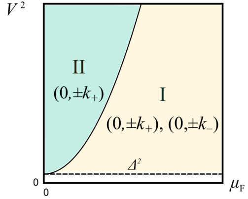
FIG. 2. Phase diagram of a Dresselhaus [110] superconductor. The solid line represents V^2 = \mu_F^2 . The dashed line represents V^2 = \Delta_s^2 .
