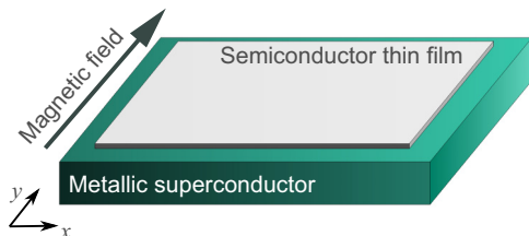
FIG. 1. Schematic image of a Dresselhaus [110] superconductor.
