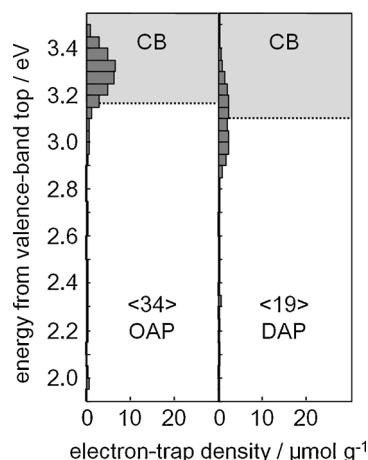
Fig. 4. Energy-resolved distribution of ET for OAP and DAP.
