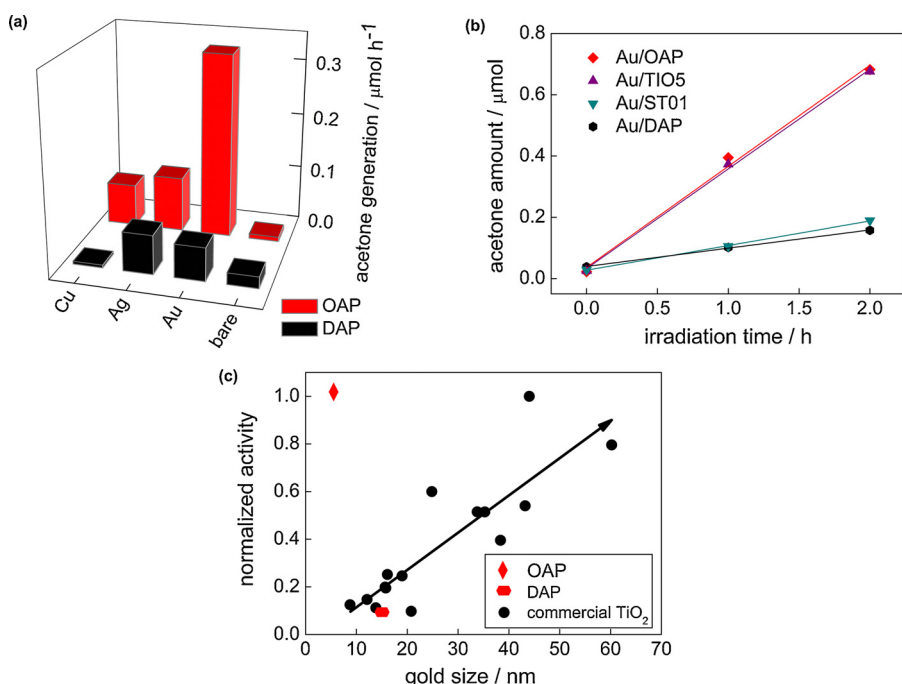
Fig. 13. (a) Visible light-photocatalytic activity for 2-propanol oxidation on bare and metal-modified OAP and DAP. (b) Comparison of visible-light photocatalytic activity of gold-modified samples based on faceted and commercial titania. (c) Correlation between gold particle size and photocatalytic activity of OAP, DAP and commercial \text{TiO}_2 .
