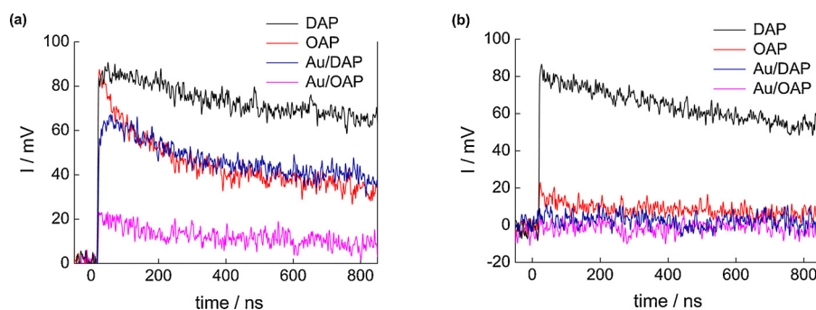
Fig. 12. Time course of TRMC signal for bare and Au-modified OAP and DAP, (a) \lambda_{\text{ex}} = 355 nm, (b) \lambda_{\text{ex}} = 545 nm.
