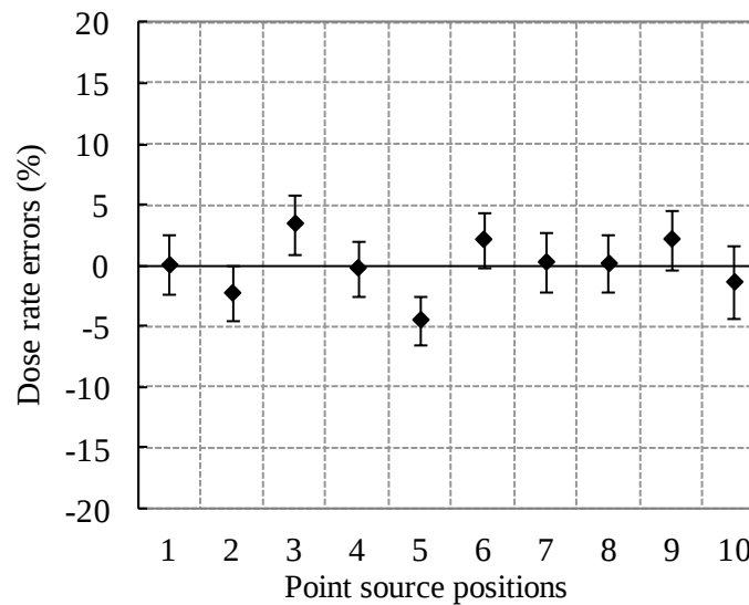
Fig. 13. Dose rate accuracy of each point in Fig. 12. Error bars denote statistical errors.
