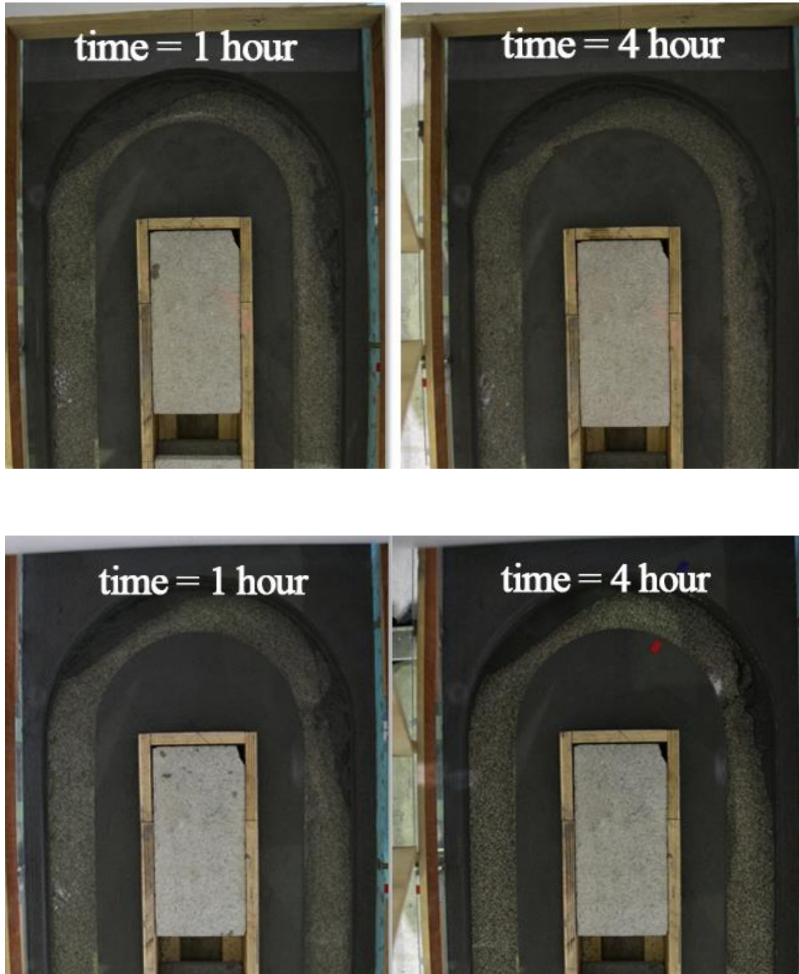
Figure 2.7: Snapshot of experimental flume at time = 1 hour and time = 4 hour. (a) Snapshots for Case 0.5. (b) Snapshots of Case 1. At time=4 hours of (a) and (b), it is apparent that bedrock in (a) is more exposed as compared to bedrock in (b).
