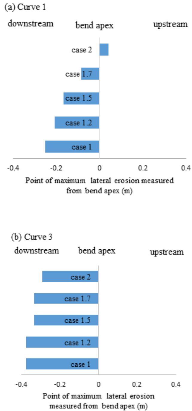
Figure 4.6. Effect of sediment feed rate. Comparison of point of maximum lateral erosion measured from bend apex in Simulation results. (a) Comparison results of curve 1 (b) comparison results of curve 3. Sediment feed rate increases from Case 1 to Case 2.
