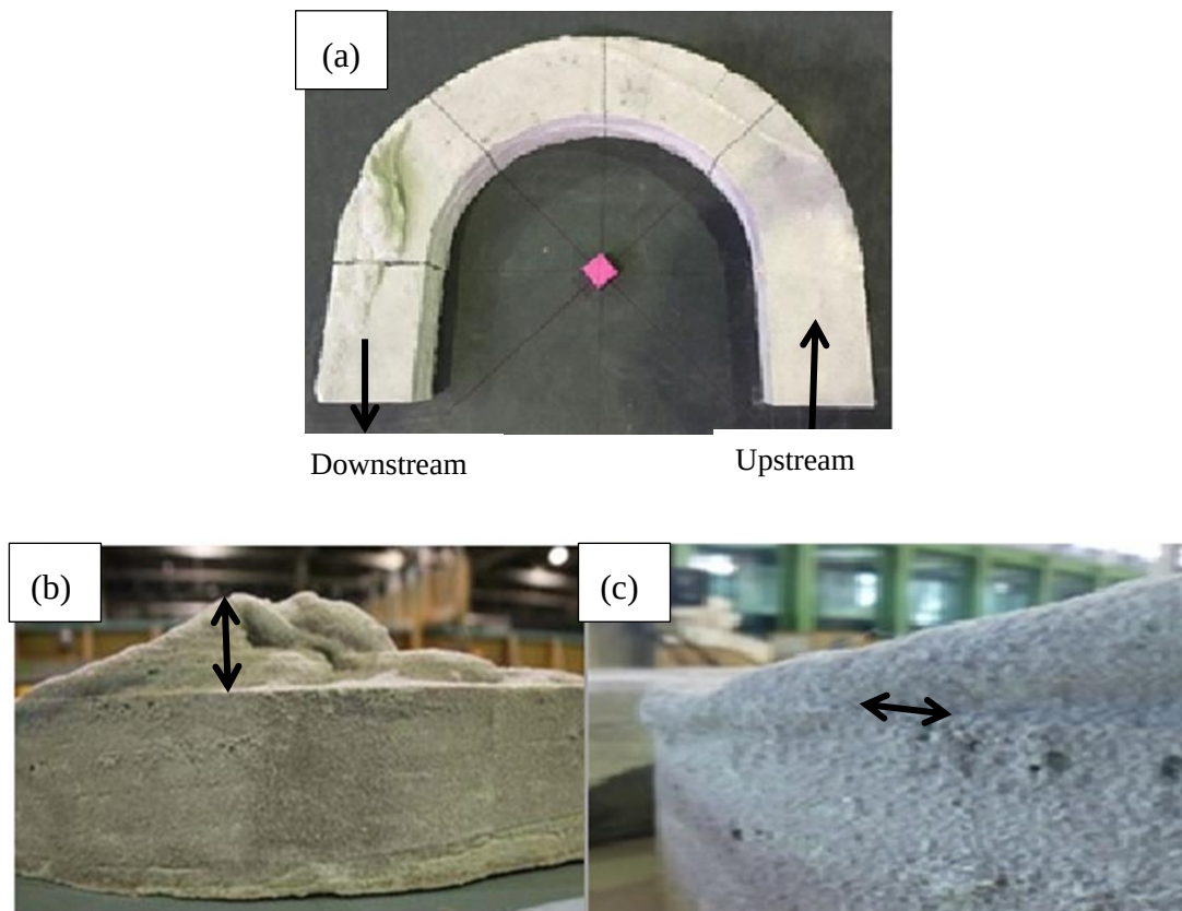
Figure 2.5 (a) Picture showing mold of the flume (b) Arrow depicting the bedrock bed erosion depth in a mold. (c) Arrow depicting bedrock bank erosion in a mold.
