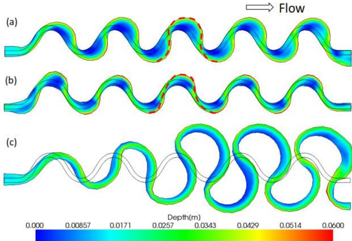
Figure.5.4 Meander bend migration. (a) Alluvial meander without bank accumulation (b) Bedrock meander without bank accumulation. (c) Alluvial meander with land accretion
