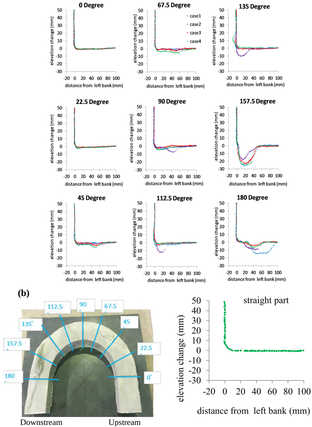
Figure 2.10: XYZ profile. (a) XYZ profile showing that bed scouring starts early, i.e. in the upstream of bend apex whereas bank erosion occurs towards the downstream of bend apex. (b) Various angles at which the XYZ profile was calculated are marked on the flume. (c) 3D scan of straight part shows no bed or wall erosion.
