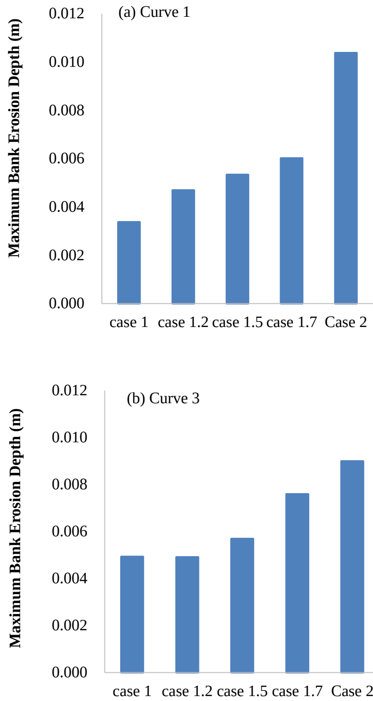
Figure 4.5. Effect of sediment feed rate in simulations. Comparison of bank erosion depth in (a) Curve 1 and (b) Curve 3. Sediment feed rate increases from Case 1 to Case 2.
