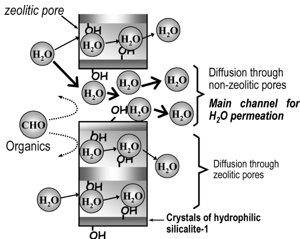
Possible relationships between the water molecules and silanol groups allowing formation of channels for water permeation.
