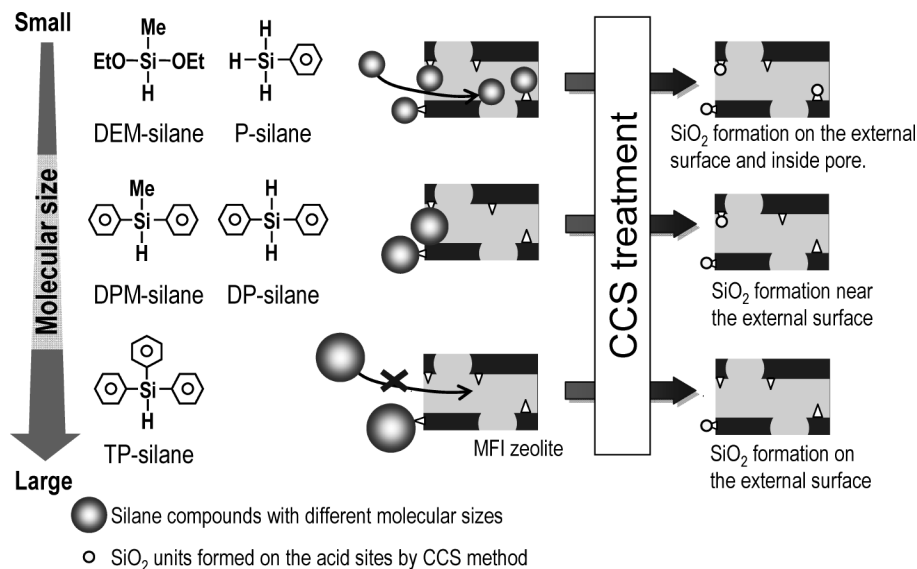
Fig. 5 Schematic Showing the Relationship between the Molecular Sizes of the Precursor Silane Compounds and the Regiospecific Deactivation of Acid Sites by the CCS Method
