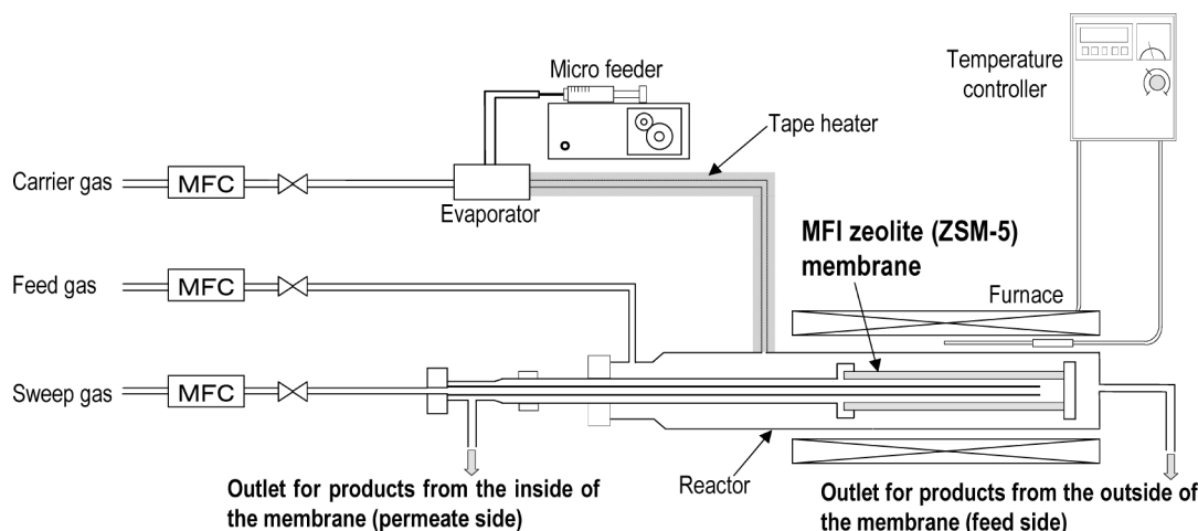
Fig. 7 Schematic of the MFI Zeolite Membrane Reactor/Separator for Gas Phase Applications
