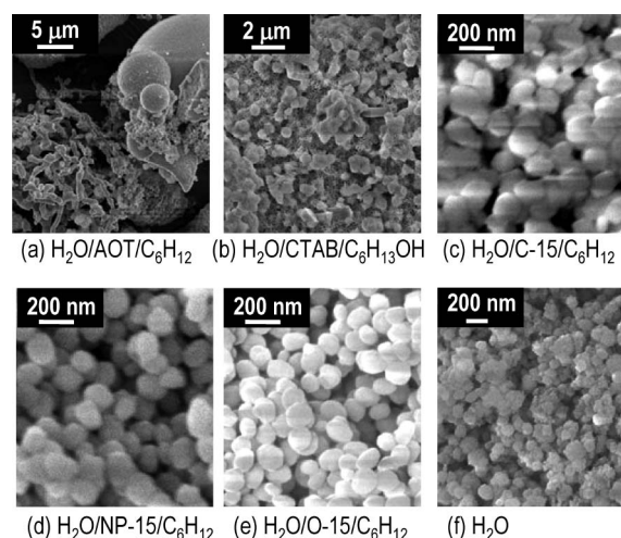
Effects of ionicity of the surfactant on the morphology of the MFI zeolite (silicalite-1). Si concentrations in water are (a)-(e) 0.63 mol/L and (f) 2.7 mol/L.
