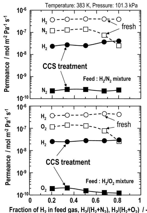
Fig. 9 Permeances of MFI Zeolite Membranes for H 2 , N 2 , and O 2 in a Flow System Using Different Molar Fractions of H 2 in the Feed Gas
