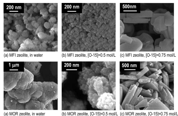
Fig. 3 FE-SEM Micrographs of MFI (silicalite-1) and MOR (Si/Al = 12.5) Zeolites with Different Crystal Sizes
