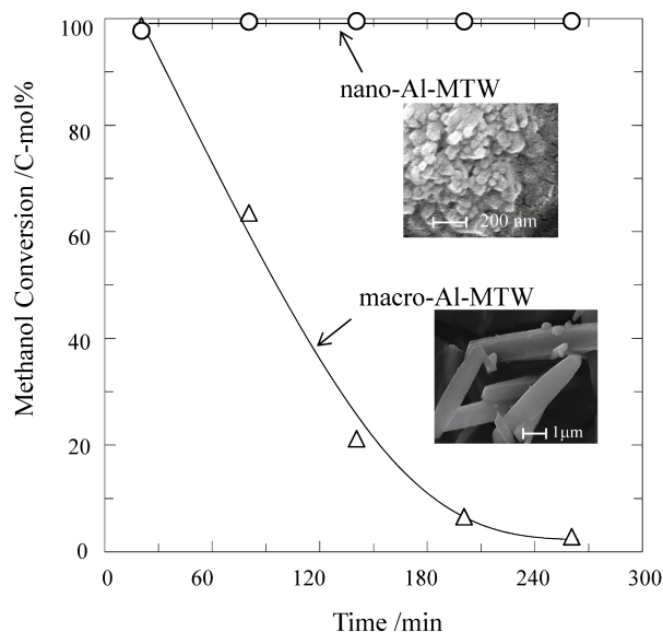
Fig. 11 Changes in Methanol Conversion with Time on Stream over Macro- and Nano-Al-MTW
