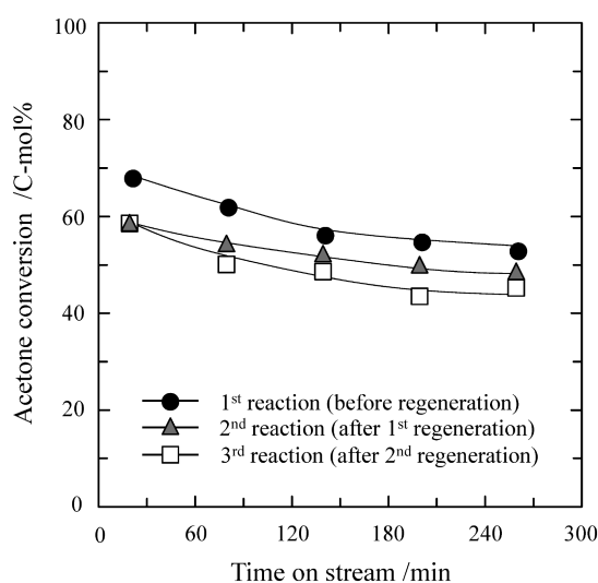
Fig. 8 Changes in Acetone Conversion with Time on Stream over Nano-Fe-MFI before/after Regeneration
