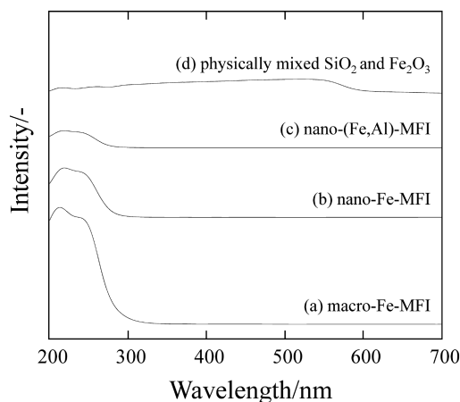
Fig. 3 UV-vis Spectra of Fe Containing Zeolites: (a) macro-Fe-MFI, (b) nano-Fe-MFI, (c) nano-(Fe,Al)-MFI, and (d) physically mixed \text{SiO}_2 and \text{Fe}_2\text{O}_3 .
