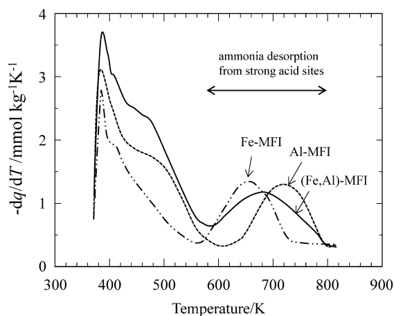
Fig. 4 ac\text{-NH}_3 -TPD Profiles of Nano-Fe-MFI, Nano-Al-MFI and Nano-(Fe,Al)-MFI
