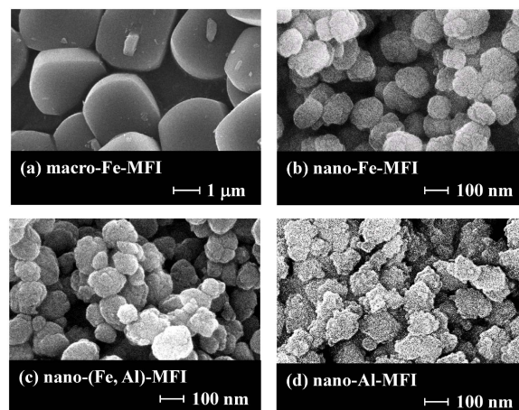
Fig. 2 FE-SEM Images of (a) Macro-Fe-MFI, (b) Nano-Fe-MFI, (c) Nano-(Fe,Al)-MFI and (d) Nano-Al-MFI Zeolites
