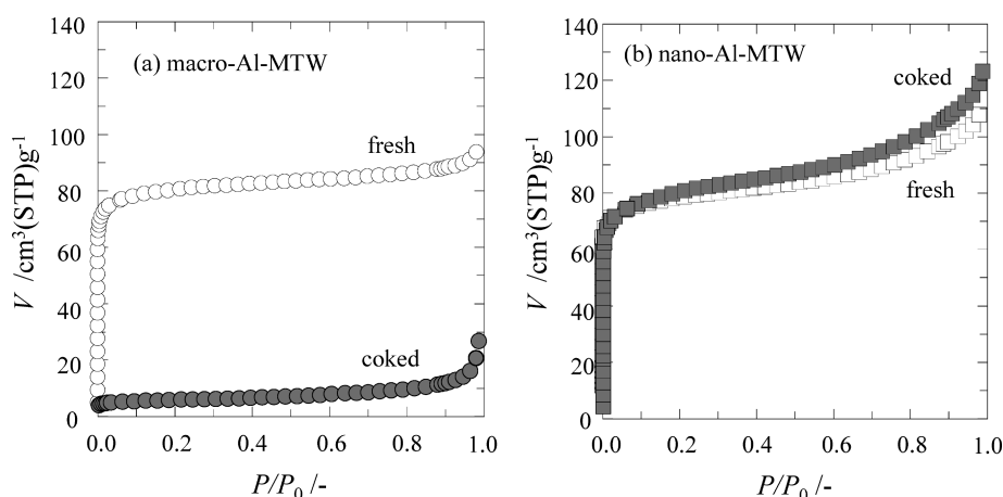
Fig. 12 Nitrogen Adsorption Isotherms of (a) Macro-Al-MTW and (b) Nano-Al-MTW before/after the Methanol to Olefins Reaction
