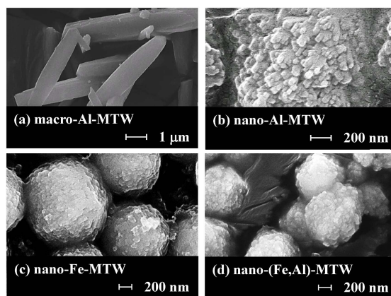
Fig. 6 FE-SEM Images of (a) Macro-Al-MTW, (b) Nano-Al-MTW, (c) Nano-Fe-MTW and (d) Nano-(Fe,Al)-MTW
