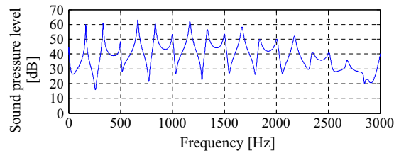
Fig. 8. Fourier spectrum of the sound pressure.
