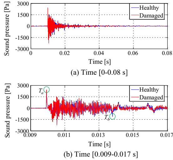
Fig. 10. Time responses in healthy and damaged (hole) conditions.
