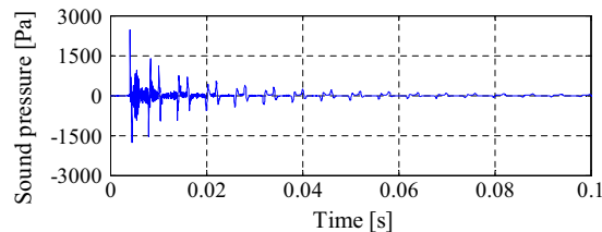
Fig. 7. Time response of the sound pressure.
