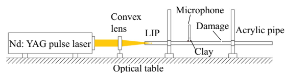
Fig. 5. Schematic of the experimental system with an LIP.
