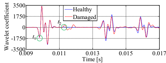
Fig. 12. Wavelet coefficients ( a = 16 ).
