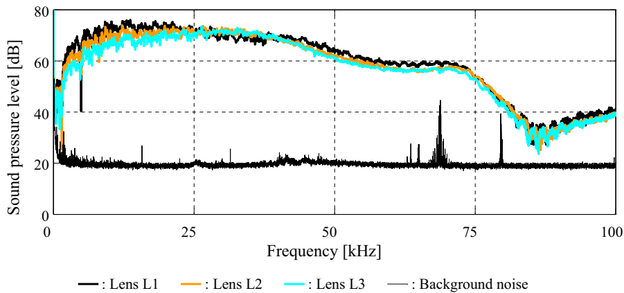
Fig. 3. Fourier spectra of sound pressure generated by LIP for three convex lenses [29].
