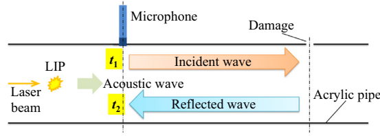
Fig. 6. Schematic diagram of the wave reflection at a damaged position.
