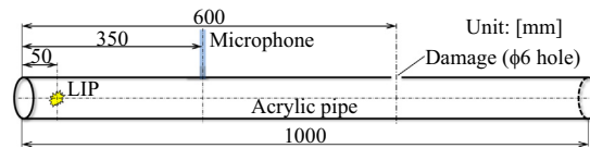
Fig. 9. Objective pipe structure with damage.
