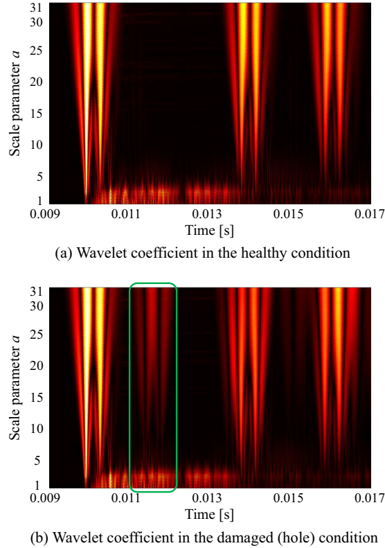
Fig. 11. Wavelet transform in healthy and damaged (hole) conditions.
