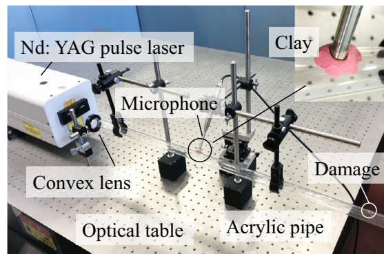
Fig. 4. Overview of the experimental system.
