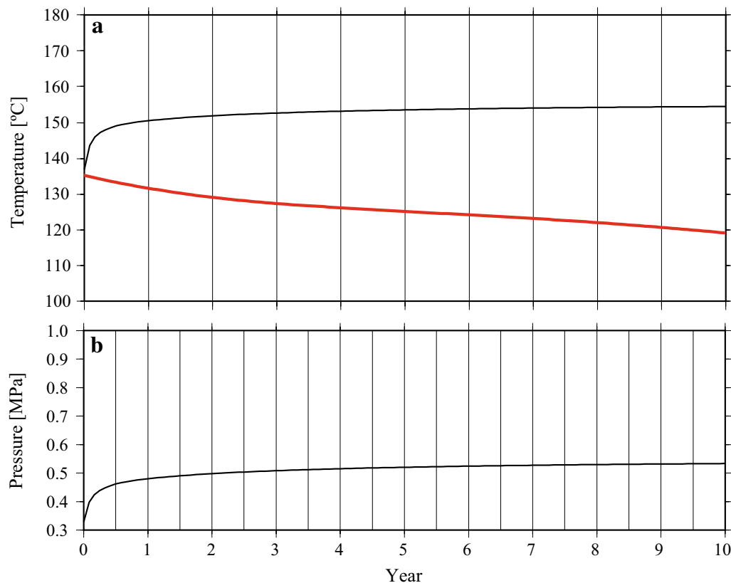
Fig. 6 Temporal change in a temperature at the crater (red line) and the observation point (black line) and b pressure at the observation point after conduit obstruction (Run 4, M' = 1000 \text{ kg s}^{-1} , k'_{\text{PCB}} = 1.0 \times 10^{-13} \text{ m}^2 )
