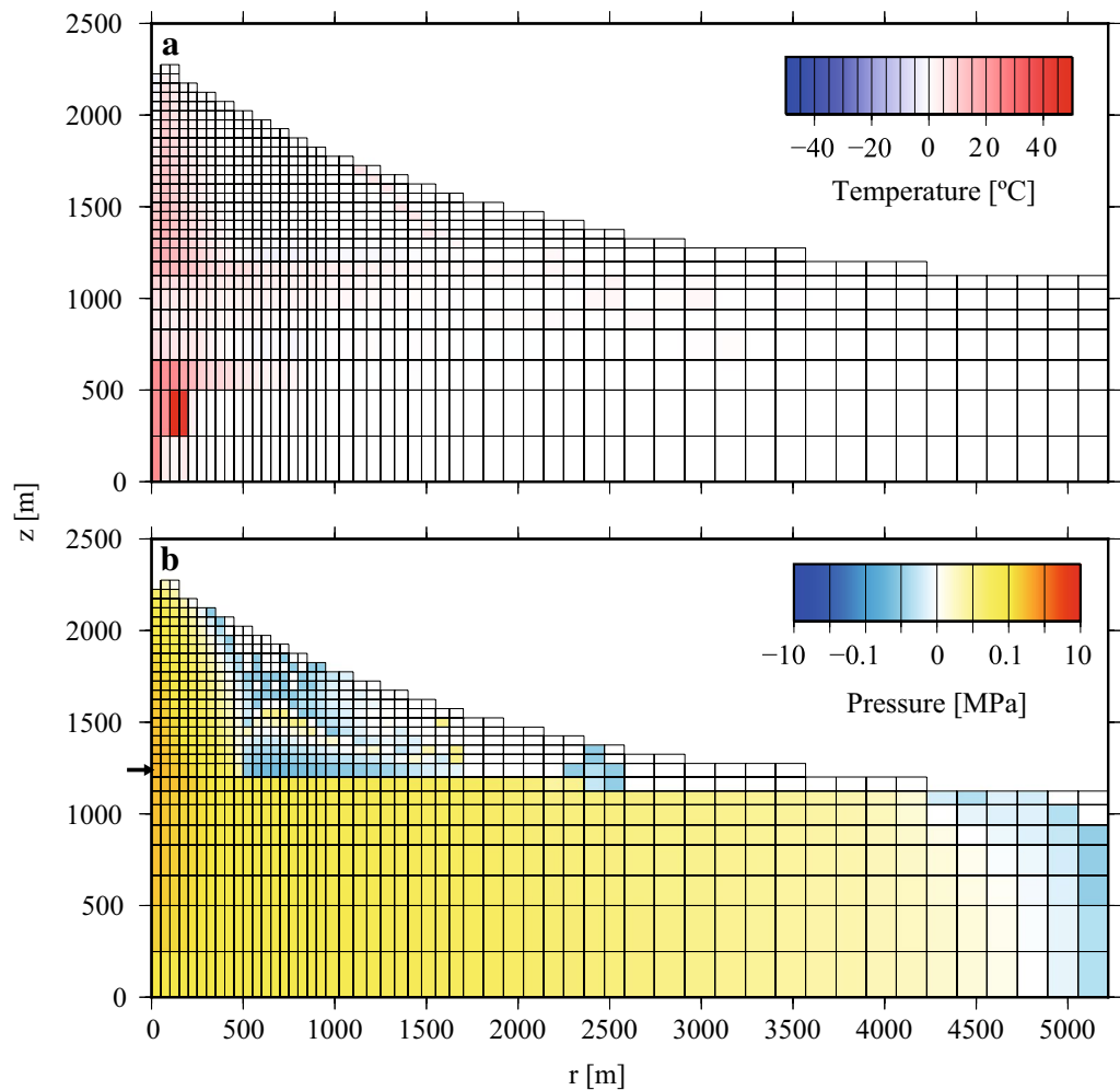
Fig. 3 Distribution of change in a temperature and b pressure 1 year after doubling the flux of hydrothermal fluid from the deep part of the system (Run 10, M' = 2000 \text{ kg s}^{-1} , k_{\text{PCB}} = 1.0 \times 10^{-10} \text{ m}^2 ). Arrow indicates the location where maximum pressure change occurs in 10-year period
