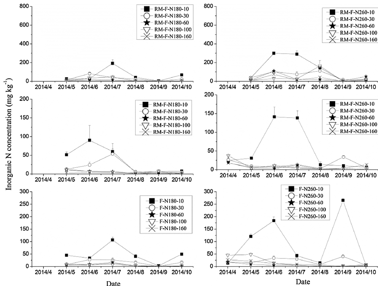
Fig. 6. Inorganic N concentrations in different soil layers during the 2014 maize growing season.
