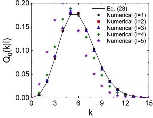
FIG. 2. Probability distribution Q_0(k|l) for Erdős-Rényi random graphs with N = 1000 and \langle k \rangle = 5.0 . Solid line indicates Q_0(k|l) given by Eq. (28), while symbols represent the numerical results for l = 1 (circles), 2 (boxes), 3 (triangles), 4 (diamonds), and 5 (stars) averaged over 100 network realizations.
