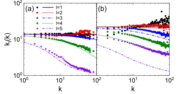
FIG. 3. Average l th neighbor degree k_l(k) of a typical node of degree k for (a) the Gnutella network [55] and (b) the coauthorship network [56]. Symbols represent k_l(k) of the real-world networks as a function of k at fixed values of l , and curves indicate those of corresponding random networks with the same degree sequences as the real networks.
