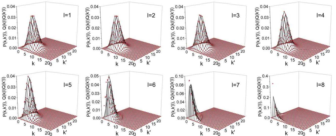
FIG. 5. Probability distributions P(k, k'|l) (wireframes) and Q(k|l)Q(k'|l) (symbols) as functions of k and k' for Erdős-Rényi random graphs with N = 1000 and \langle k \rangle = 5.0 . Each panel represents the result for l = 1 to 8 from the top left to the bottom right.
