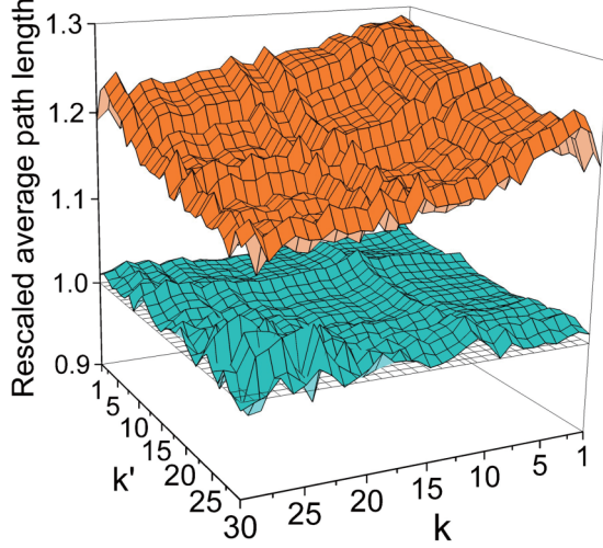
FIG. 4. Rescaled average shortest path length \langle l(k, k') \rangle_{\text{res}} between nodes of degree k and k' . The lower and upper surfaces represent the results for the Gnutella network and the coauthorship network, respectively. The bottom flat mesh indicates \langle l(k, k') \rangle_{\text{res}} = 1 .
