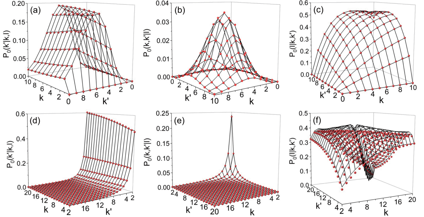
FIG. 1. Probability distributions P_0(k'|k, l) , P_0(k, k'|l) , and P_0(l|k, k') as functions of k and k' for l = 4 and N = 1000 . Wireframes indicate the distributions calculated analytically by the method explained in Sec. III B, and dots represent those measured for numerically realized random networks. Upper three panels [(a)–(c)] are the results for Erdős-Rényi random graphs with \langle k \rangle = 5.0 , and lower panels [(d)–(f)] for scale-free random networks with the degree distribution P(k) \propto k^{-3} .
