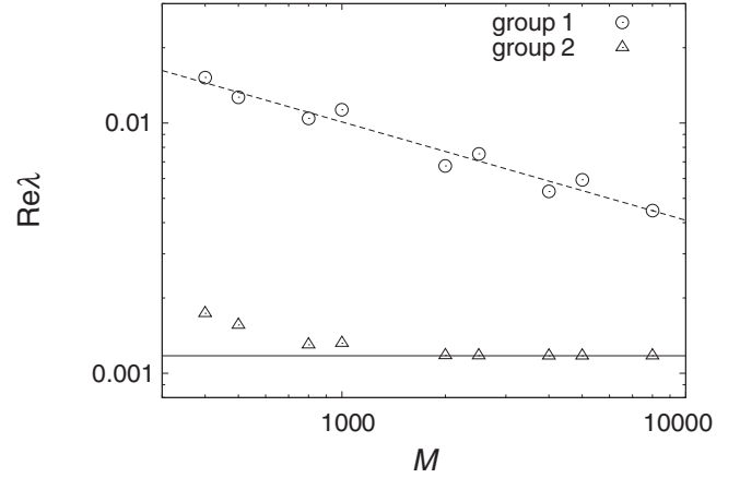
FIG. 8. Transition of the positive real parts of the eigenvalues of L_d for an unstable stationary 2-multichimera ( \alpha = 1.480 and r = 0.360 ) with increasing M . Open circles denote the maximum values of the real parts of the eigenvalues in group 1, and open triangles denote those in group 2. The data for group 1 are fitted linearly (dashed line) in the log-log plot, and go to zero with increasing M . In contrast, the data for group 2 converge to a positive constant 1.175 \times 10^{-3} (solid line).
