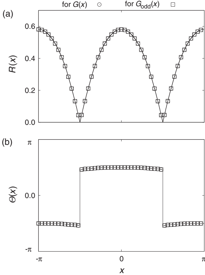
FIG. 5. Local mean field \tilde{Y}(x) of a stationary 2-multichimera. (a) The amplitude R(x) ; (b) the argument \Theta(x) . Open circles denote the time-averaged local mean field \langle \tilde{Y}(x) \rangle for Eq. (1) with the step kernel G(x) , namely, Eq. (4), with N = 100\,000 , \alpha = 1.480 , and r = 0.440 , and open squares denote \langle \tilde{Y}(x) \rangle for G_{\text{odd}}(x) with the same parameters. Note that those are plotted once every 2000 oscillators. The solid line denotes the numerical solution \tilde{Y}(x) to the self-consistency equations given by Eqs. (12) and (13) with G_{\text{odd}}(x) .
