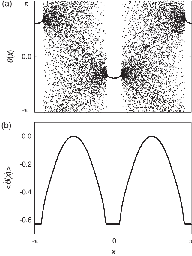
FIG. 1. Multichimera state with two coherent and incoherent regions for Eq. (4) with N = 10\,000 , \alpha = 1.480 , and r = 0.360 . (a) The snapshot of the phase \theta(x, t) . (b) The profile of the average frequency \langle \dot{\theta}(x) \rangle with T = 2000 .
