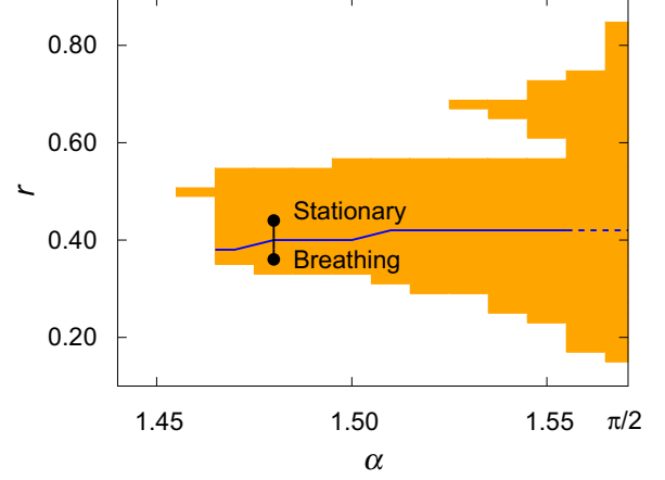
FIG. 2. Stability region of 2-multichimera for Eq. (4) obtained by the numerical simulation with N = 100\,000 . Black circles denote the parameter values of Fig. 3. The blue line denotes the Hopf bifurcation points obtained by the linear stability analysis for the stationary 2-multichimera with fixed \alpha in Sec. IV, but we could not determine those points for \alpha close to \pi/2 (dashed line).
