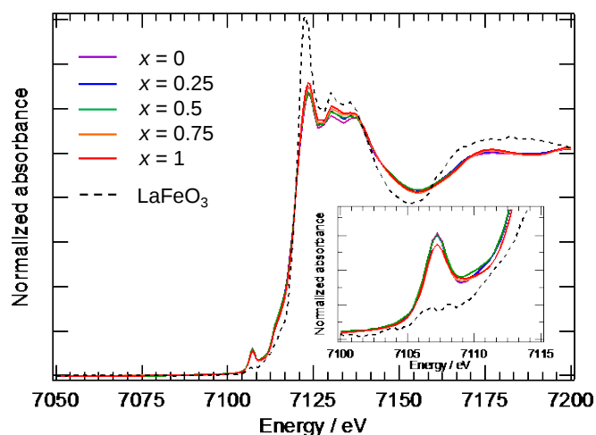
Figure 3. Fe K-edge XANES spectra of \text{Ca}_2\text{Fe}_{2-x}\text{Co}_x\text{O}_5 and \text{LaFeO}_3 . The inset represents enlarged spectra in the vicinity of the pre-edge peak attributable to Td\text{-Fe} in \text{Ca}_2\text{Fe}_{2-x}\text{Co}_x\text{O}_5 .
