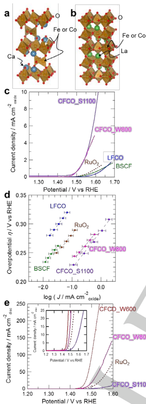
Figure 1. (a) Crystal structures of BM-type \text{Ca}_2\text{FeCoO}_5 (CFCO) and (b) its isoelectronic reference oxide, PV-type \text{LaFe}_{0.5}\text{Co}_{0.5}\text{O}_3 (LFCO). The illustrations were drawn with VESTA software [29] based on the structural model reported in the literature. (c) Linear sweep voltammograms of CFCO_S1100, W800, LFCO, BSCF and \text{RuO}_2 for OER. The current density was normalized with the specific surface areas. (d) Tafel plots of CFCO_S1100, W800, LFCO, BSCF and \text{RuO}_2 . Error bars represent standard deviations from at least four independent measurements. (e) Linear sweep voltammograms of CFCO_S1100, W800, W600, and \text{RuO}_2 . The current density was normalized with the geometric surface area of the disc electrode. All the measurements were conducted at room temperature in a 4 \text{ mol dm}^{-3} KOH aqueous solution. It should be emphasized that the usage of concentrated alkaline solutions is mandatory for constructing practical metal-air secondary batteries to enhance the ionic conductivity of the electrolyte and to suppress corrosions of the negative electrodes. Such OER data with high KOH concentrations are thus informative to evaluate the performance in practical metal-air secondary batteries.
