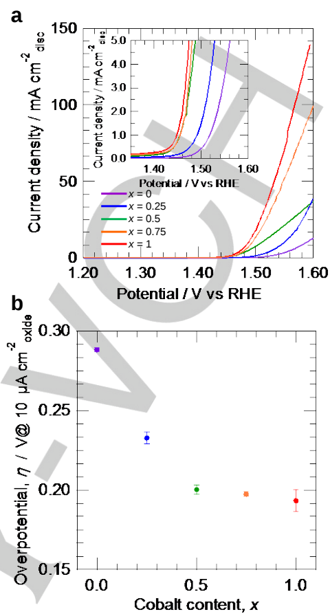
Figure 2. (a) Linear sweep voltammograms of \text{Ca}_2\text{Fe}_{2-x}\text{Co}_x\text{O}_5 ( 0 \leq x \leq 1 ) for OER. The samples were synthesized via a wet-chemical route with a firing temperature of 800^\circ\text{C} . The current density was normalized with the geometric surface area of the disc electrode. (b) The overpotentials ( \eta ) vs cobalt content ( x ) relation for \text{Ca}_2\text{Fe}_{2-x}\text{Co}_x\text{O}_5 ( 0 \leq x \leq 1 ). The \eta values were determined from the onset potential E_{\text{onset}} ; E_{\text{onset}} is the potential to give a current density, which was normalized with the specific surface areas (Table S2), of 10 \mu\text{A cm}^{-2} oxide.
