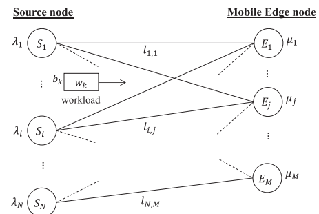
Fig. 4 Problem model
