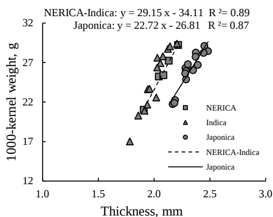
Figure 3 Relationship between weight and thickness of rough rice.
