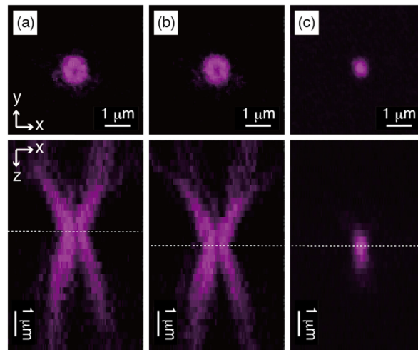
Fig. 4. Reconstructed fluorescent images of a 100 nm Red bead, excited by both the STED and two-photon excitation lights. (a) STED light, minimum voltage applied to the tLCD-G. (b) STED light, maximum voltage applied to the tLCD-G. (c) Two-photon excitation light.
