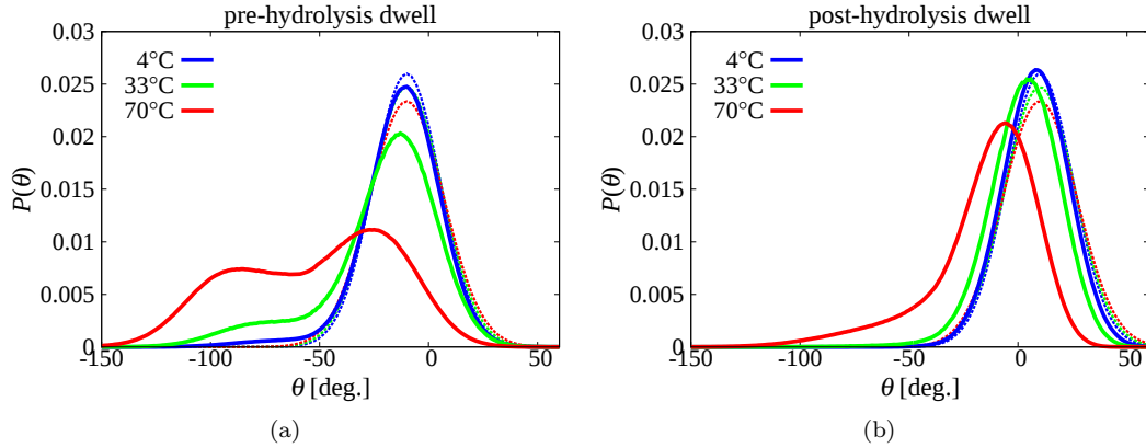
Fig.3.2: The steady state angle distribution at 4, 33, 70 ^{\circ}\text{C} .
