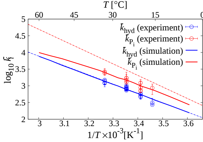
Fig.3.1: The Arrhenius plot of the rate coefficients of hydrolysis (blue) and \text{P}_i release (red).
