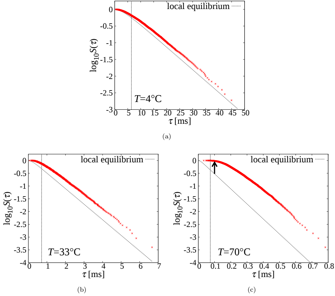
Fig.3.12: The dwell time survival distributions at 4, 33, 70°C obtained by simulation (red). The grey broken lines show double exponential functions assuming fast diffusion limit \bar{k}_{\text{hyd}/\text{P}_i}^{\text{FDL}} , i.e., the steady-state angle distributions equal to the Boltzmann distributions.
