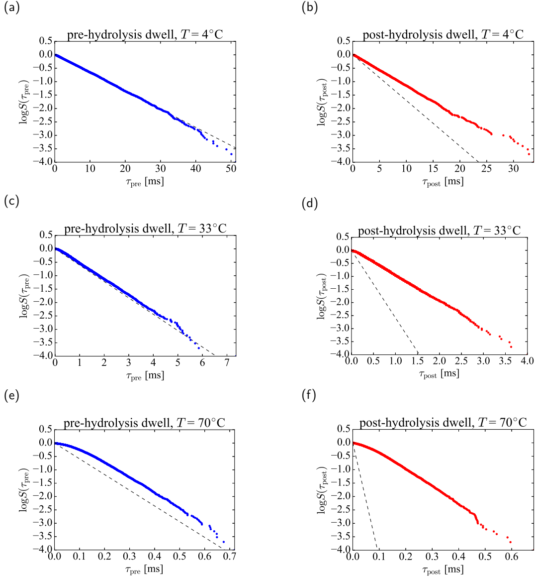
Fig.3.11: The survival distributions of sub-dwell time; pre-hydrolysis dwell time (left column) and post-hydrolysis dwell time (right column) at T = 4^\circ\text{C} (first row), 33^\circ\text{C} (second row), and 70^\circ\text{C} (third row). The broken lines show the single exponential functions with fast diffusion limit rate constants \bar{k}_i^{\text{FDL}} .
