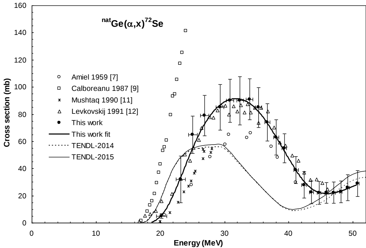
Figure 2. Experimental cross section data for the ^{\text{nat}}\text{Ge}(\alpha, x)^{72}\text{Se} reaction in comparison with the earlier measured data and the results of theoretical calculations. The thick solid line is a spline fit over the experimental points measured in this work.
