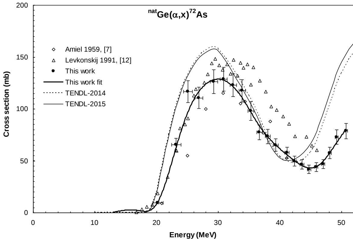
Figure 6 Experimental cross section data for the ^{\text{nat}}\text{Ge}(\alpha, x)^{72}\text{As} reaction in comparison with the earlier measured data and the result of the theoretical calculations. The thick solid line is a spline fit over the experimental points measured in this work.
