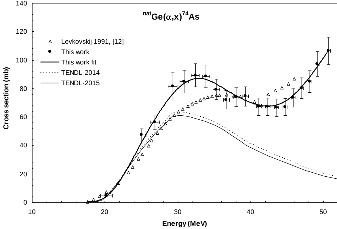
Figure 7. Experimental cross section data for the ^{\text{nat}}\text{Ge}(\alpha, x)^{74}\text{As} reaction in comparison with the earlier measured data and the result of the theoretical calculations. The thick solid line is a spline fit over the experimental points measured in this work.
