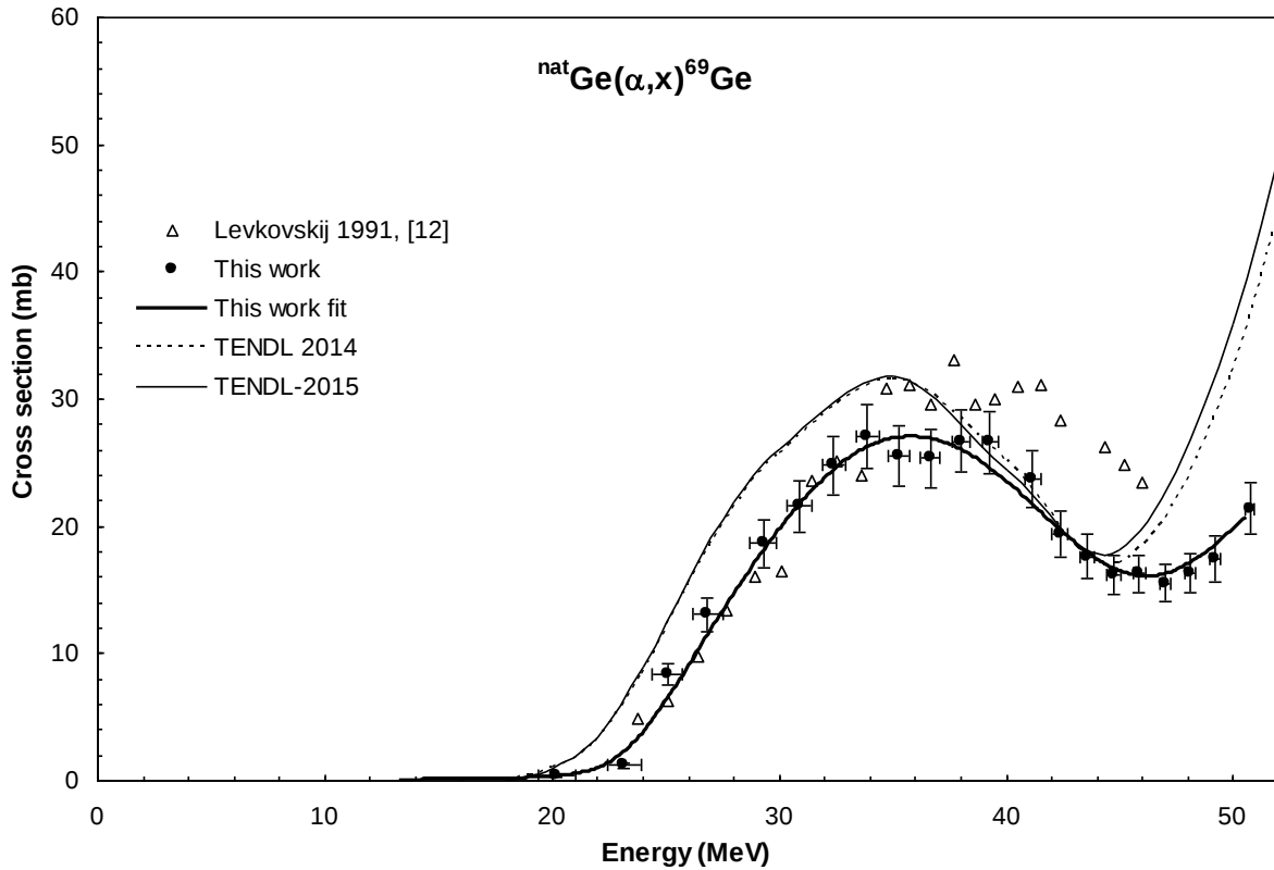
Figure 10. Experimental cross section data for the ^{nat}\text{Ge}(\alpha,x)^{69}\text{Ge} reaction in comparison with the earlier measured data and the result of the theoretical calculations. The thick solid line is a spline fit over the experimental points measured in this work.
