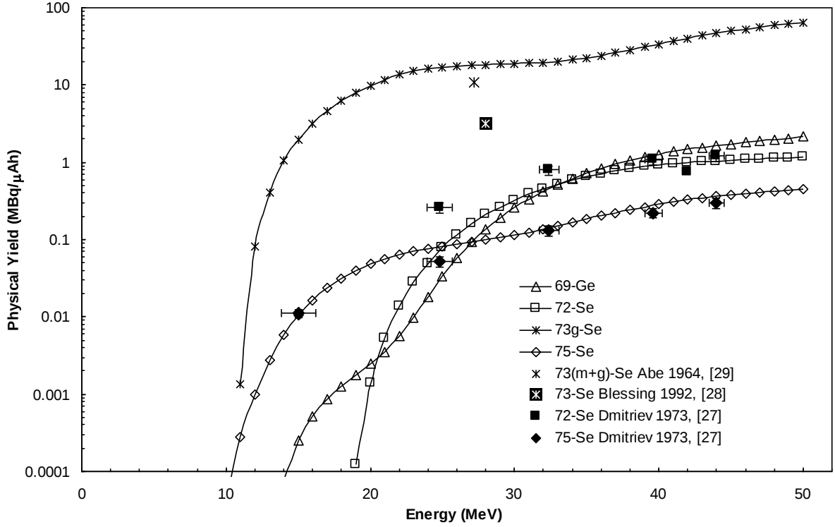
Figure 11. Calculated physical thick target yields for production of ^{72,73,75}\text{Se} and ^{69}\text{Ge} based on the newly measured cross section data in comparison with the available experimental yield data.
