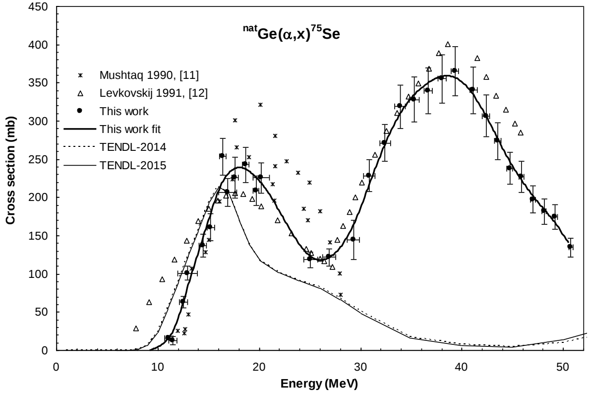
Figure 4 Experimental cross section data for the {}^{\text{nat}}\text{Ge}(\alpha, x){}^{75}\text{Se} reaction in comparison with the earlier measured data and the result of the theoretical calculations. The thick solid line is a spline fit over the experimental points measured in this work.
