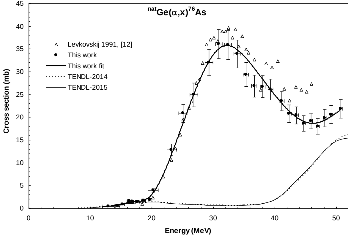
Figure 8. Experimental cross section data for the ^{nat}\text{Ge}(\alpha,x)^{76}\text{As} reaction in comparison with the earlier measured data and the result of the theoretical calculations. The thick solid line is a spline fit over the experimental points measured in this work.
