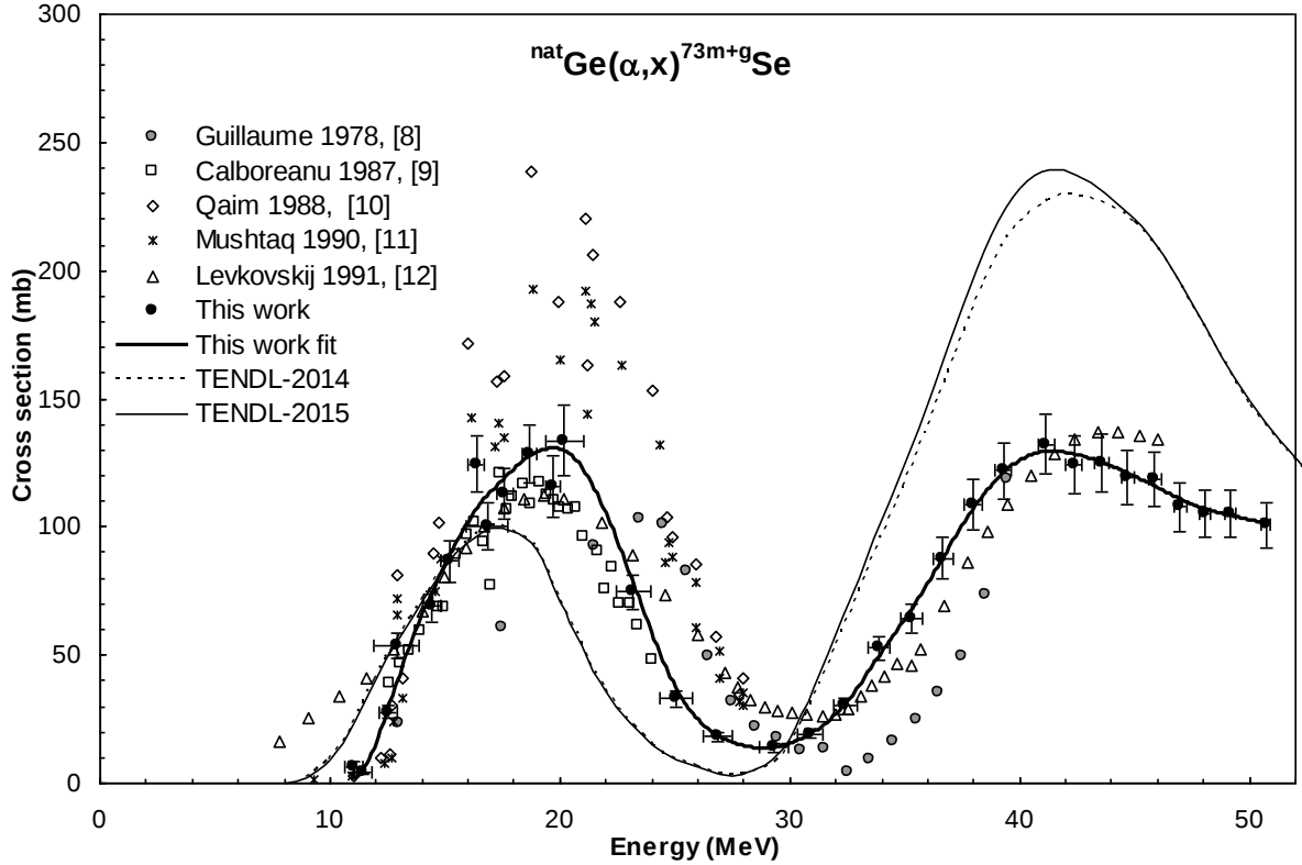
Figure 3. Experimental cross section data for the ^{nat}\text{Ge}(\alpha, x)^{73m+g}\text{Se} reaction in comparison with the available literature data and the result of the theoretical calculations. The thick solid line is a spline fit over the experimental points measured in this work.
