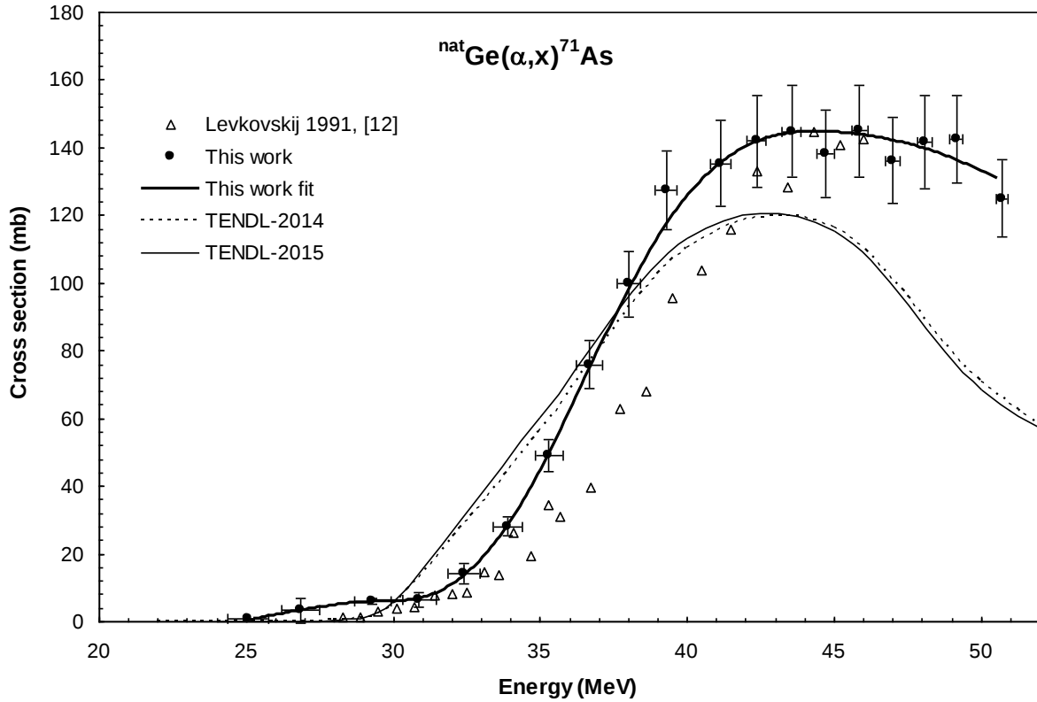
Figure 5. Experimental cross section data for the ^{\text{nat}}\text{Ge}(\alpha, x)^{71}\text{As} reaction in comparison with the earlier measured data and the result of the theoretical calculations. The thick solid line is a spline fit over the experimental points measured in this work.
