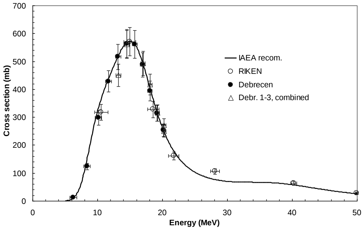
Figure 1. Comparison of the recommended excitation function of the ^{nat}\text{Ti}(\alpha, x)^{51}\text{Cr} reaction [21] and the experimental cross section data points deduced in these experiments. The open circle represents the experiment in RIKEN, the full dot represents the stack in Atomki containing only Ti foils, and the open triangle represents the combined three experiments in Atomki with Ge targets.
