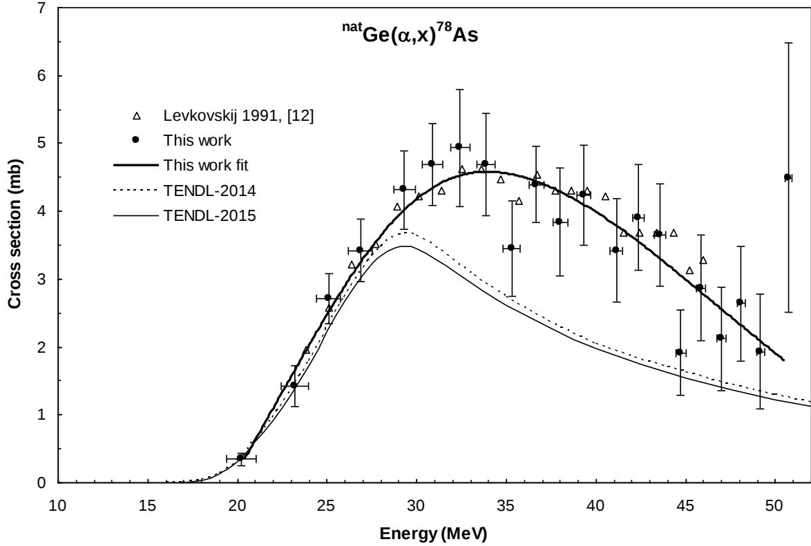
Figure 9 Experimental cross section data for the {}^{\text{nat}}\text{Ge}(\alpha, x){}^{78}\text{As} reaction in comparison with the earlier measured data and the result of the theoretical calculations. The thick solid line is a spline fit over the experimental points measured in this work.
