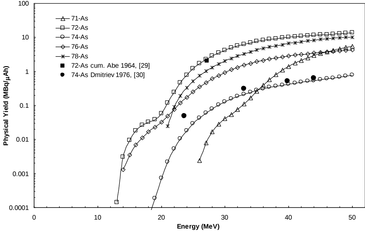
Figure 12. Calculated physical thick target yields for production of ^{71,72,74,76,78}\text{As} based on the newly measured cross section data in comparison with the available experimental yield data.
