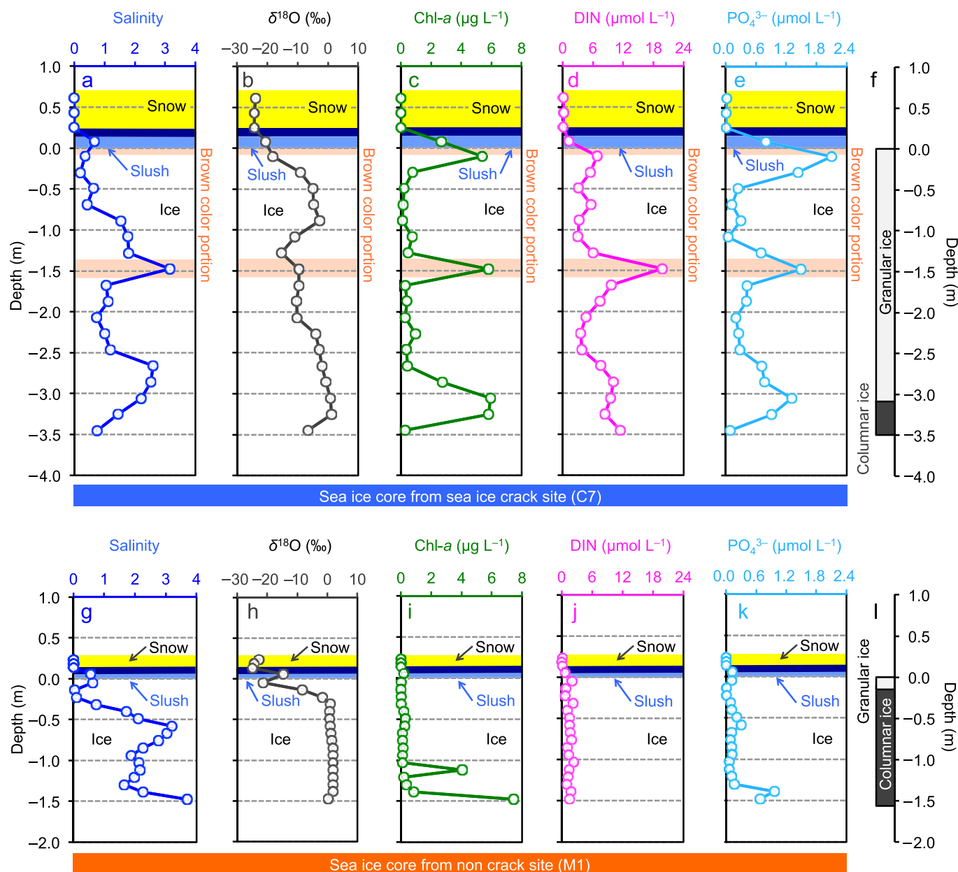
Figure 6. Depth profiles of (a, g) salinity, (b, h) \delta^{18}\text{O} , (c, i) chl a concentration, (d, j) DIN concentration, (e, k) \text{PO}_4^{3-} concentration, and (f, l) sea ice structure at (a–f) C7 and (g–l) M1. The yellow, blue, light blue, and brown shading (Figures 6a–6e and 6g–6k) indicate the snow, superimposed ice, slush, and discoloration (brown) portions of the sea ice, respectively.
