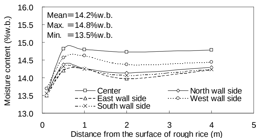
Figure 7 - Moisture content distribution of rough rice stored in the silo at the end of storage.
