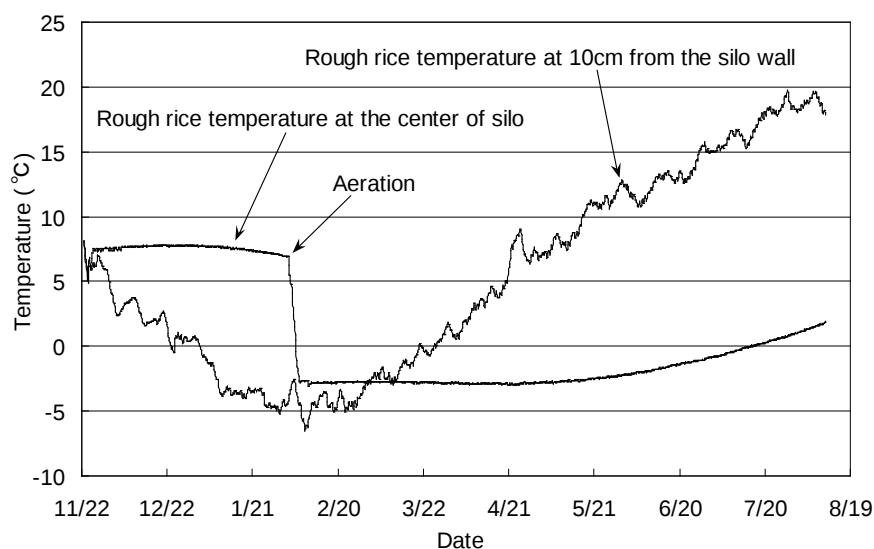
Figure 5 - Rough rice temperature during on-farm storage.
