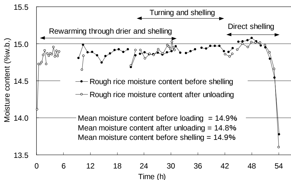
Figure 10 - Moisture content of rough rice during unloading and rewarming.
