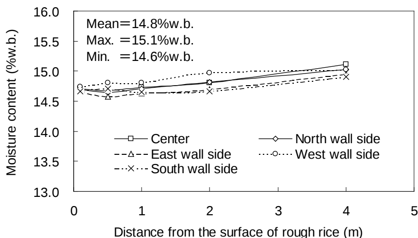
Figure 6 - Moisture content distribution of rough rice stored in the silo at the beginning of storage.
