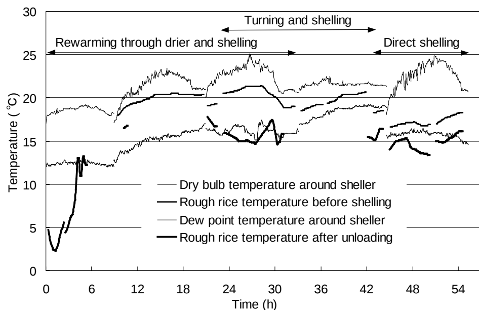
Figure 9 - Temperature of grain and temperature around sheller during unloading, rewarming and shelling.
