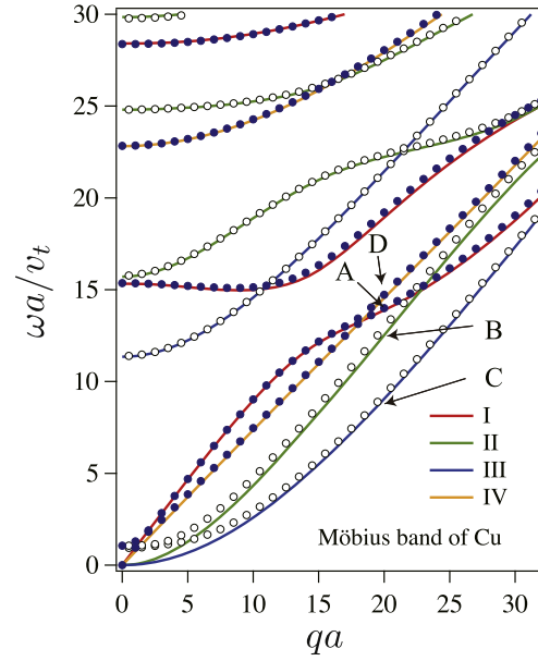
Figure 2. Phonon frequencies versus wave number of a copper Möbius band with cross sectional dimensions (2w/a) \times (2h/a) = 0.1 \times 0.2 . The solid circles and open circles indicate phonon spectra at wave number q of an integer and half-integer multiple of 1/a , respectively. The solid lines are the dispersion relations of phonon modes in a rectangular wire of copper with the same cross section area as Möbius band. Four different kinds of modes referred to as I, II, III and IV are distinguished by colors. Vibrational patterns at four points labelled A, B, C, and D are examined below. The used material parameters are \rho = 8.94 \text{ g/cm}^3 , C_{11} = 168.4 \text{ GPa} , C_{12} = 121.4 \text{ GPa} , C_{44} = 75.4 \text{ GPa} [1].
