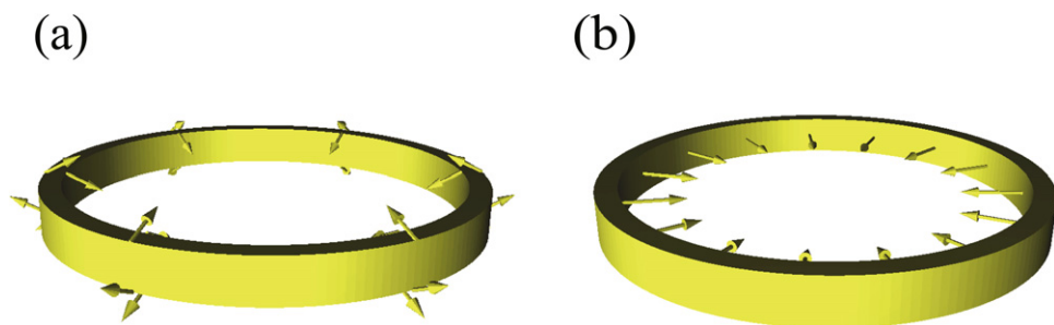
Figure 8. Vibrational patterns of modes in a ring at (a) and (b) denoted in figure 5. The arrows indicate the directions of displacement vectors, showing (a) a uniform torsional motion and (b) a breathing motion.
