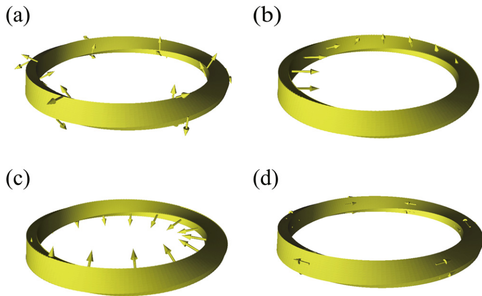
Figure 7. Vibrational patterns at (a)–(d) denoted in figures 3 and 4. The arrows indicate the directions of displacement vectors. Modes (b) and (c) have a period of 4\pi a .
