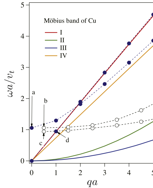
Figure 3. Phonon spectra of a copper Möbius band in the low frequency region near the zone center of figure 2. Points labelled a, b, c and d indicate characteristic frequencies of Möbius band. See the text.
