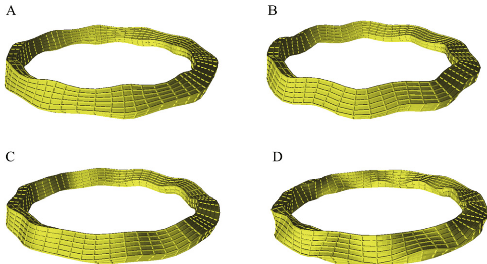
Figure 6. Vibrational patterns at A, B, C and D denoted in figure 2. The wavelengths of A and D are \lambda = 2\pi a/10 and those of B and C are \lambda = 2\pi a/9.5 . For vibrational pattern B (C), the displacement occurs primarily in the direction of the longer (shorter) edge of the cross section. Compared with B, C can be considered to be more like the flexural vibrations of a thin-plate, therefore having a vibration frequency lower than that of B.
