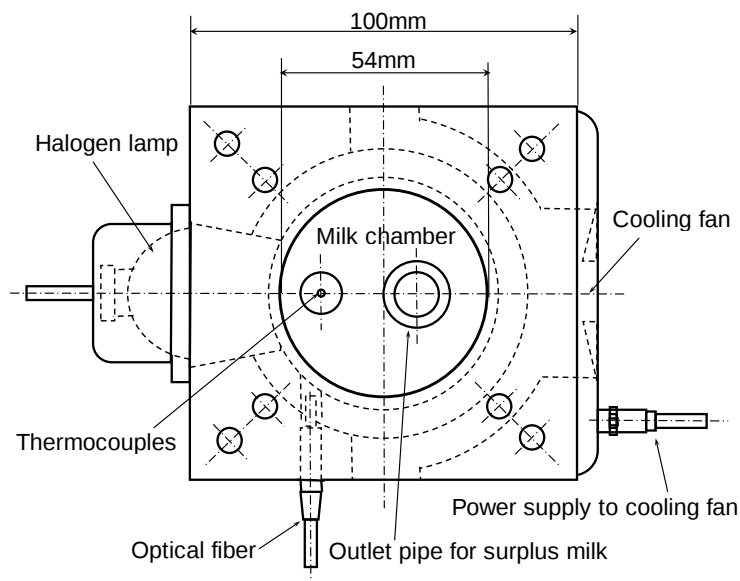
Figure 3. Plane view of the near-infrared spectrum sensor constructed on an experimental basis.
