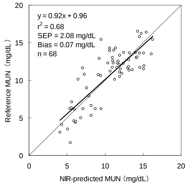
Figure 9. Correlation between reference MUN and NIR-predicted MUN.
