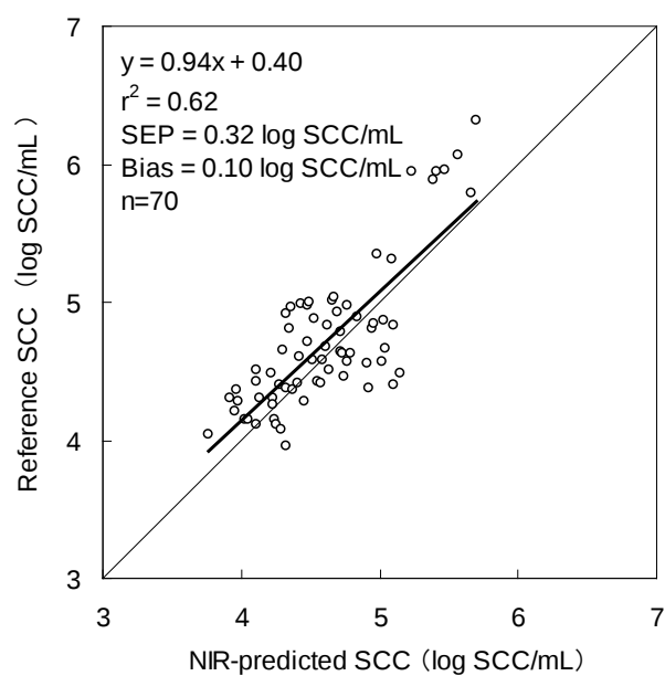
Figure 8. Correlation between reference SCC and NIR-predicted SCC.
