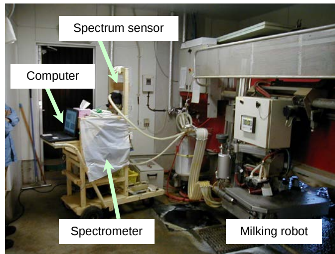
Figure 2. On-line near-infrared spectroscopic sensing system installed in an automatic milking system.
