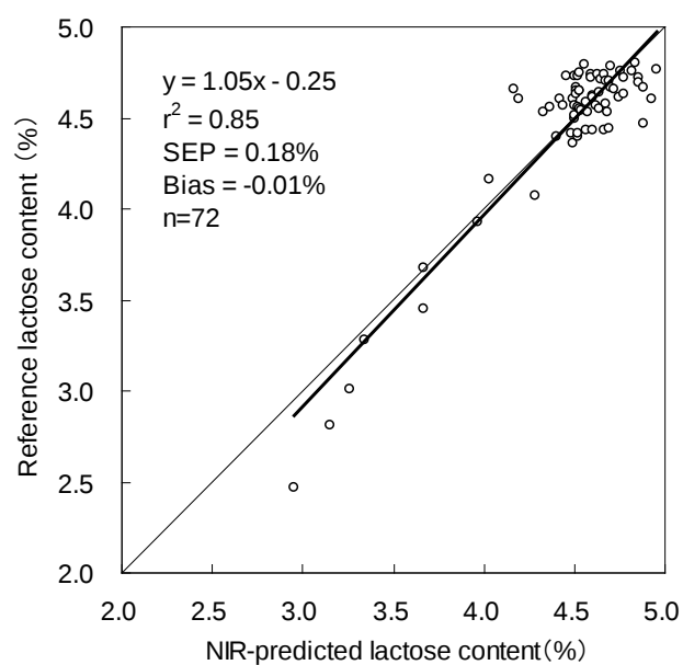
Figure 7. Correlation between reference lactose content and NIR-predicted lactose content.
