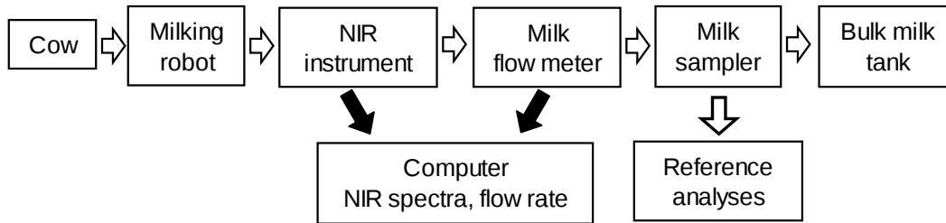
Figure 1. Flow chart of an on-line near-infrared spectroscopic sensing system for assessing milk quality in an automatic milking system.
