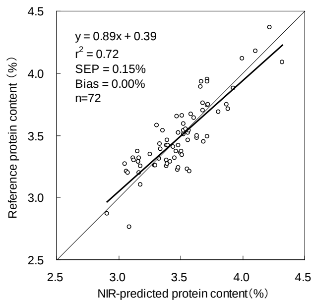
Figure 6. Correlation between reference protein content and NIR-predicted protein content.
