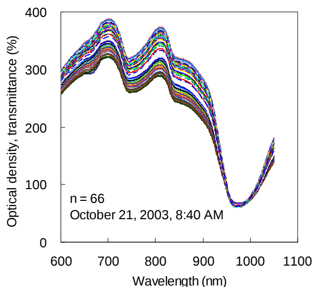
Figure 4. Original spectra of unhomogenized milk from cow number 304 during milking on October 21, 2003.
