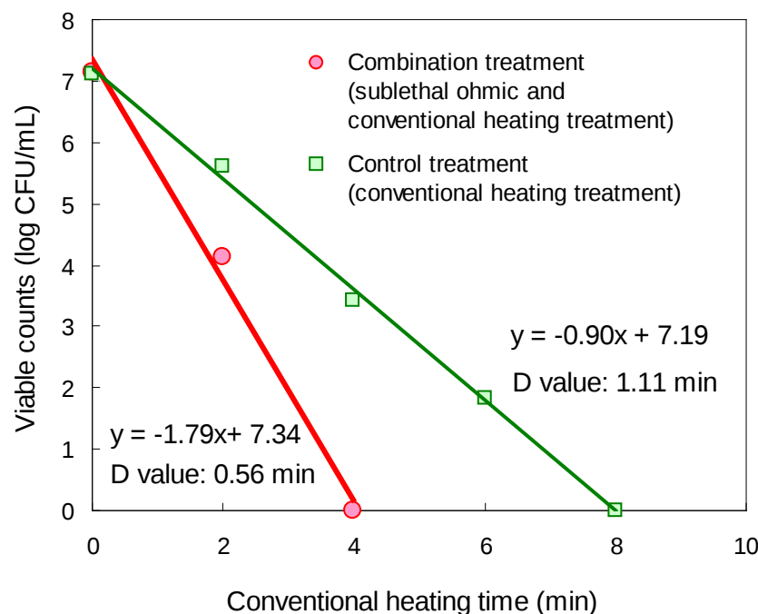
Figure 7. Regression line of heating time and Streptococcus thermophilus counts.
