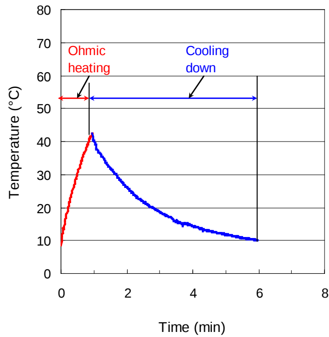
Figure 4. Heating and cooling history during sublethal ohmic heating.
