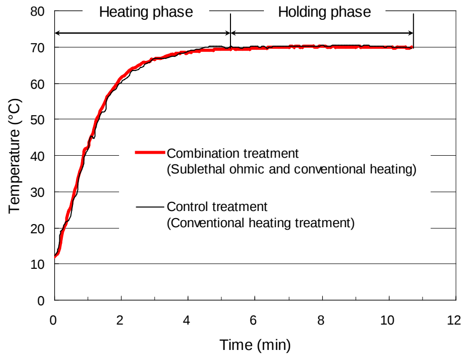
Figure 5. Comparison of temperature histories during conventional heating for combination and control treatments.
