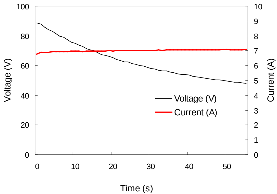
Figure 3. Voltage and current histories during sublethal ohmic heating.
