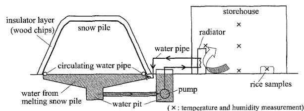
Fig. 3. Schematic diagram of the snow cooling system.
