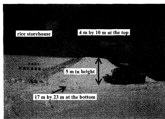
Fig. 1. Snow pile made next to the storehouse.
