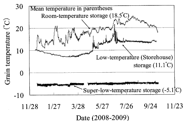
Fig. 6. Rice grain temperatures during storage for 10 months.
