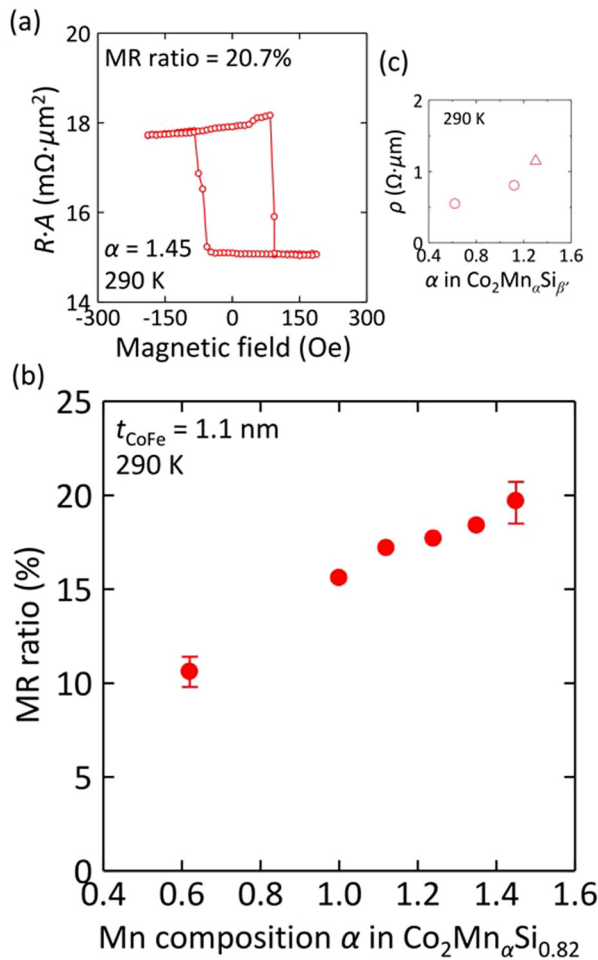
FIG. 2. (a) Typical MR curve at 290 K for a series-B spin valve [CMS/CoFe (1.1 nm)/Ag/CoFe (1.1)/CMS] with Mn-rich ( \alpha = 1.45 ) CMS electrodes and (b) MR ratio of series-B spin valves at 290 K as a function of Mn composition, \alpha , in \text{Co}_2\text{Mn}_x\text{Si}_{0.82} electrodes ranging from \alpha = 0.62 to 1.45. (c) Mn-composition dependence of the resistivity, \rho , of off-stoichiometric \text{Co}_2\text{MnSi} thin films at 290 K in \text{Co}_2\text{Mn}_x\text{Si}_{\beta'} ( \beta' = 0.82 or 0.90). The \rho values of two samples with \alpha = 0.62 and 1.12 in \text{Co}_2\text{Mn}_x\text{Si}_{0.82} (open circles), and a sample with \alpha = 1.30 in \text{Co}_2\text{Mn}_x\text{Si}_{0.90} (open triangle) are shown, where \alpha + \beta' < 2 and \alpha + \beta' > 2 in \text{Co}_2\text{Mn}_x\text{Si}_{\beta'} correspond to (Mn + Si)-deficient and (Mn + Si)-rich compositions, respectively.
