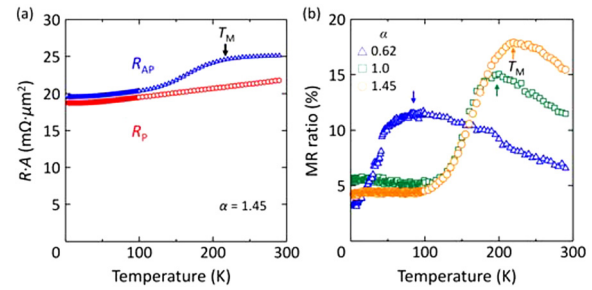
FIG. 3. (a) Temperature dependence of R_{AP} and R_P for a series-B spin valve [CMS/CoFe (1.1 nm)/Ag/CoFe (1.1)/CMS] with Mn-rich ( \alpha = 1.45 ) CMS electrodes and (b) T dependence of the measured MR ratio, defined as (R_{AP} - R_P)/R_P , in which the influence of R_c is not corrected, for series-B spin valves with \alpha = 0.62 , 1.0, and 1.45.
