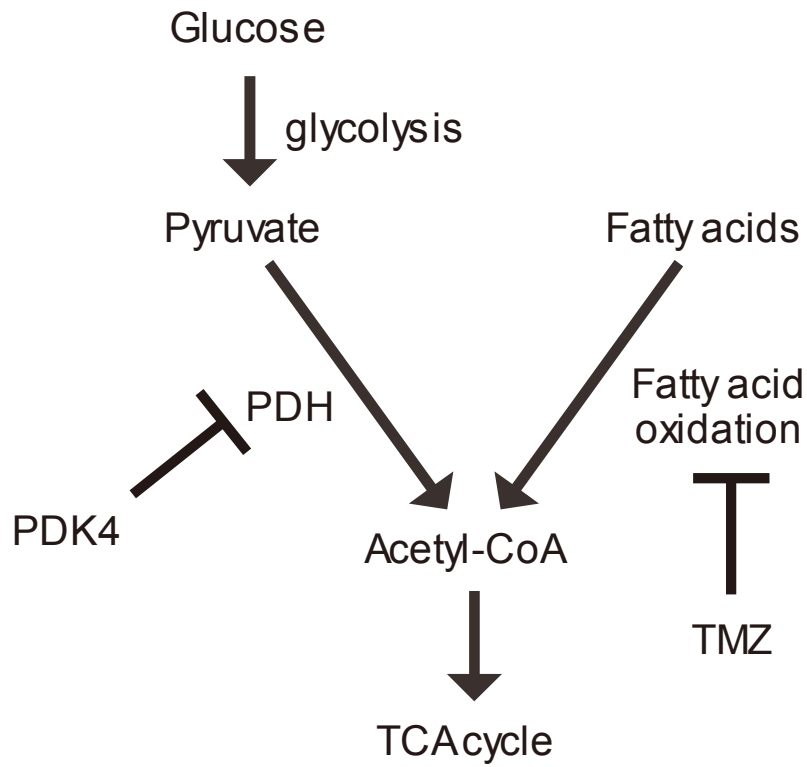
Figure 3.3. Schematic diagram for glycolysis and fatty acid oxidation.
