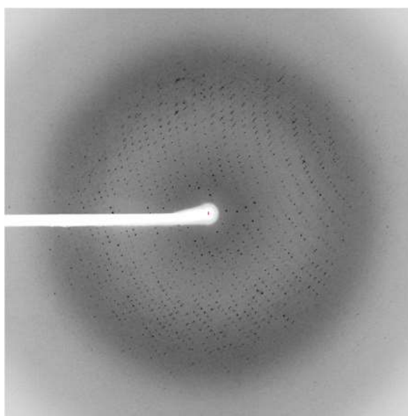
Figure 4.16 X-ray diffraction pattern from IRP1 C437S/C503S crystal.
