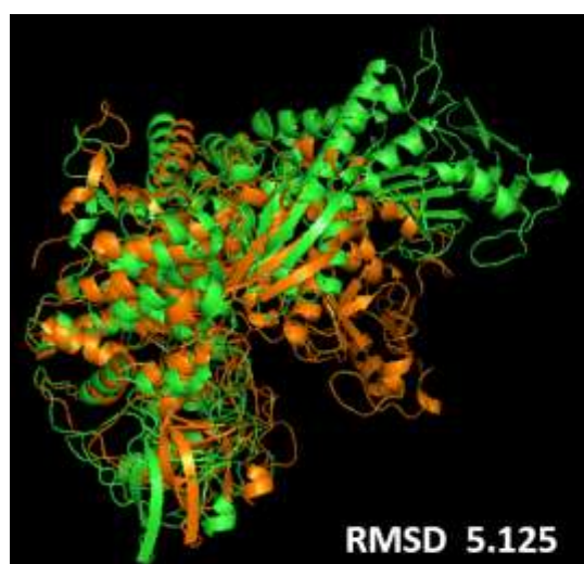
HEME - mRNA
