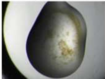
Figure 4.13 Crystals of IRP1 at initial screening.
