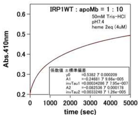
Figure 3.5 Time course of the displacement of heme from heme-IRP1 to apo-myoglobin.
