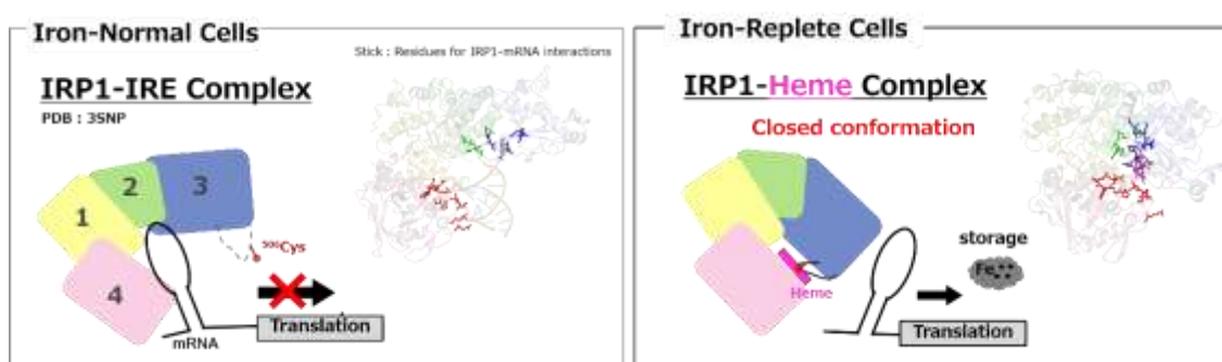
Figure 4.25. The novel mechanism of regulatory processes controlling IRP1 by heme.
