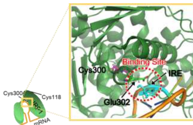
Figure 4.23 The location of HRM on the crystal structure of the IRP1-IRE complex (PDB: 3SNP).
