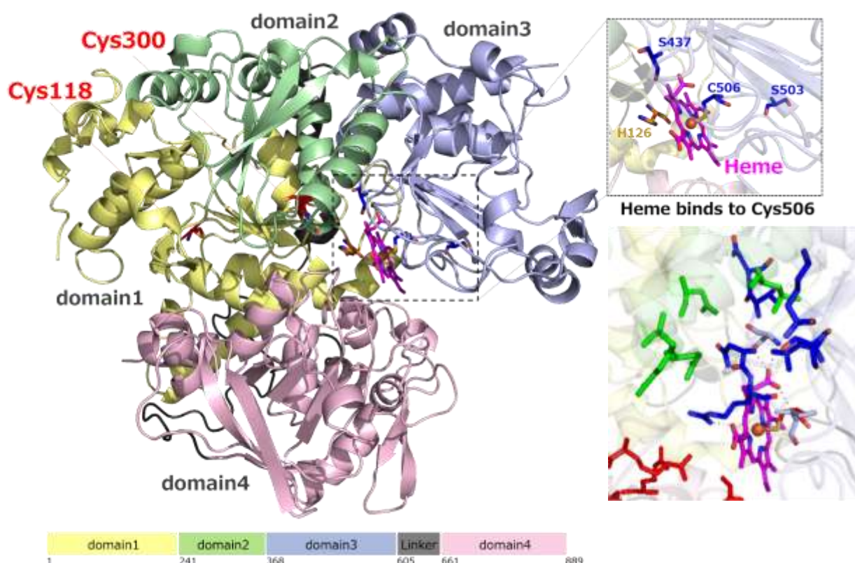
Figure 4.17 The determined X-ray structure of IRP1 with heme.
