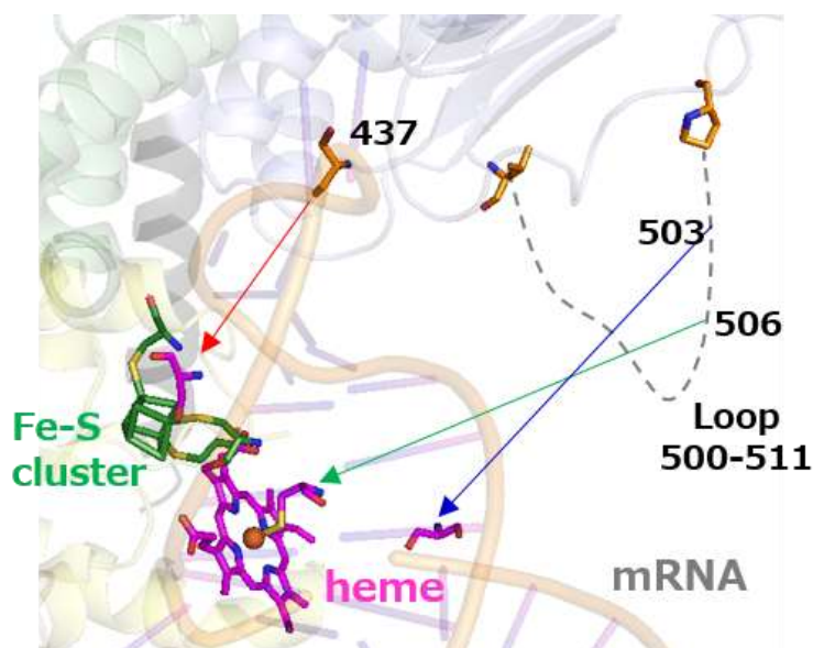
Figure 4.24. Superposition of the models of three IRP1 crystal forms.
