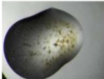
Flag-IRP1 C437S/C503S 12.7 mg/mL heme 2.4eq
