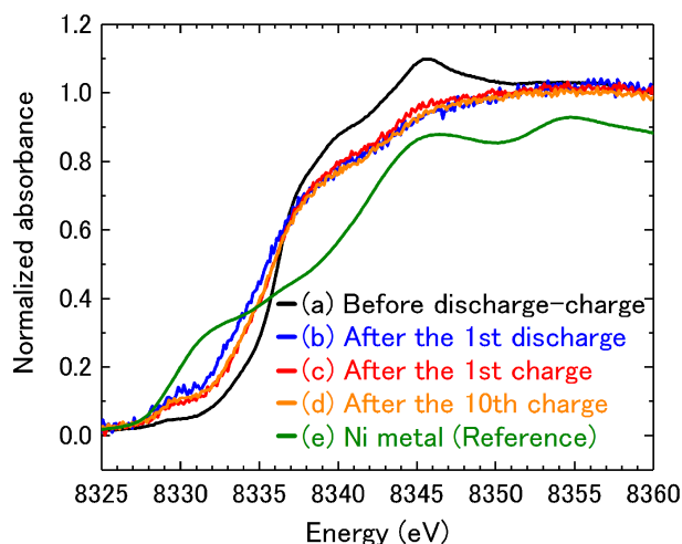
Fig. 5. Ni K-edge XANES spectra of (a) as-prepared NiPS 3 , and the working electrodes (b) after the 1st discharge, (c) after the 1st charge and (d) after the 10th charge. (e) The spectrum of Ni metal is also shown as a reference.
