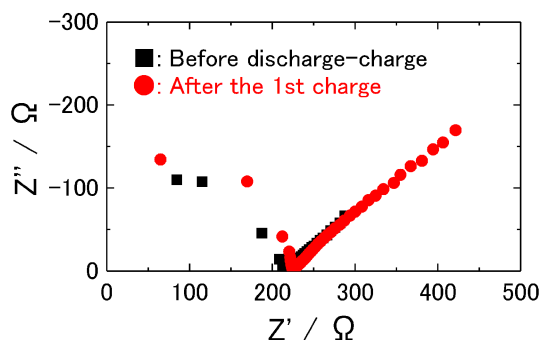
Fig. 3. Impedance profiles of Li-In/80 \text{Li}_2\text{S} ·20 \text{P}_2\text{S}_5 /NiPS 3 cells before and after the 1st discharge-charge.
