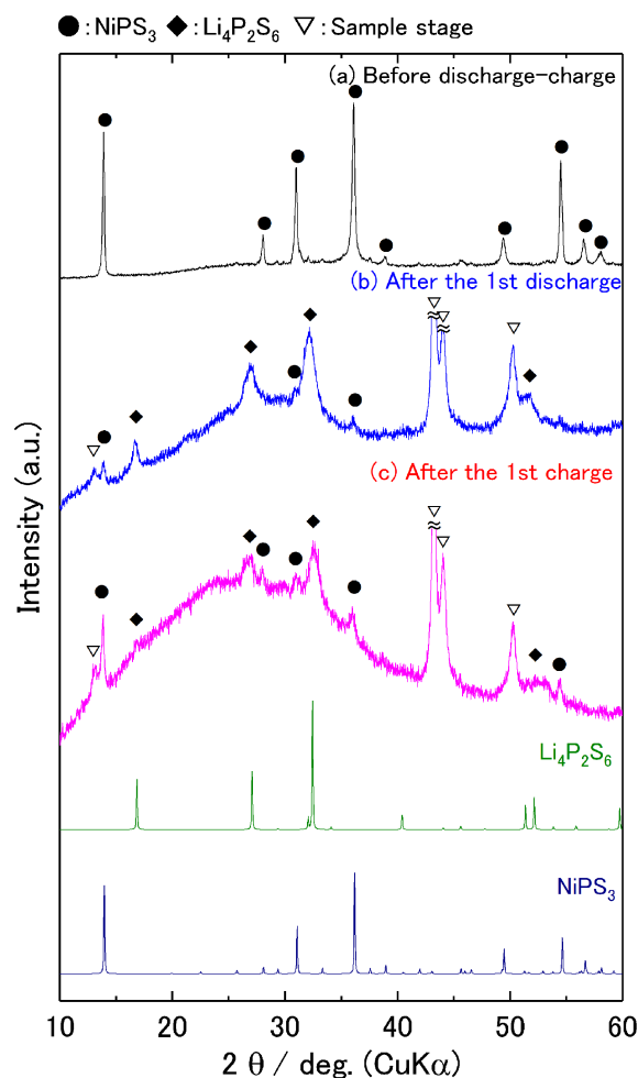
Fig. 4. XRD patterns of (a) as-prepared NiPS 3 , and the working electrodes (b) after the 1st discharge and (c) after the 1st charge. The simulated diffraction patterns of \text{Li}_4\text{P}_2\text{S}_6 (ICSD #33506) and NiPS 3 (ICSD #646133) were also shown as references.
