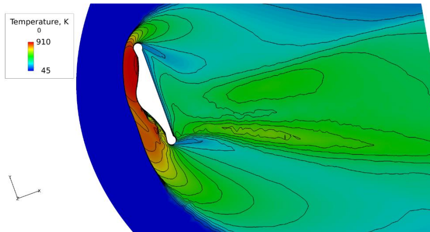
Figure 13. Gas temperature distribution around HWT-MAAC at AOA of 20 degree.
