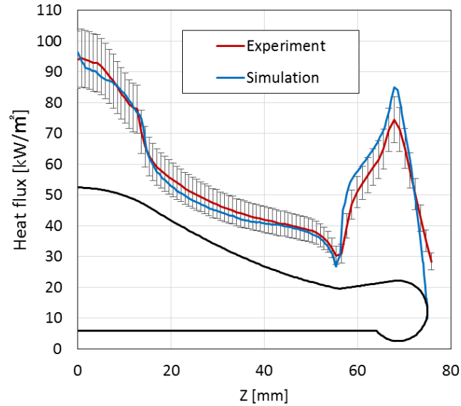
Figure 16. Comparison of heat flux on front surface of HWT-MAAC at AOA of 0 degree between experiment and numerical analysis.
