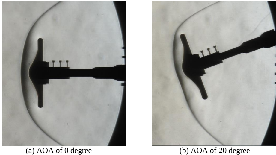
Figure 2. Density gradient distribution around HWT-MAAC by Schlieren photograph technique for case1 and case3
