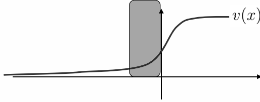
FIGURE 3. An image of v showing blocking of a front
