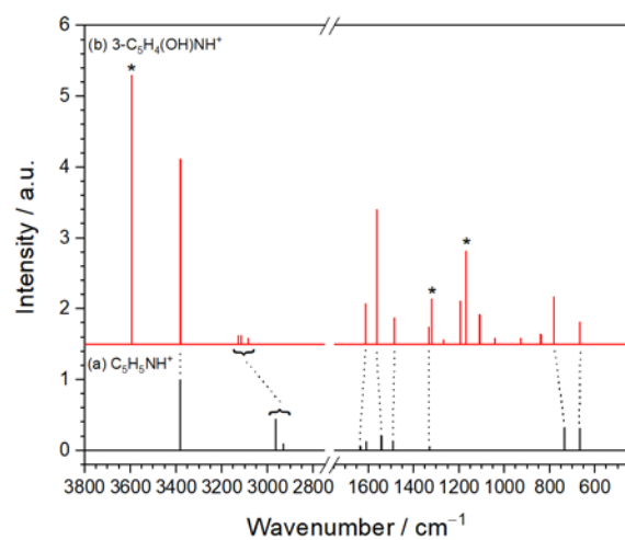
FIG. 6. Comparison of stick spectra of lines of (a) protonated pyridine, \text{C}_5\text{H}_5\text{NH}^+ , and (b) protonated 3-hydroxy-pyridine, trans -3-hydroxy-(1H)-pyridinium cation. The additional lines associated with vibrations of the OH moiety are indicated with *. The dotted lines connect similar vibrational modes.
