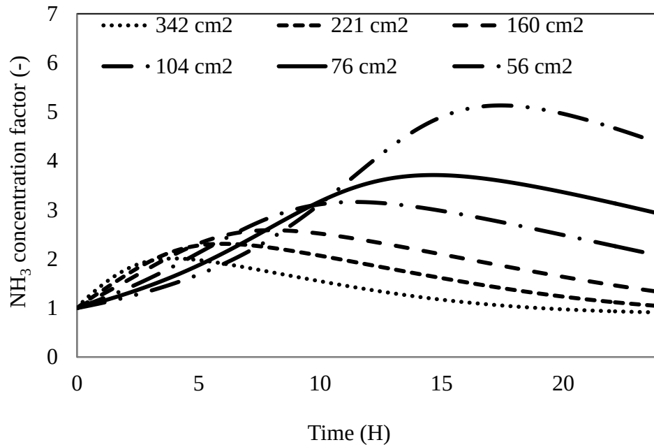
Figure 6 Time course of \text{NH}_3 concentration factor calculated with variable membrane areas (342 - 56 \text{cm}^2 )
