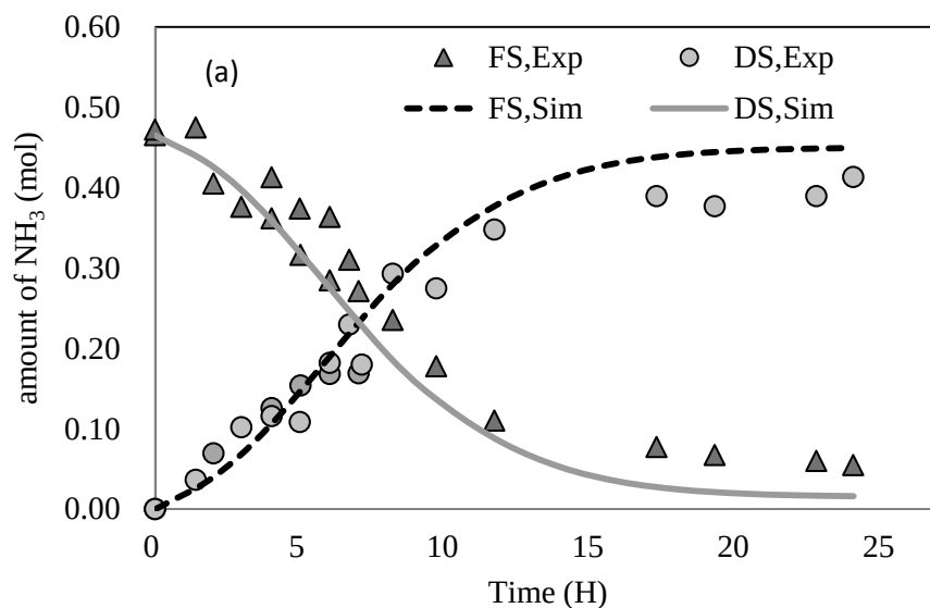
Figure 8 (a) Time course of \text{NH}_3 amount during synthetic hydrolyzed urine concentration with 5 mol/L NaCl draw solution
