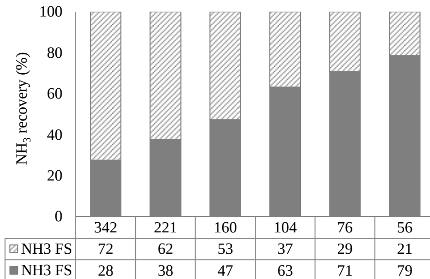
Figure 7 Recovery percentage of \text{NH}_3 corresponding to 1/5 volume reduction, case of variable membrane areas
