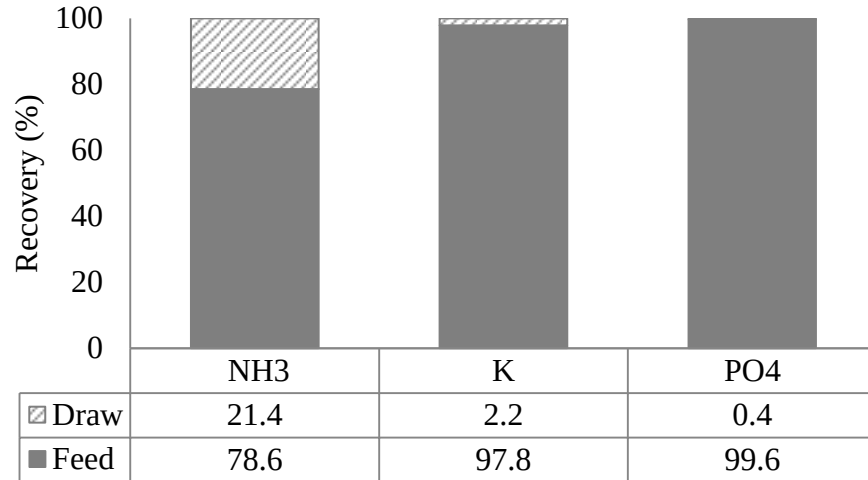
Figure 9 Recovery of \text{NH}_3 , K, \text{PO}_4 at 5 times urine volume reduction calculated with the proposed design parameters
