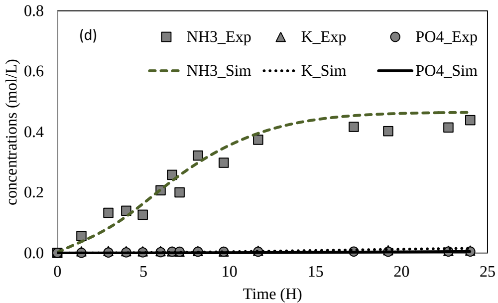
Figure 7 Validation of concentrations estimation: (c) time course of nutrients ( \text{NH}_3 , K, \text{PO}_4 ) concentrations in feed solution, (d) time course of nutrients ( \text{NH}_3 , K, \text{PO}_4 ) concentrations in draw solution.
