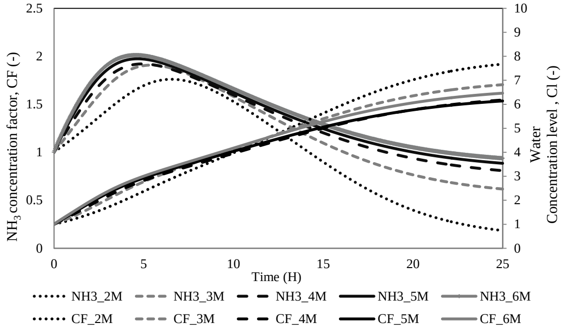
Figure 3 Time course of \text{NH}_3 concentration and the volume concentration level, case of 300 \text{ cm}^2 membrane area
