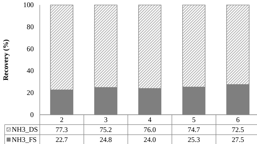
Figure 4 Recovery percentage of \text{NH}_3 corresponding to 1/5 volume reduction, case of 300 \text{ cm}^2 membrane area
