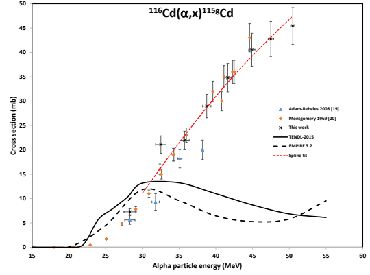
Figure 7: Excitation function of the ^{116}\text{Cd}(\alpha,x)^{115g}\text{Cd} nuclear reaction in comparison with the previous literature data and the results of the theoretical nuclear reaction model codes EMPIRE 3.2 and TALYS 1.8 (TENDL-2015)
