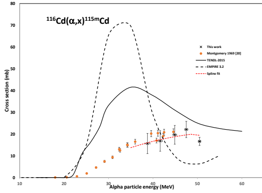
Figure 6: Excitation function of the ^{116}\text{Cd}(\alpha,x)^{115m}\text{Cd} nuclear reaction in comparison with the previous literature data and the results of the theoretical nuclear reaction model codes EMPIRE 3.2 and TALYS 1.8 (TENDL-2015)
