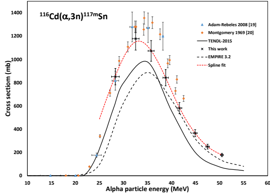
Figure 1: Excitation function of the ^{116}\text{Cd}(\alpha,3n)^{117m}\text{Sn} nuclear reaction in comparison with the previous literature data and the results of the theoretical nuclear reaction model codes EMPIRE 3.2 and TALYS 1.8 (TENDL-2015)
