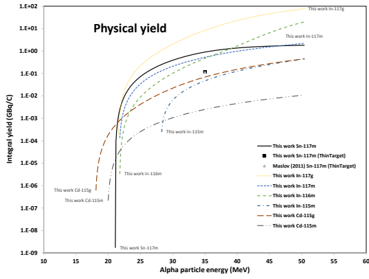
Figure 8: Thick target physical yields of the investigated radioisotopes. Thin target yield of Maslov et al. is also presented in this figure and compared with the thin target yield calculated from our results using the same input parameters (target thickness, energy window, enrichment)
