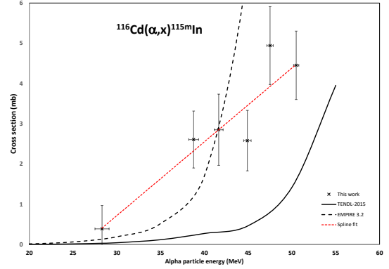
Figure 5: Excitation function of the ^{116}\text{Cd}(\alpha, x)^{115m}\text{In} nuclear reaction in comparison with the results of the theoretical nuclear reaction model codes EMPIRE 3.2 and TALYS 1.8 (TENDL-2015)
