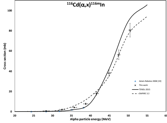
Figure 4: Excitation function of the ^{116}\text{Cd}(\alpha, x)^{116m}\text{In} nuclear reaction in comparison with the previous literature data and the results of the theoretical nuclear reaction model codes EMPIRE 3.2 and TALYS 1.8 (TENDL-2015)
