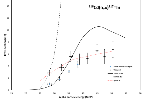
Figure 2: Excitation function of the ^{116}\text{Cd}(\alpha,x)^{117m}\text{In} nuclear reaction in comparison with the previous literature data and the results of the theoretical nuclear reaction model codes EMPIRE 3.2 and TALYS 1.8 (TENDL-2015)
