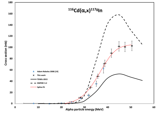
Figure 3: Excitation function of the ^{116}\text{Cd}(\alpha,x)^{117g}\text{In} nuclear reaction in comparison with the previous literature data and the results of the theoretical nuclear reaction model codes EMPIRE 3.2 and TALYS 1.8 (TENDL-2015)
