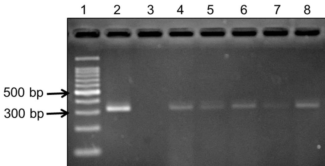
Figure 3. ITS1-PCR result.
