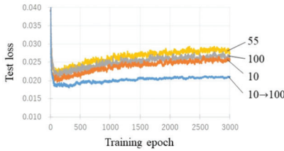
(a) First condition: N_1 = 10 , N_2 = 100 .
