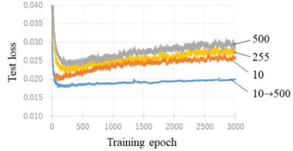
(b) Second condition: N_1 = 10 , N_2 = 500 .
