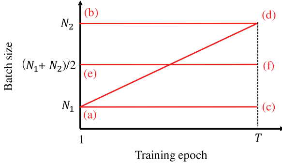
Figure 5: Batch size changing strategies. Four strategies were tested: (a)→(d), (a)→(c), (b)→(d), and (e)→(f).
