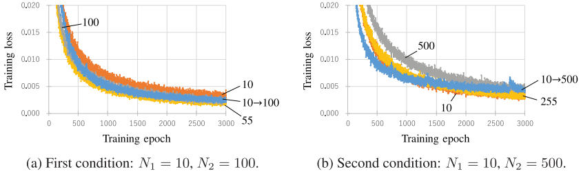
Figure 8: Effect of changing batch size on training loss.
