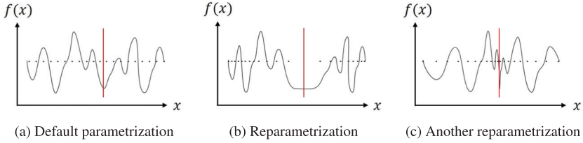
Figure 2: A one-dimensional example of how much geometry of loss function depends on parameter space chosen (based on Dinh et al., 2017). The x -axis represents parameter value, and the y -axis represents loss.
