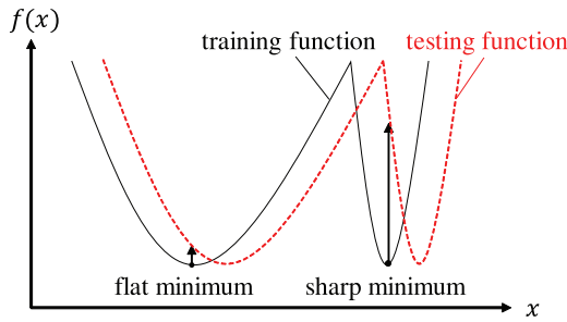
Figure 1: Conceptual sketch of flat and sharp minima (based on Keskar et al., 2017). The y -axis represents value of loss function, and the x -axis represents variables.
