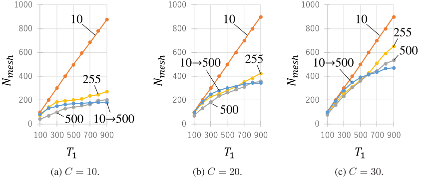
Figure 11: Comparison of the number of cells visited in the first part.
