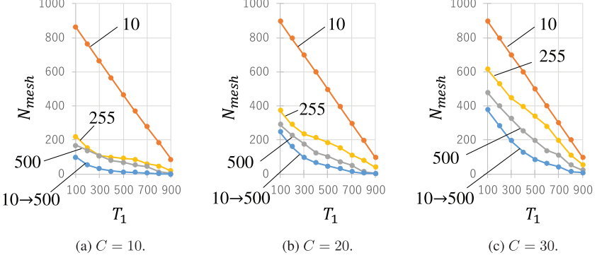
Figure 10: Comparison of the number of cells visited in the latter part.
