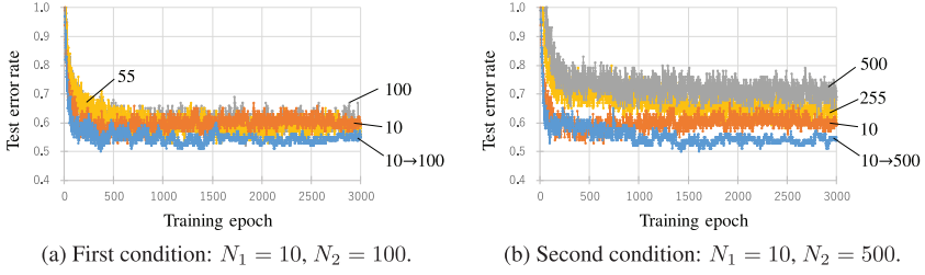
Figure 7: Effect of changing batch size on test error rate.
