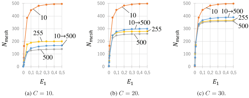
Figure 12: Comparison of the number of cells visited in the region E < E_1 before epoch T_1 = 500 .
