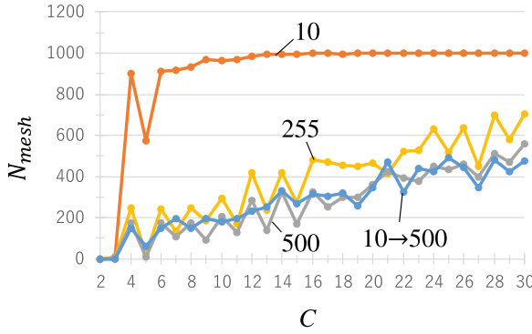
Figure 9: Comparison of the number of cells visited.
