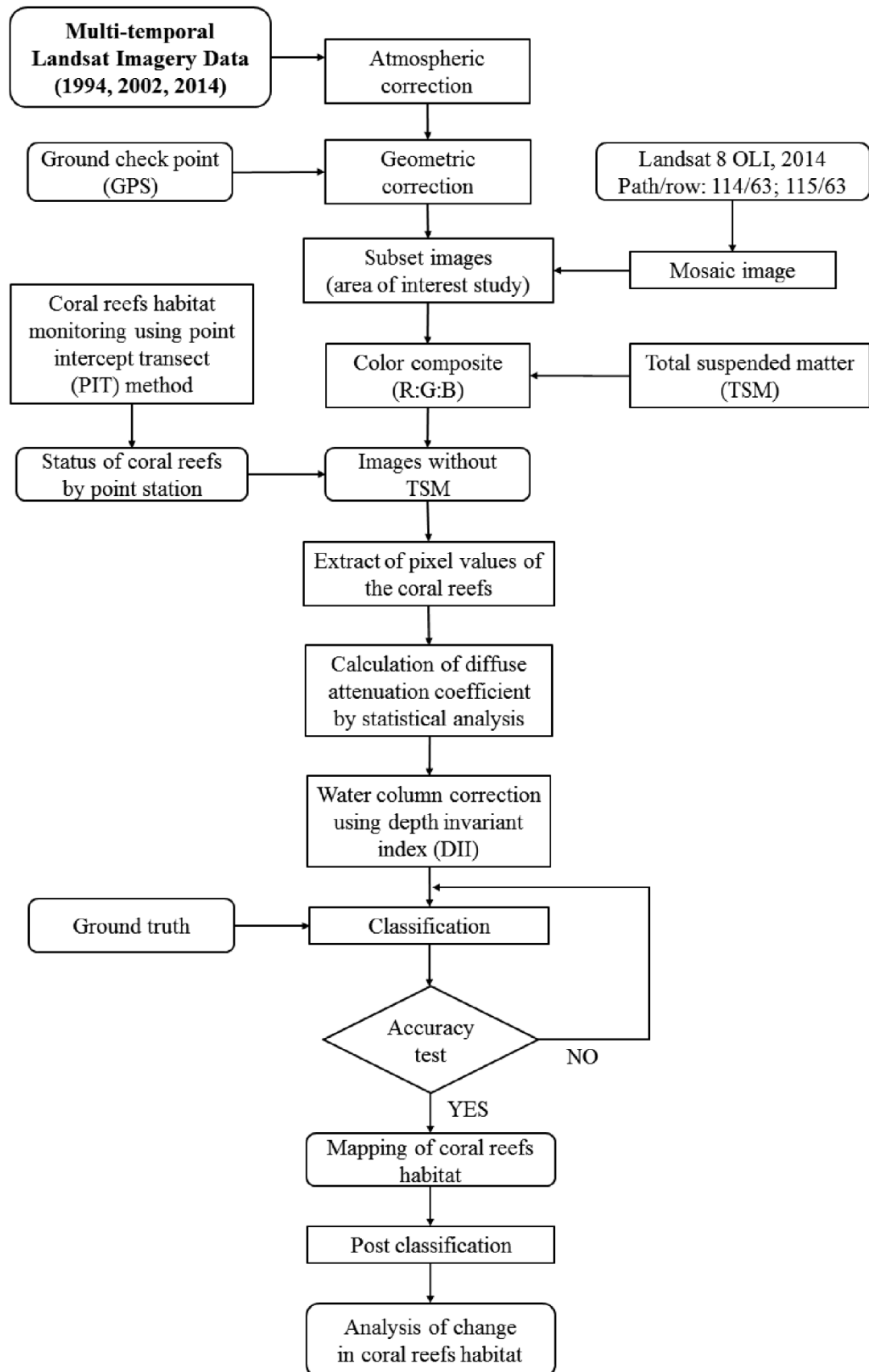
Fig. 3 Flowchart research on mapping and analysis of changes in coral reef habitat
