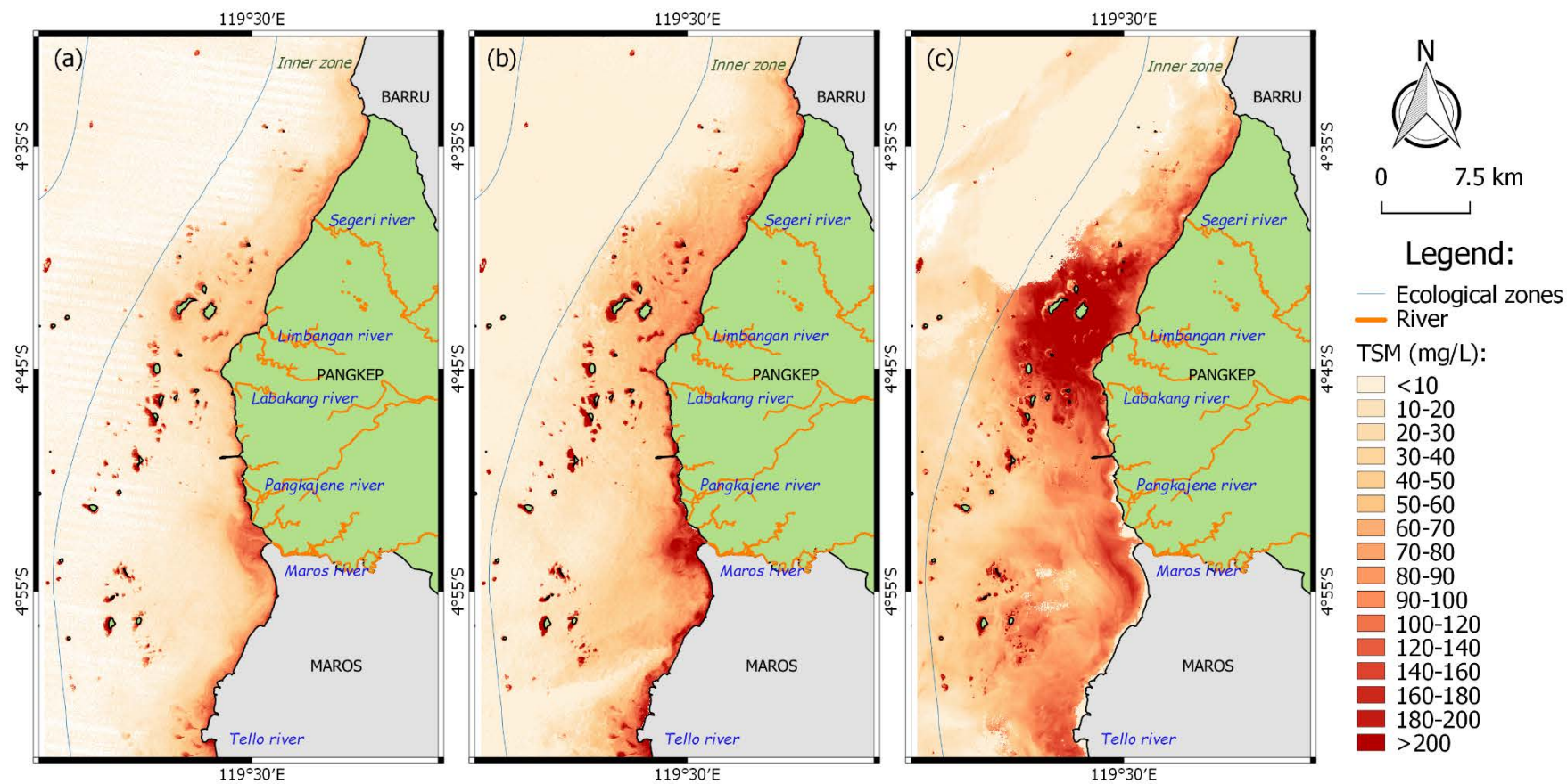
Fig. 8 Distribution and concentration of total suspended matter (TSM) in study area using (a) in Landsat 5 TM, 1994, (b) Landsat 7 ETM, 2002 and (c) Landsat 8 OLI, 2014
