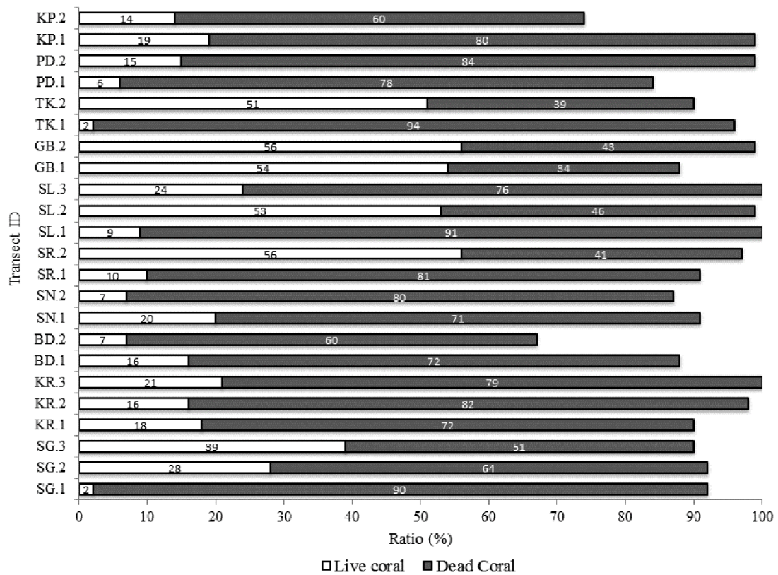
Fig. 4 Ratio of live corals and dead corals at all sites in the PANGKEP Regency, Spermonde Archipelago, Indonesia. The graph summarizes the calculation for each category obtained by PIT method in each village (2-3 observation transects per village)
