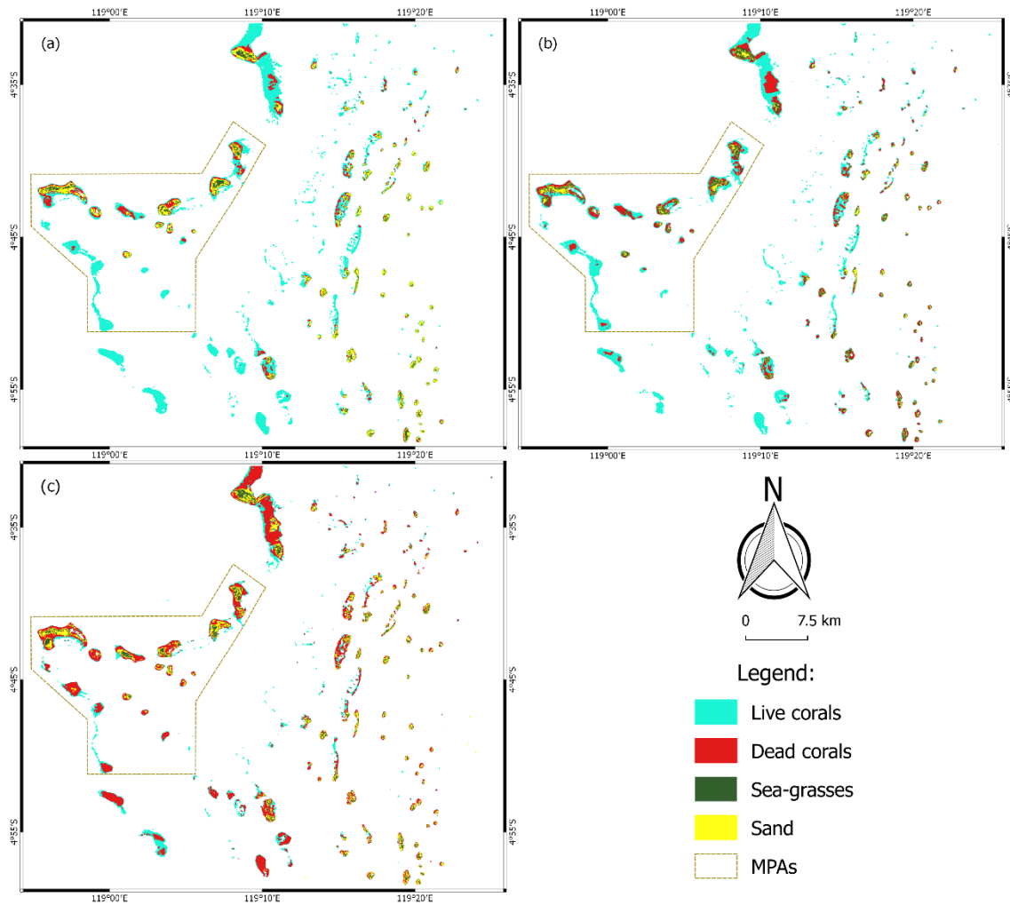
Fig. 11 Distribution and condition of coral reefs in the PANGKEP, Spermonde Archipelago, Indonesia, obtained from three series multi-temporal Landsat imagery data. (a) Landsat 5 TM, 1994; (b) Landsat 7 ETM, 2002; (c) Landsat 8 OLI, 2014
