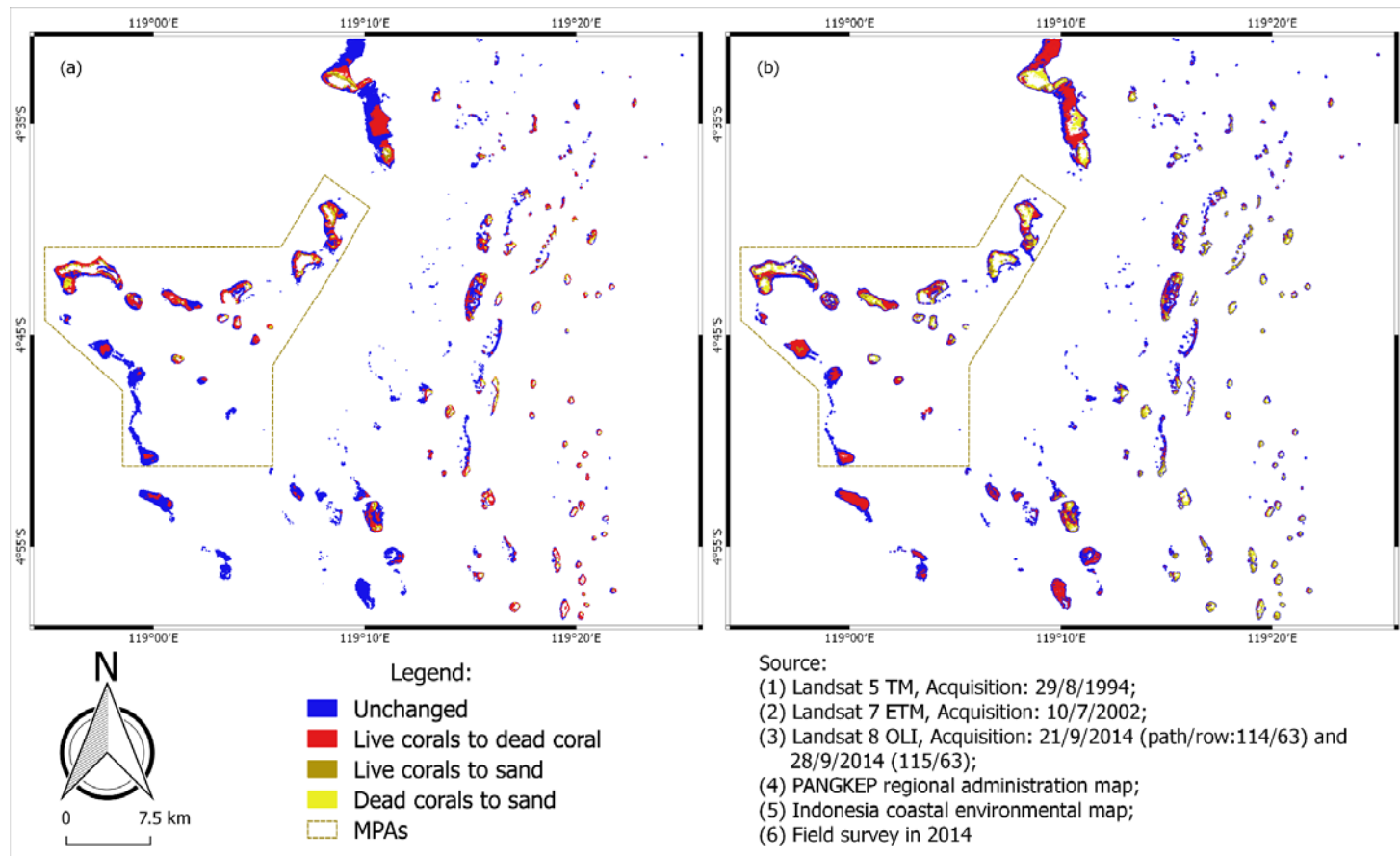
Fig. 12 Map of change in bottom substrate in the PANGKEP Regency, Spermonde Archipelago, Indonesia: (a) from 1994 to 2002 and (b) from 2002 to 2014. The Kapoposang MPAs is located in the outer zone of the PANGKEP islands which also experienced a drastic decline in coral reef habitats in this period
