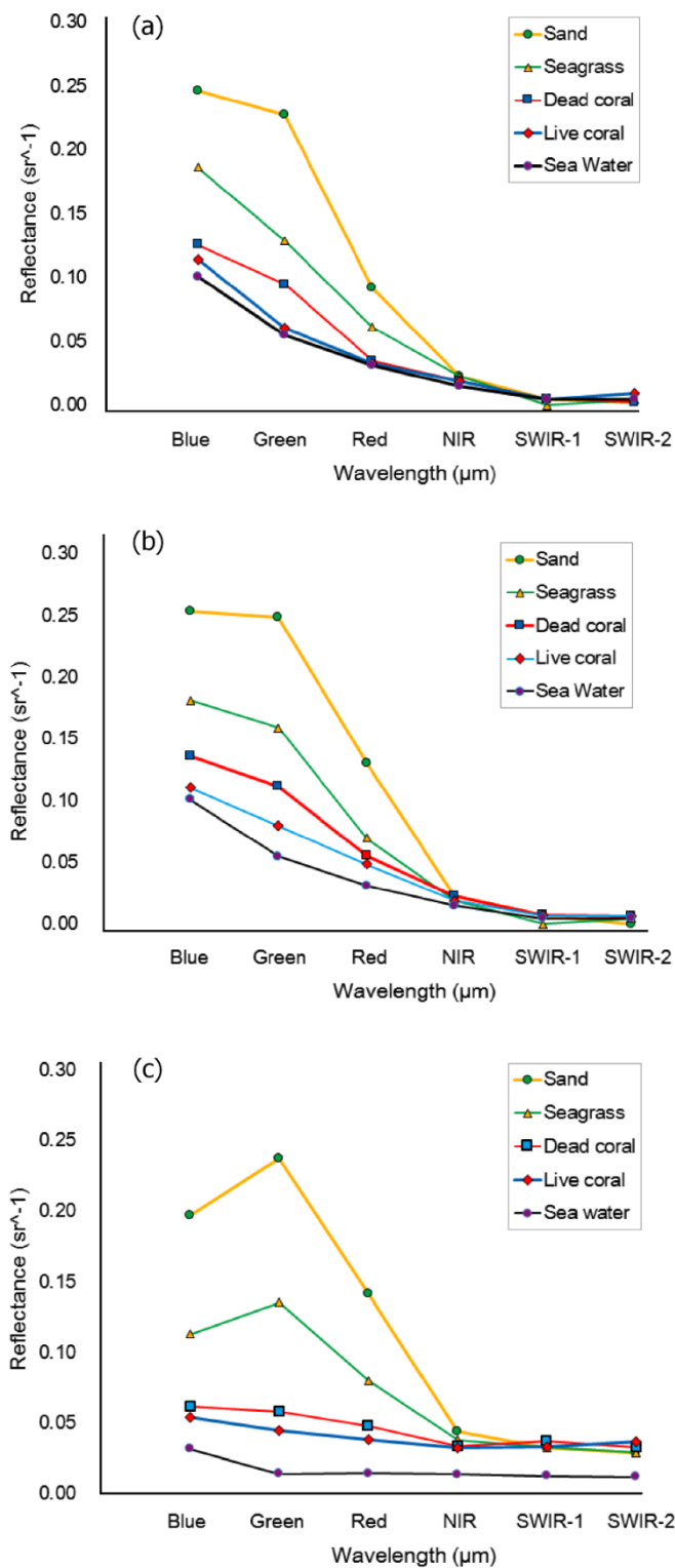
Fig.7 Spectral profile of object classes (sand, seagrasses, dead corals, live corals and sea water) on three series Landsat Imagery data: (a) Landsat TM 1994, (b) Landsat 7 ETM 2002, and (c) Landsat 8 OLI 2014
